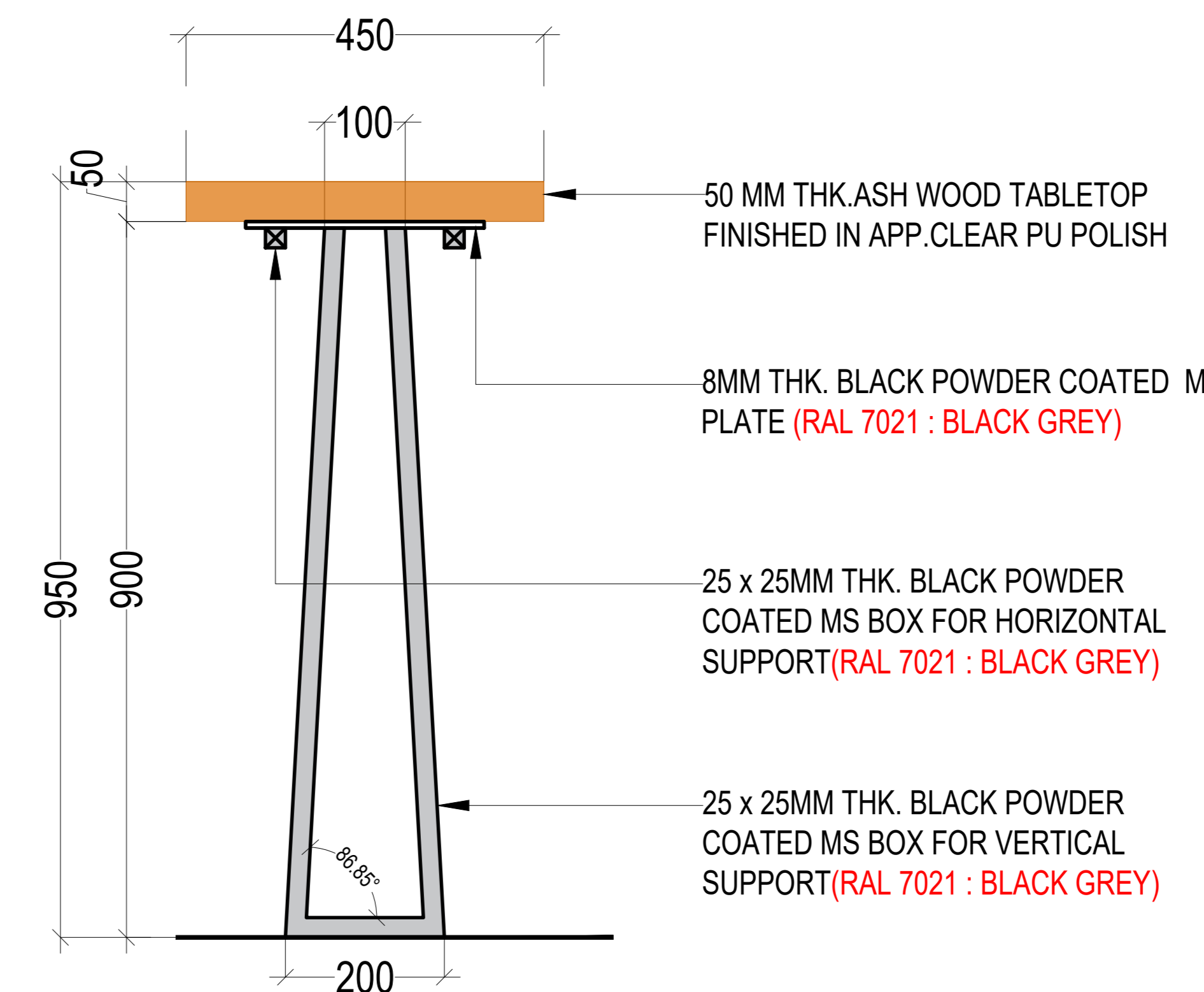
SIDE ELEVATION
