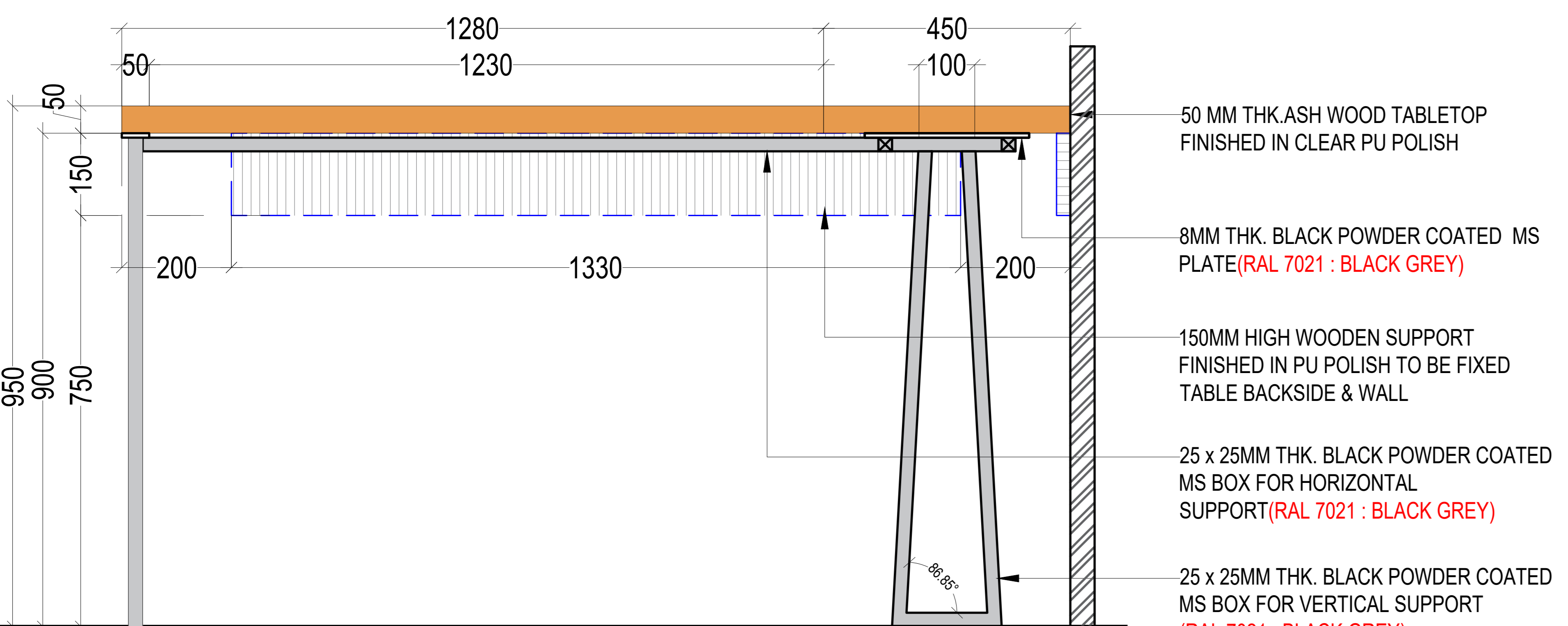
SECTIONAL ELEVATION BB'
