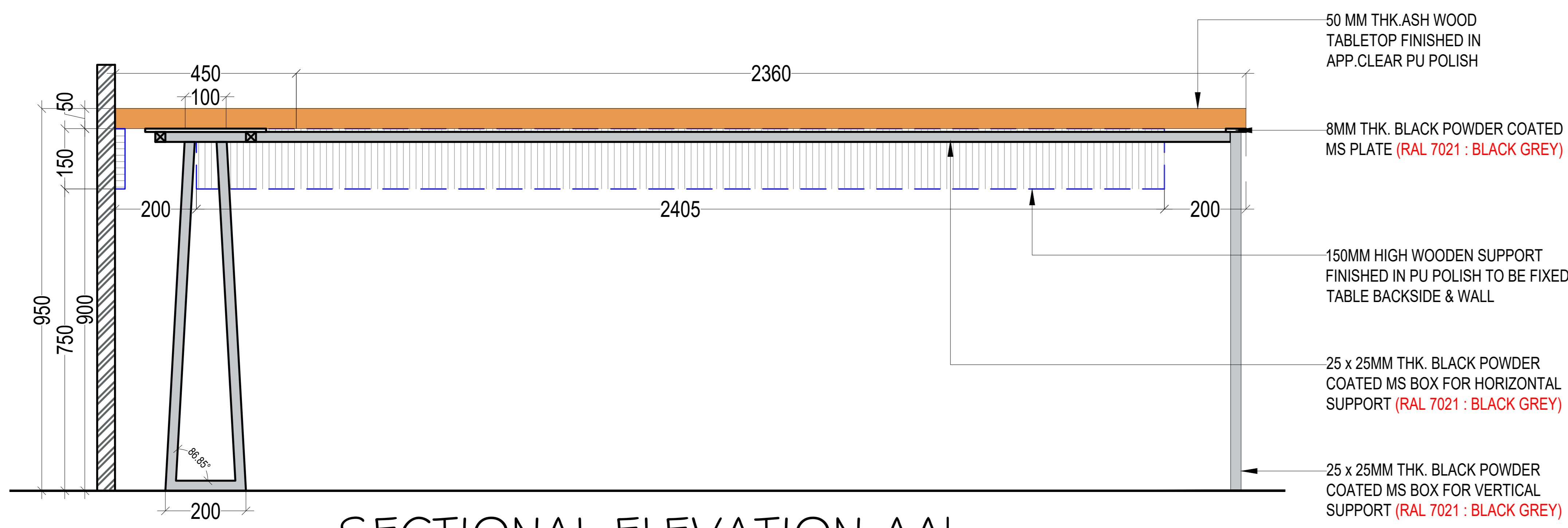
SECTIONAL ELEVATION AA'
