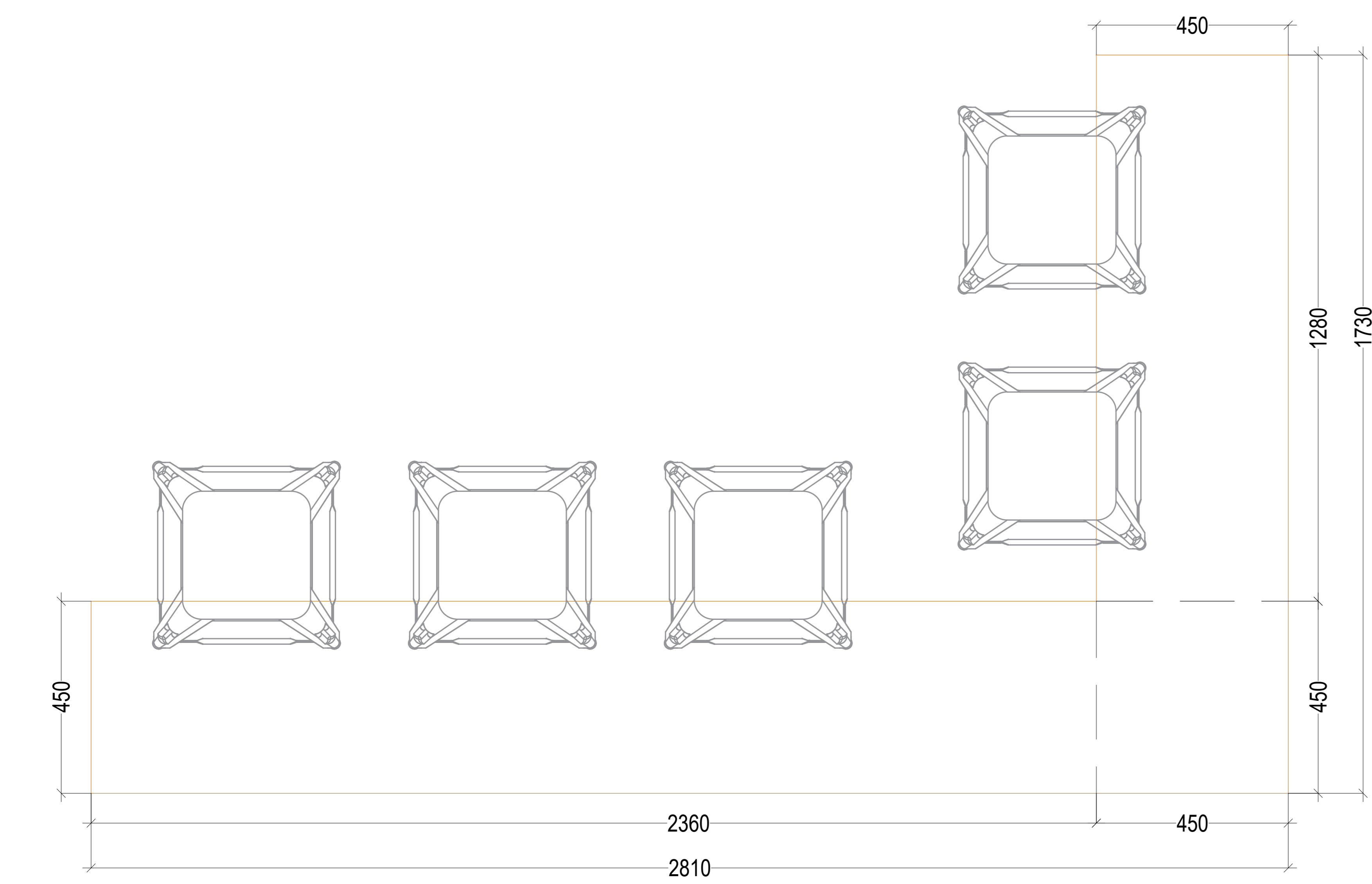
PLAN
