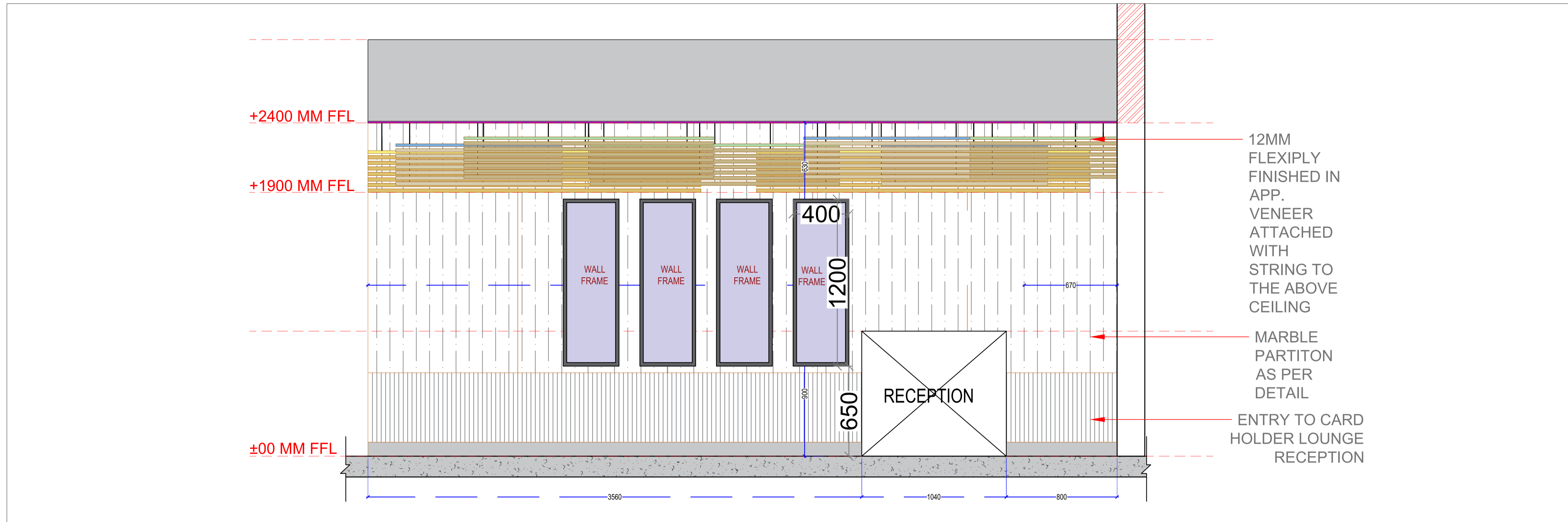
CARD HOLDER -RIGHT SIDE WALL ELEVATION
