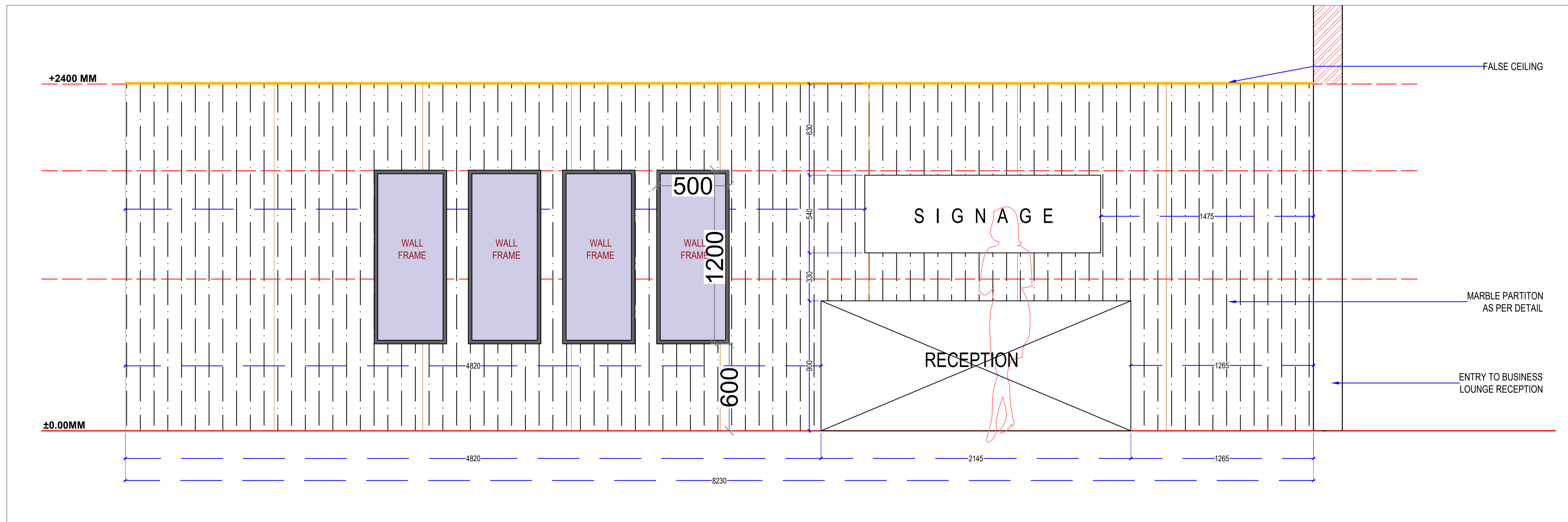
BUSINESS LOUNGE - RIGHT SIDE WALL ELEVATION
