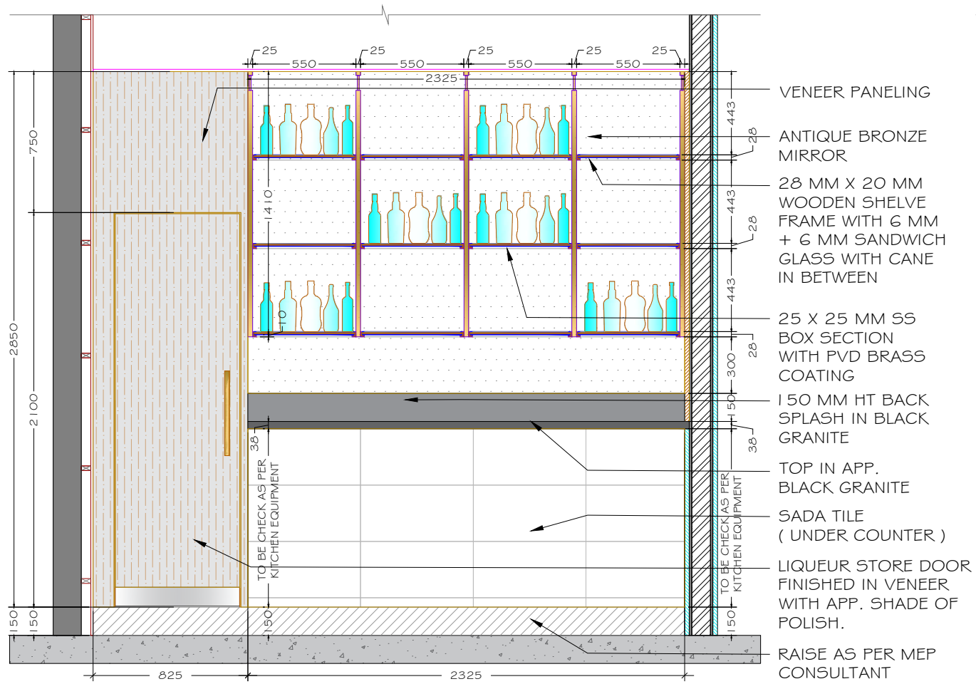
ELEVATION C-C' ( BAR BACK )
