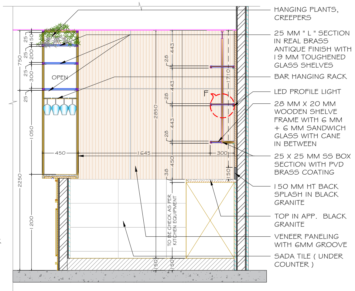
SECTION D-D'
