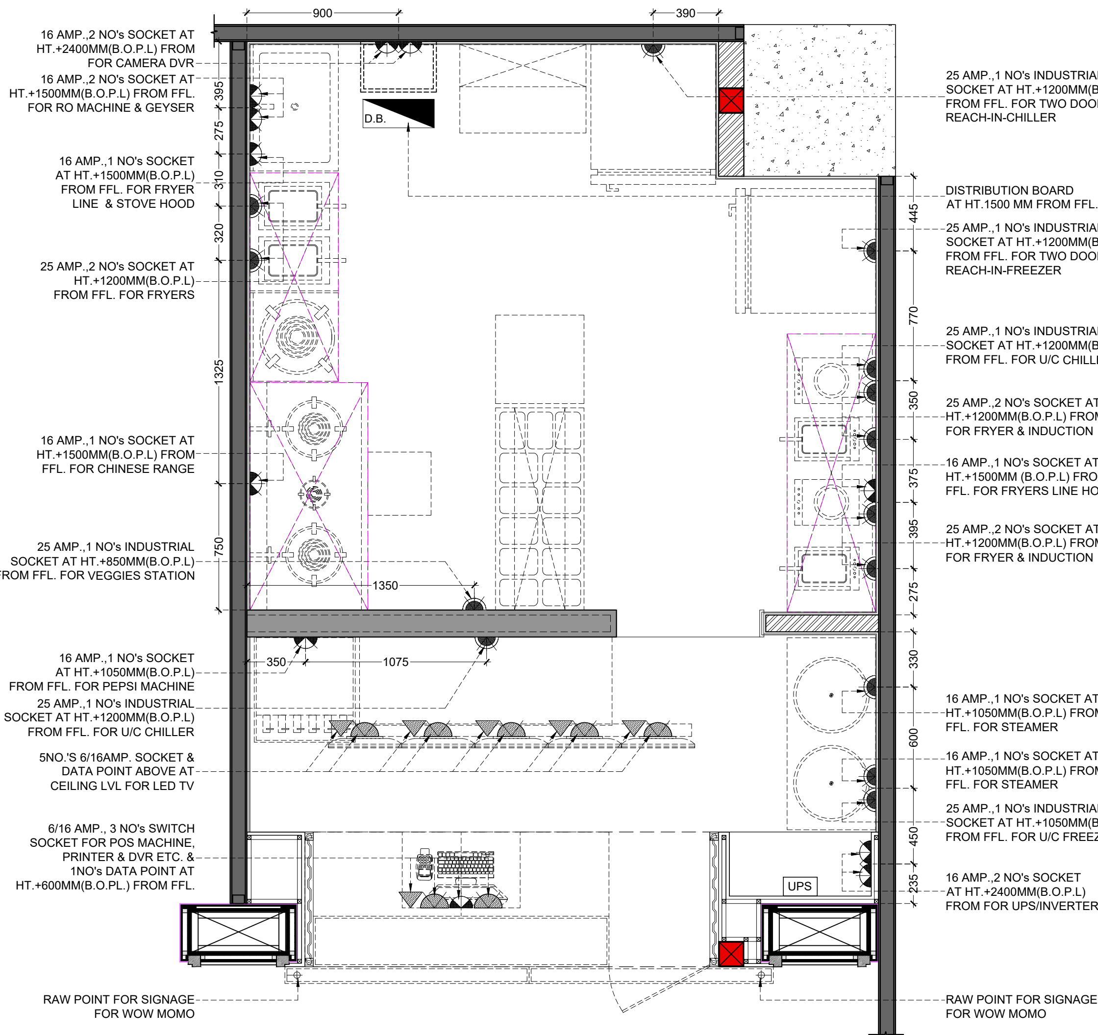
WALL ELECTRICAL LAYOUT
