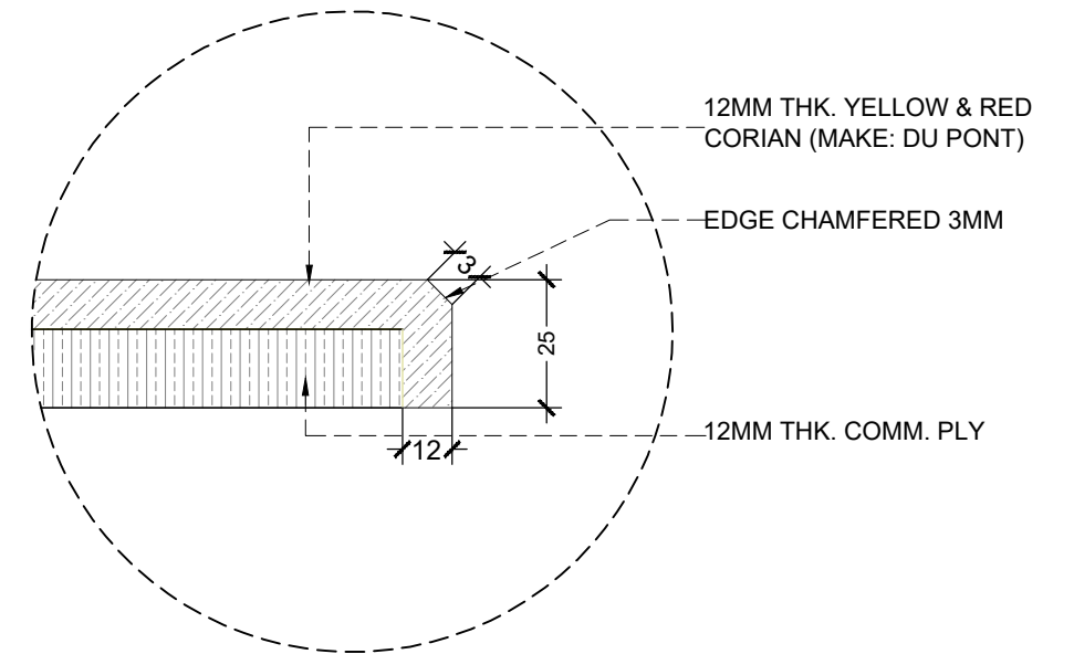
DETAIL-X1 TYPICAL CORIAN EDGE DETAIL
