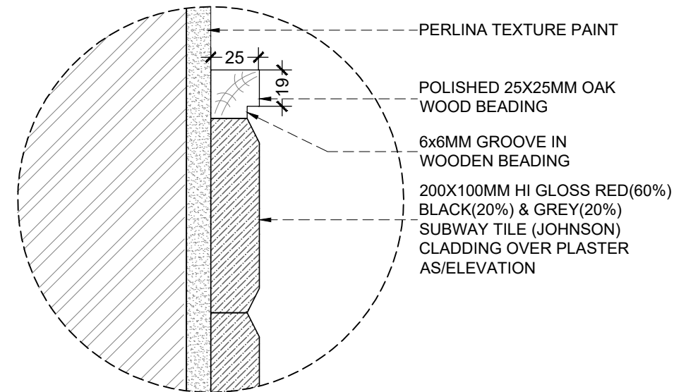
DETAIL-Y1 TYPICAL SECTIONAL DETAIL FOR BEADING
