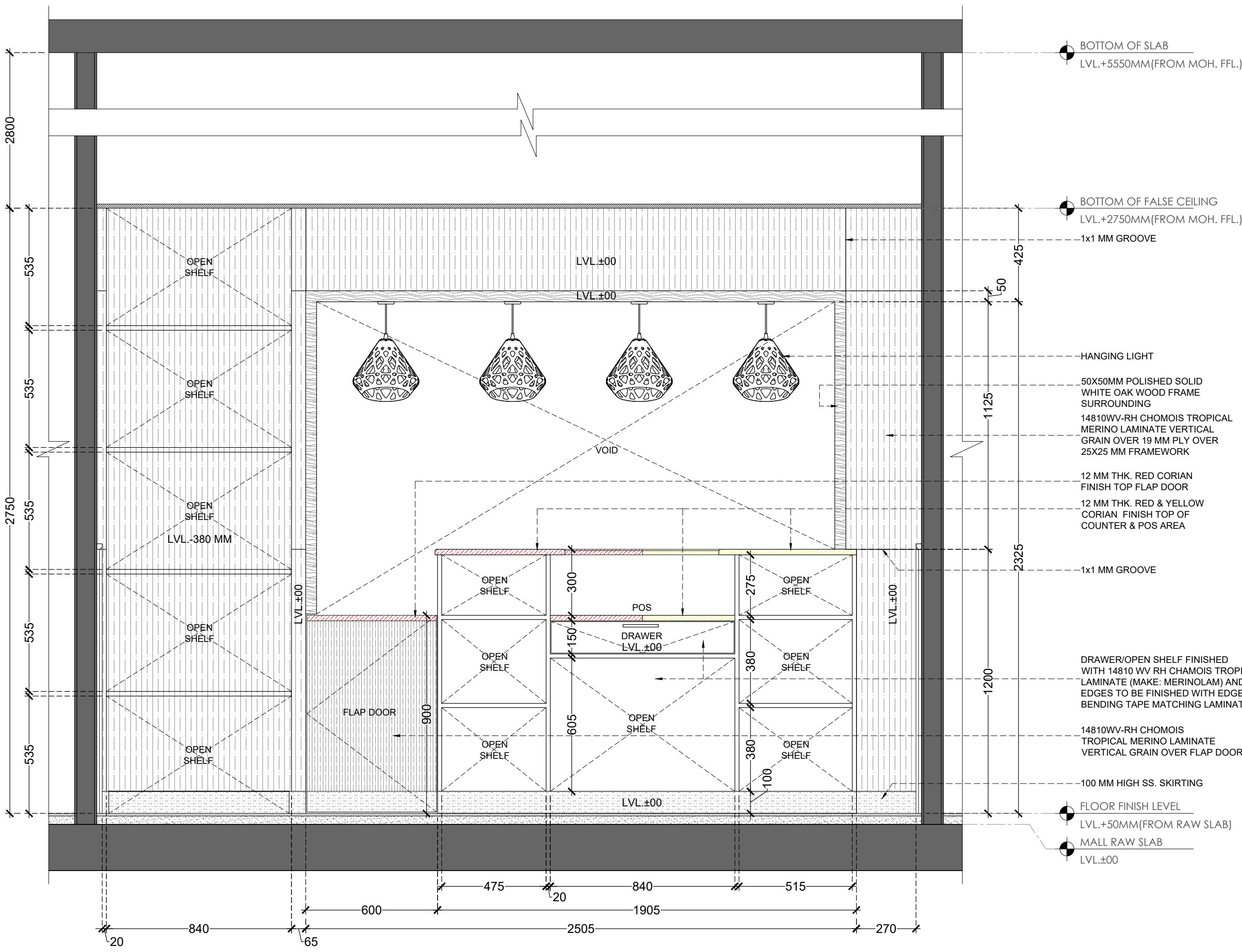
SECTIONAL ELEVATION-D
