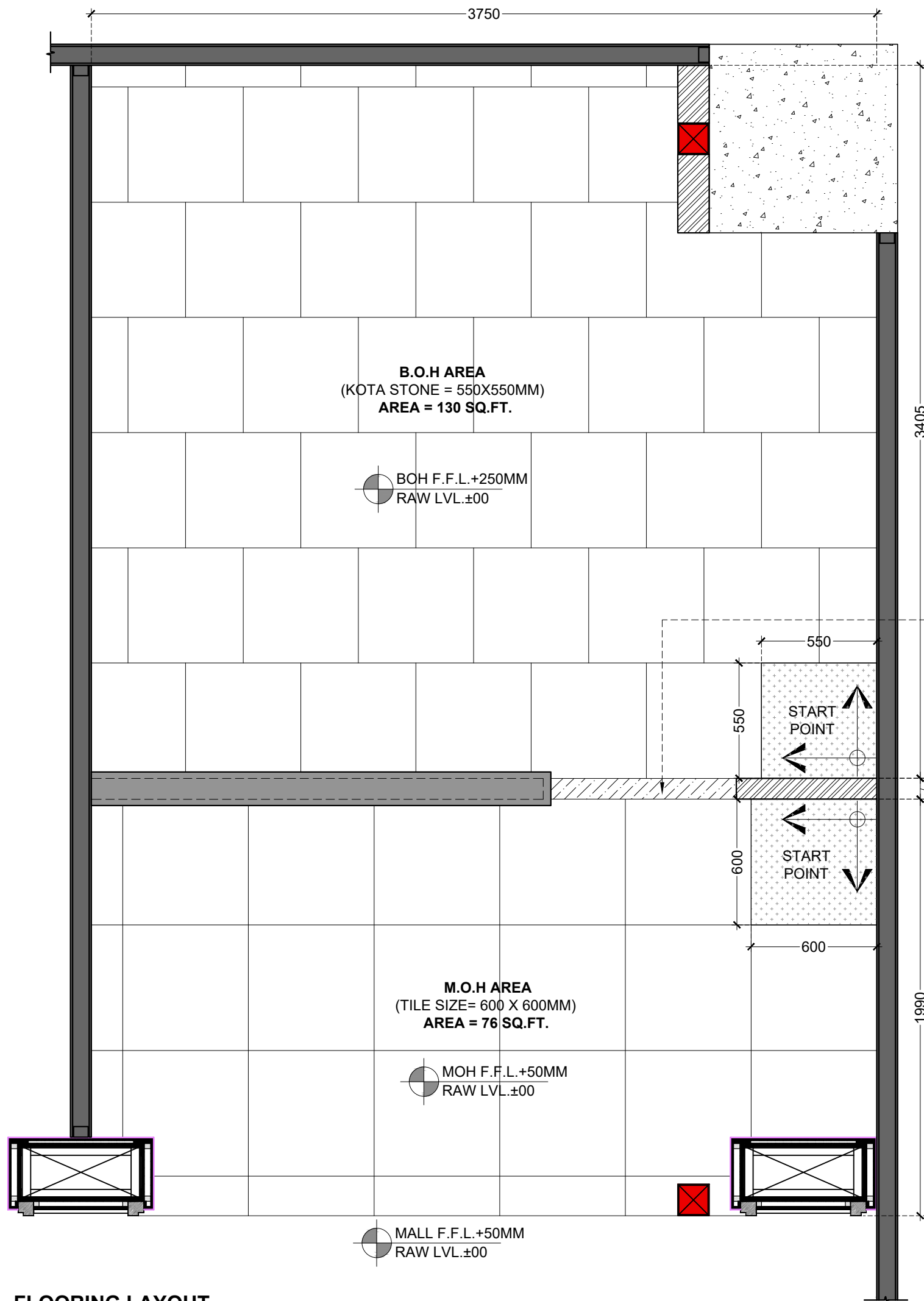
FLOORING LAYOUT
