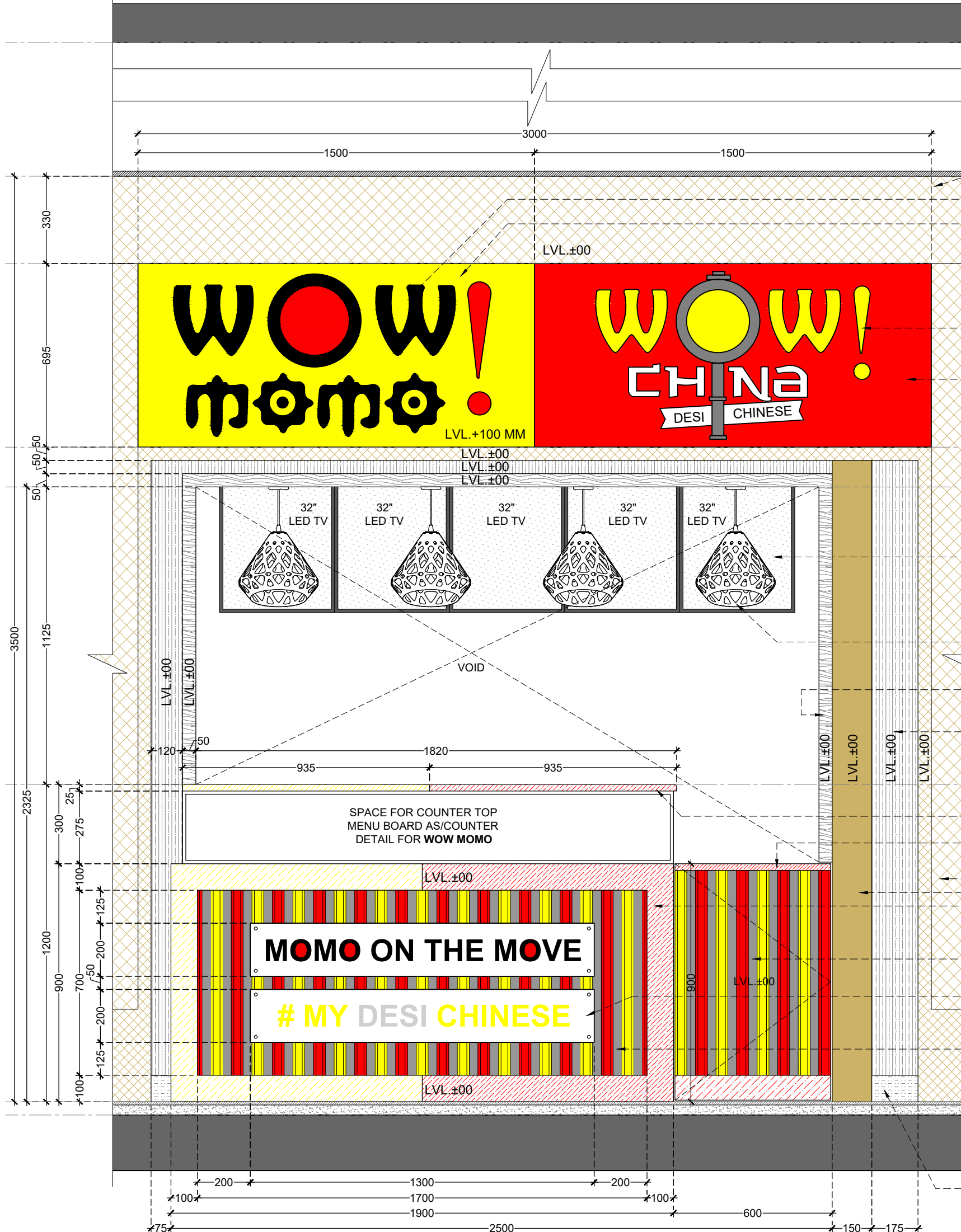
FRONT ELEVATION
