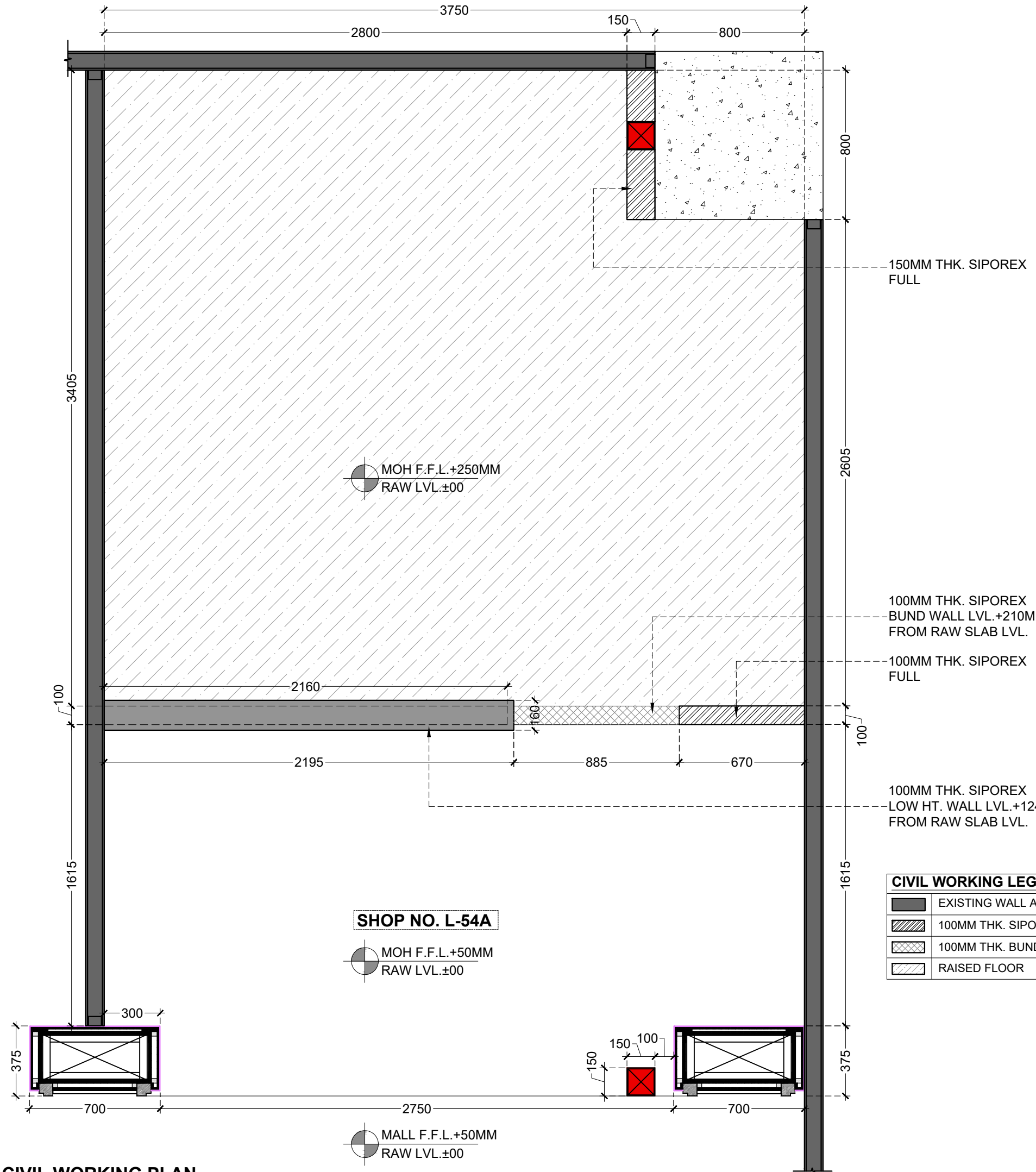
CIVIL WORKING PLAN
