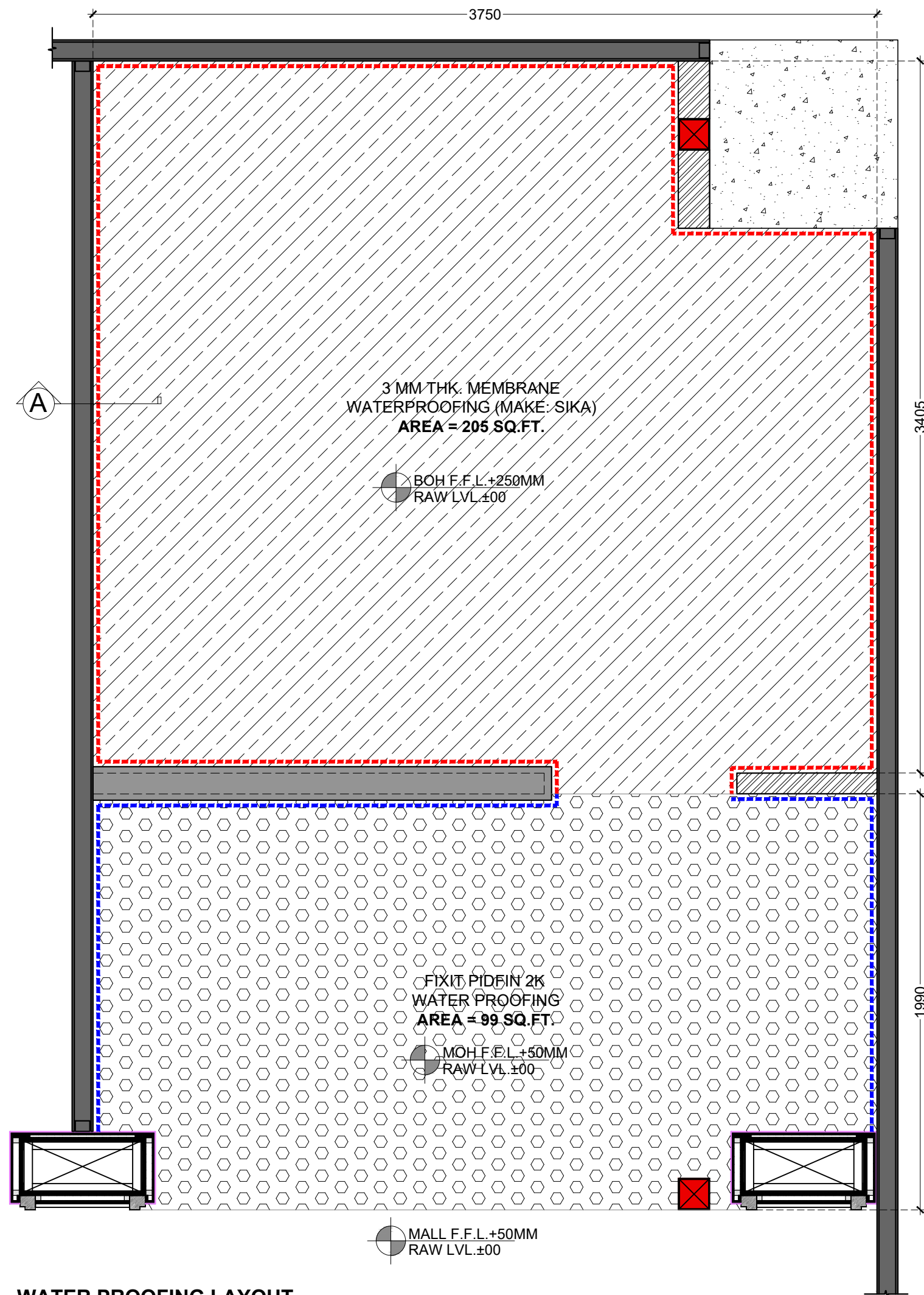
WATER PROOFING LAYOUT
