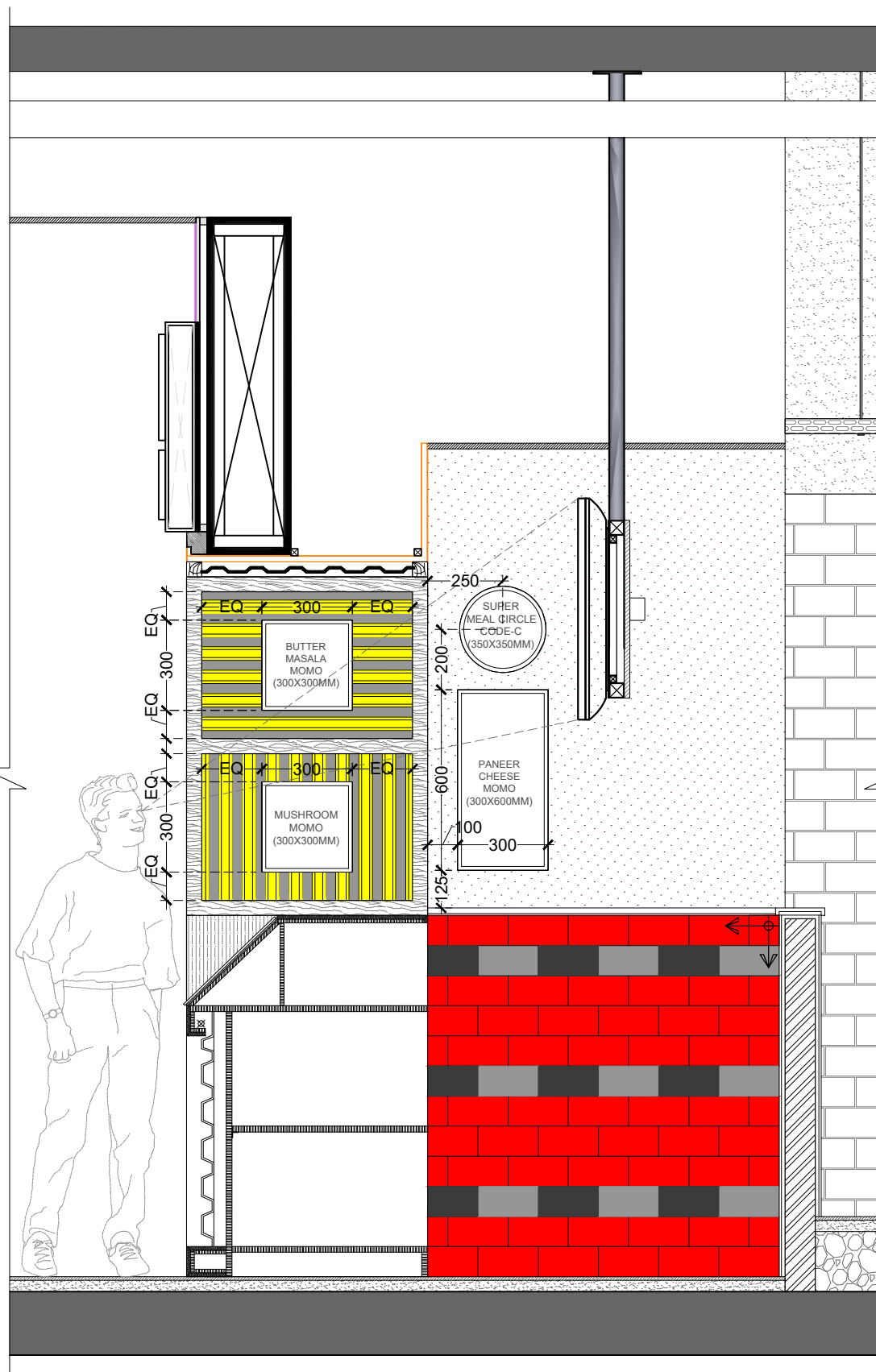
BRANDING ELEVATION-A
