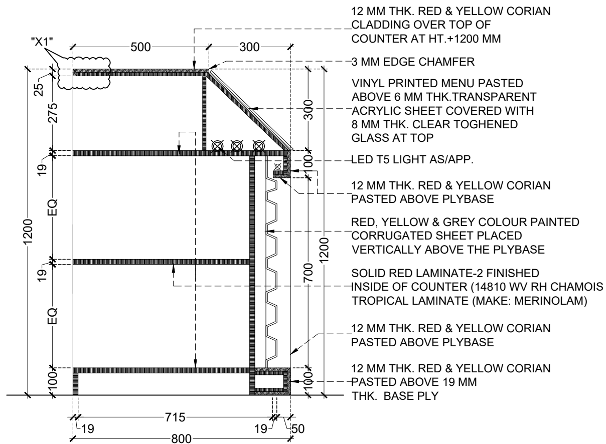
TYPICAL COUNTER SECTION
