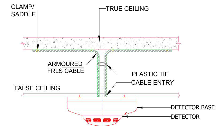
TYPICAL FIXING DETAIL OF DETECTOR AT BELOW FALSE CEILING AREA
