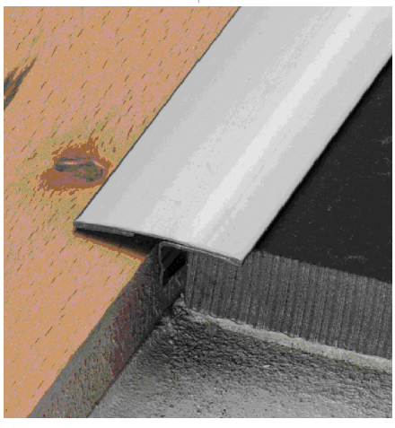
6MM S.S TRANSITION STRIP TO BE ADDED AT THE ENTRANCE TO SEPARATE THE AIRPORT'S FLOORING FROM THE SUBWAY FLOORING
