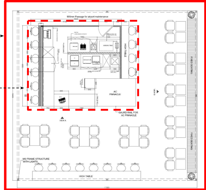
ABC BAR LAYOUT
