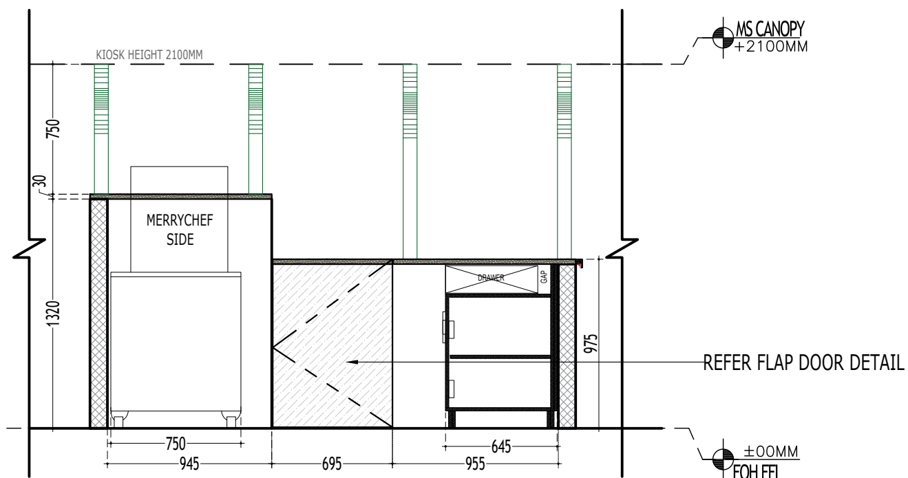
1 ELEVATION - BB' (WITH EQUIPMENTS) SCALE 1:30
