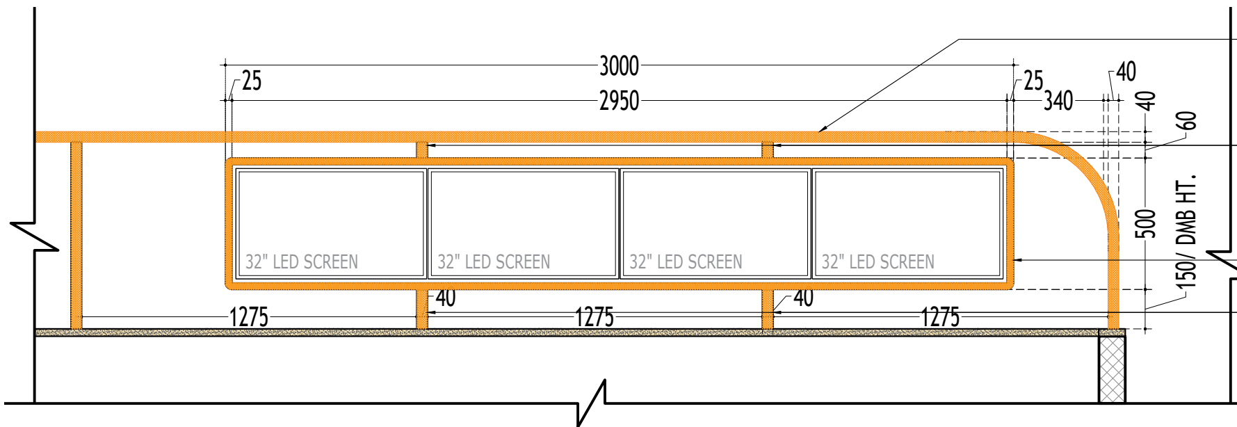
1 FRONT ELEVATION SCALE 1:20
