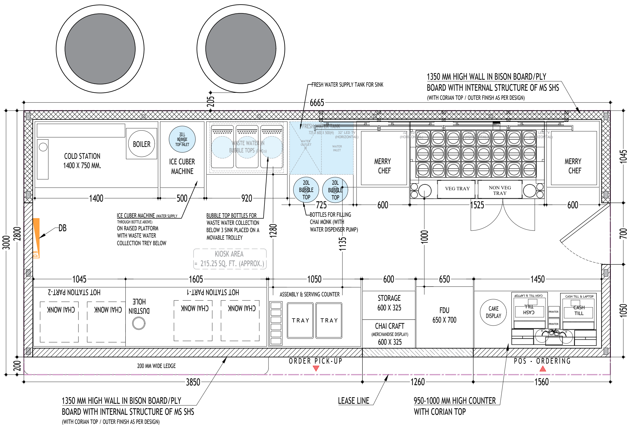
1 LAYOUT PLAN SCALE 1:25
