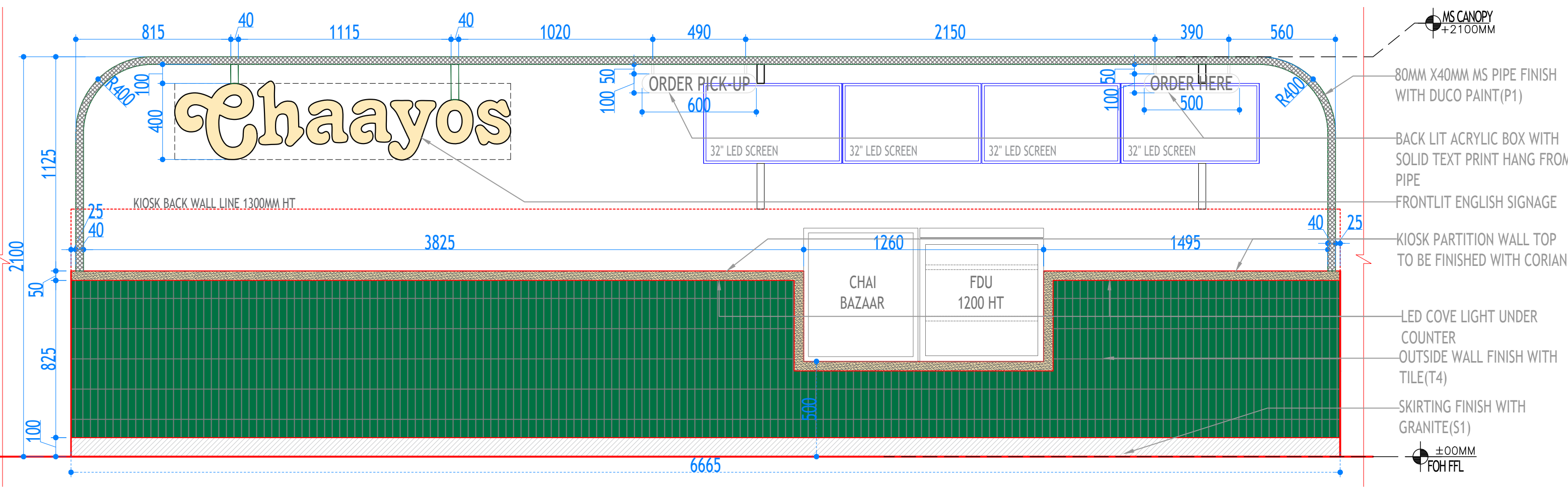
1 ELEVATION BB' SCALE 1:20
