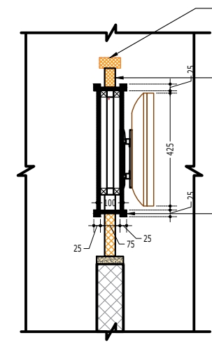
3 SIDE SECTION SCALE 1:20
