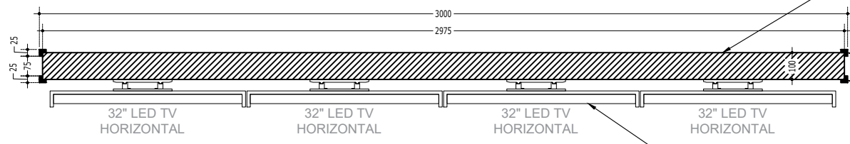
2 PLAN (VIEW FROM TOP) SCALE 1:20
