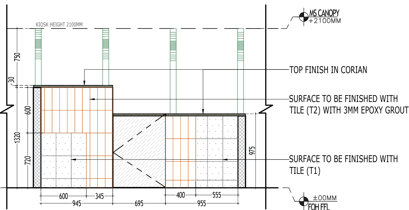
2 ELEVATION - BB' (WITHOUT EQUIPMENTS) SCALE 1:30
