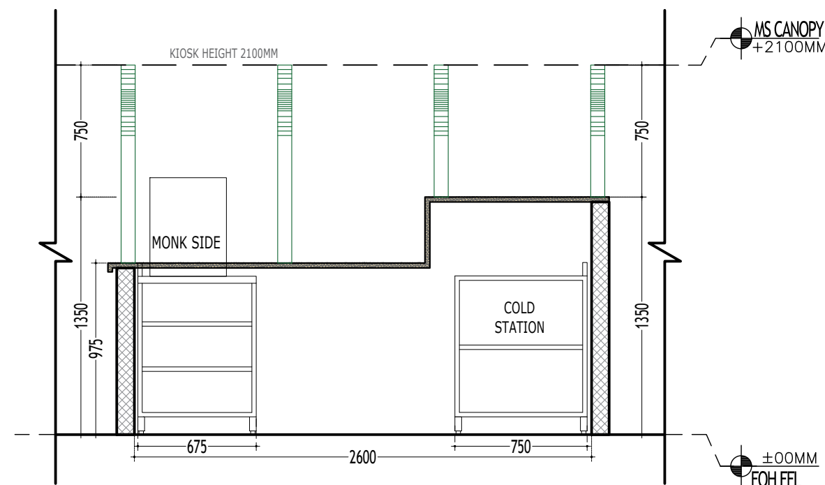
3 ELEVATION - DD' (WITH EQUIPMENTS) SCALE 1:30
