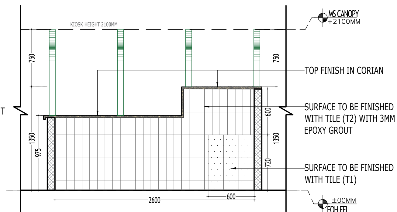
4 ELEVATION - DD' (WITHOUT EQUIPMENTS) SCALE 1:30
