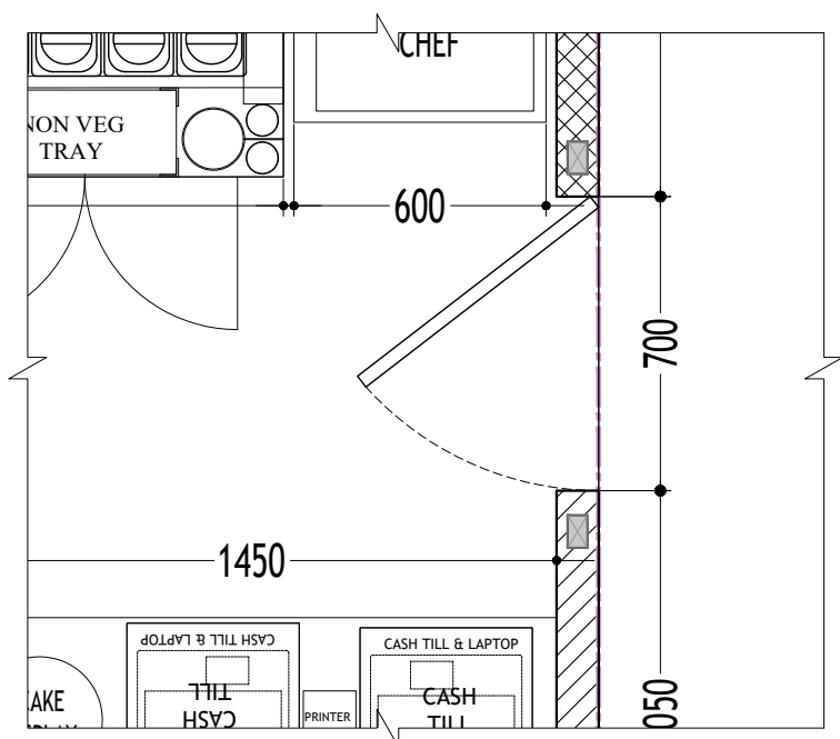
1 FLAP DOOR - D1 PLAN SCALE 1:20
