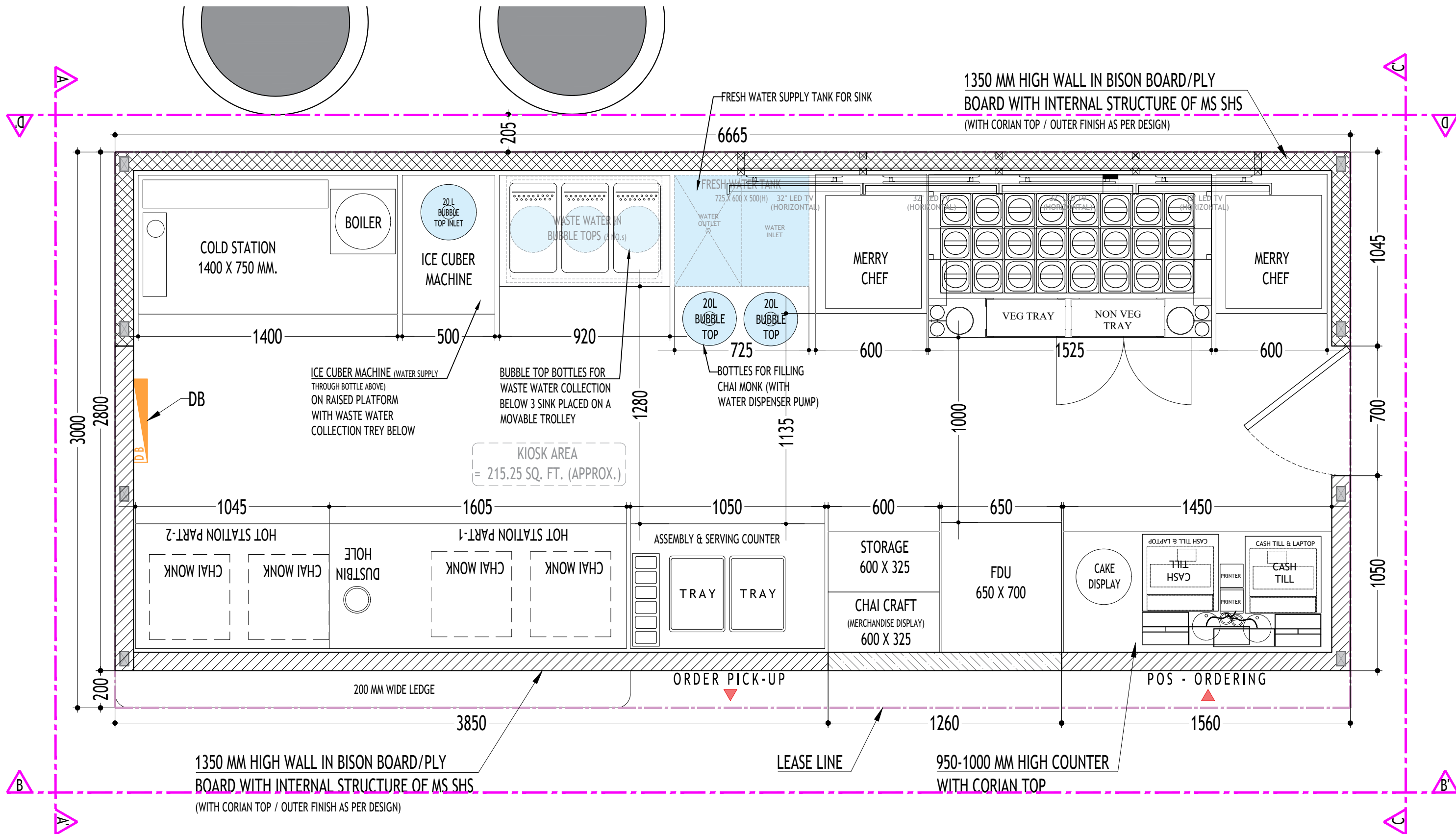
1 LAYOUT PLAN SCALE 1:20
