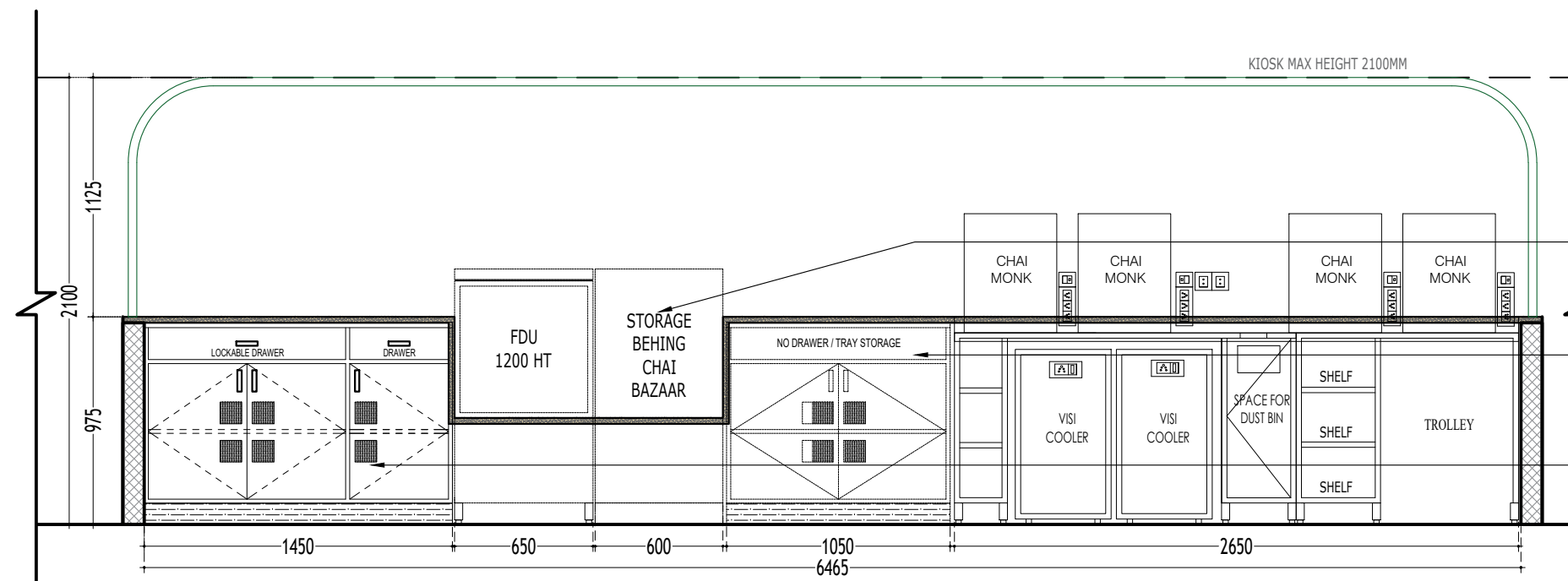
1 ELEVATION - DD' (WITH EQUIPMENTS) SCALE 1:30
