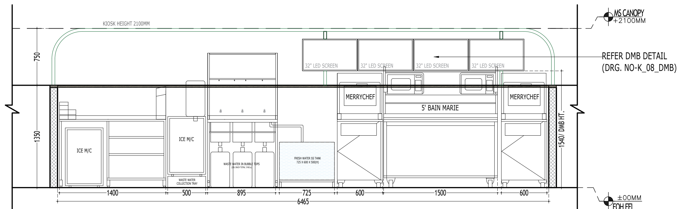
1 ELEVATION - AA' (WITH EQUIPMENTS) SCALE 1:30
