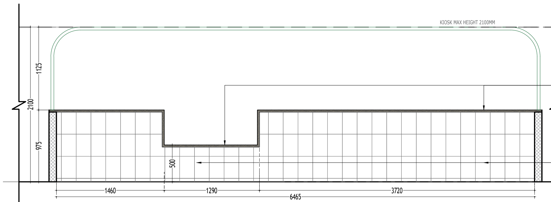
2 ELEVATION - DD' (WITHOUT EQUIPMENTS) SCALE 1:30
