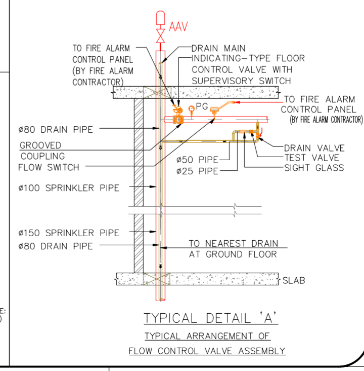
TYPICAL DETAIL 'A' TYPICAL ARRANGEMENT OF FLOW CONTROL VALVE ASSEMBLY
