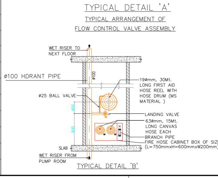
TYPICAL DETAIL 'A' TYPICAL ARRANGEMENT OF FLOW CONTROL VALVE ASSEMBLY
