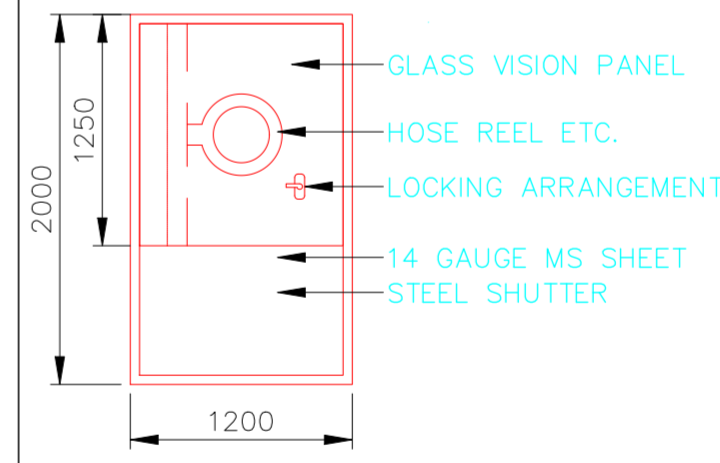
TYPICAL INTERNAL HYDRANT ENCLOSURE DETAILS
