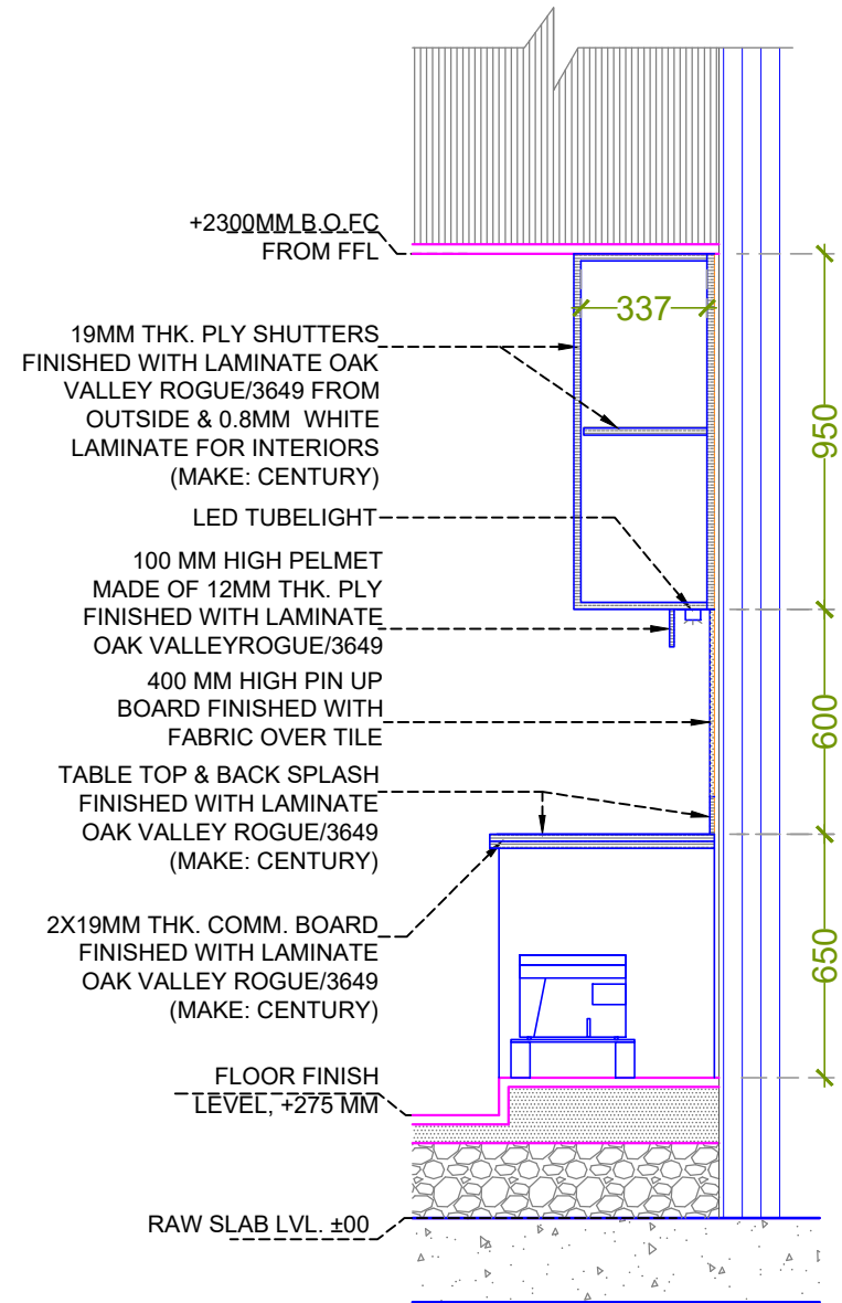
SECTIONAL ELEVATION-B
