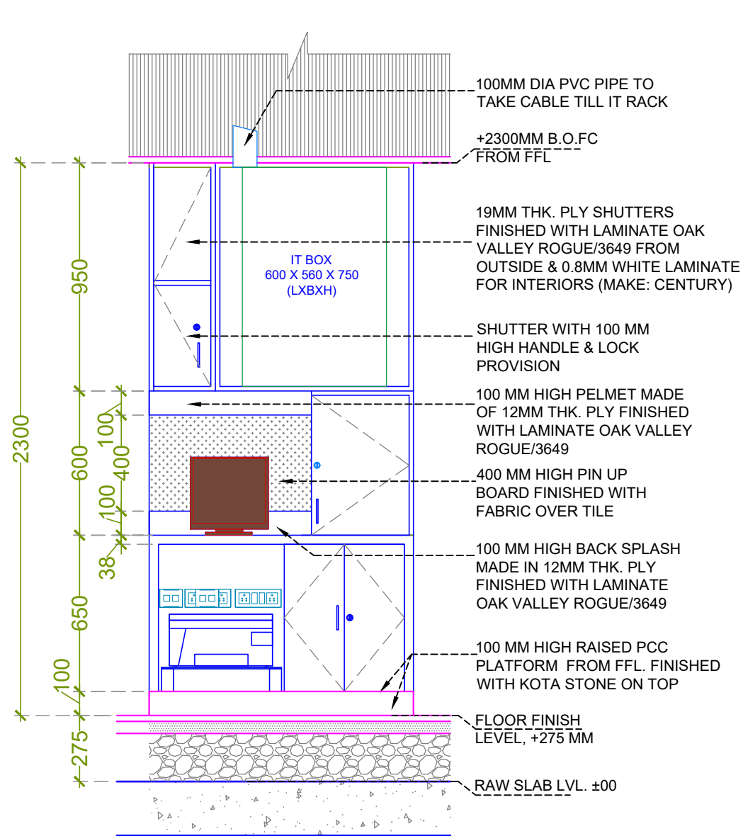
FRONT ELEVATION
