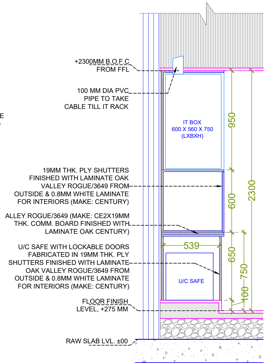
SECTIONAL ELEVATION-A
