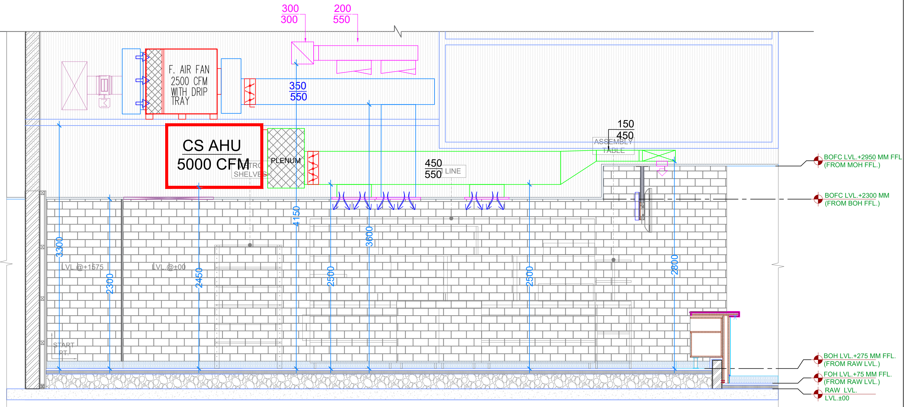
SECTIONAL ELEVATION-A
