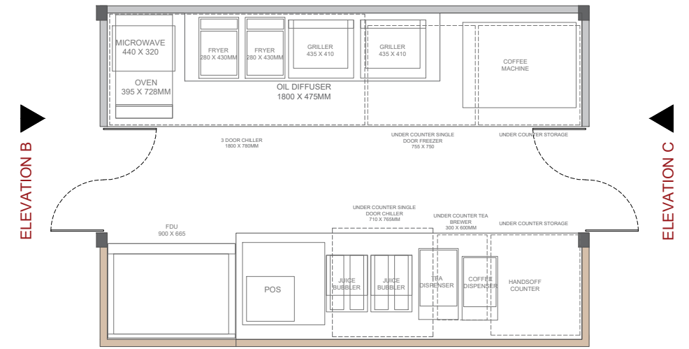
ELEVATION A LAYOUT
