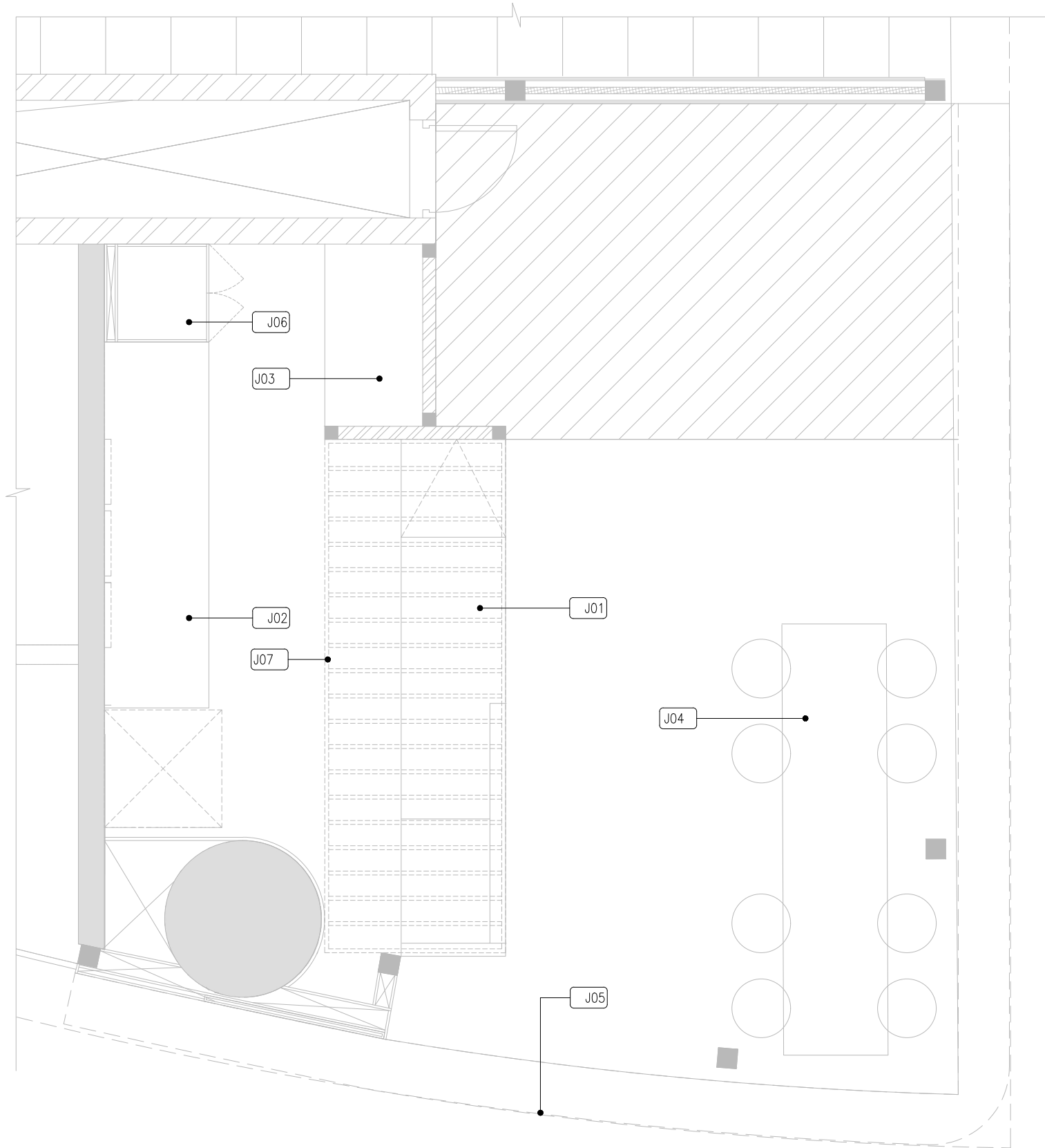
01 DETAIL DRAWING LEGEND 02GA-005 1:40
