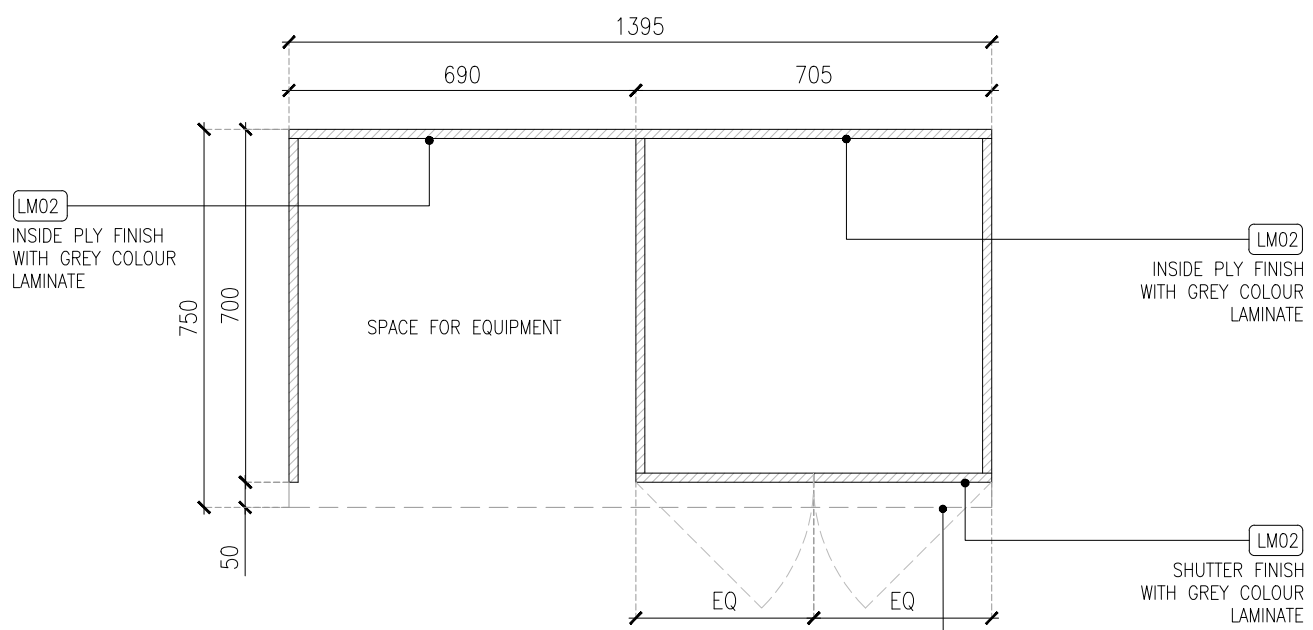
FRAMING PLAN @500MM LVL (SCALE 1:15)
