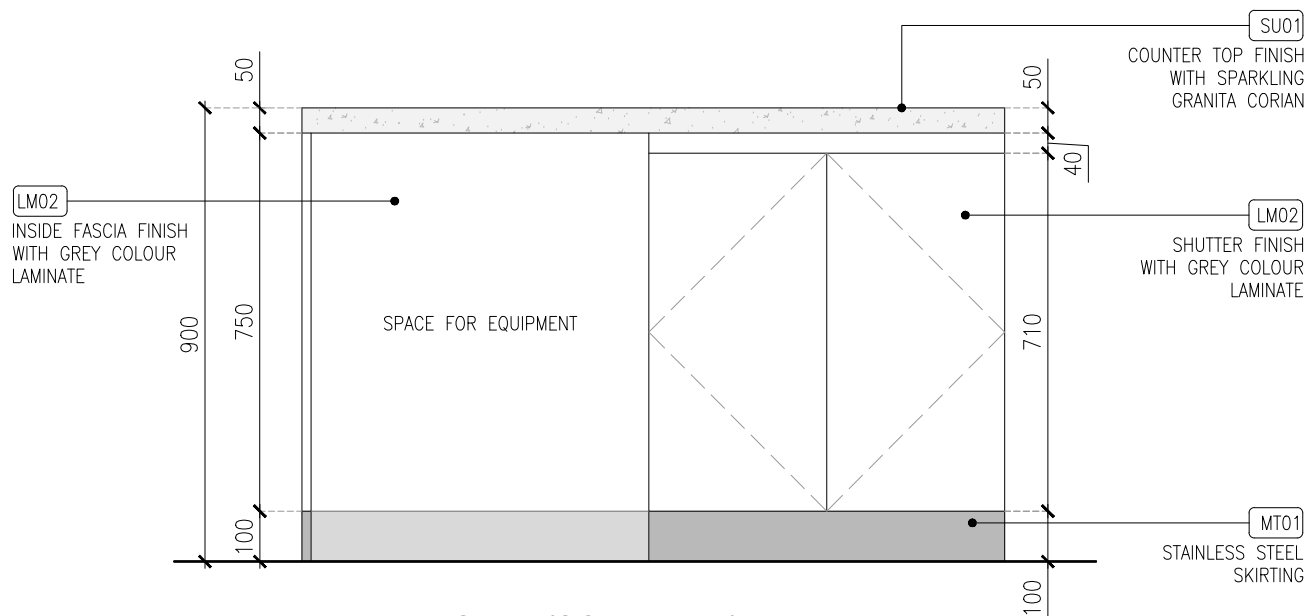
ELEVATION-01 (SCALE 1:15)
