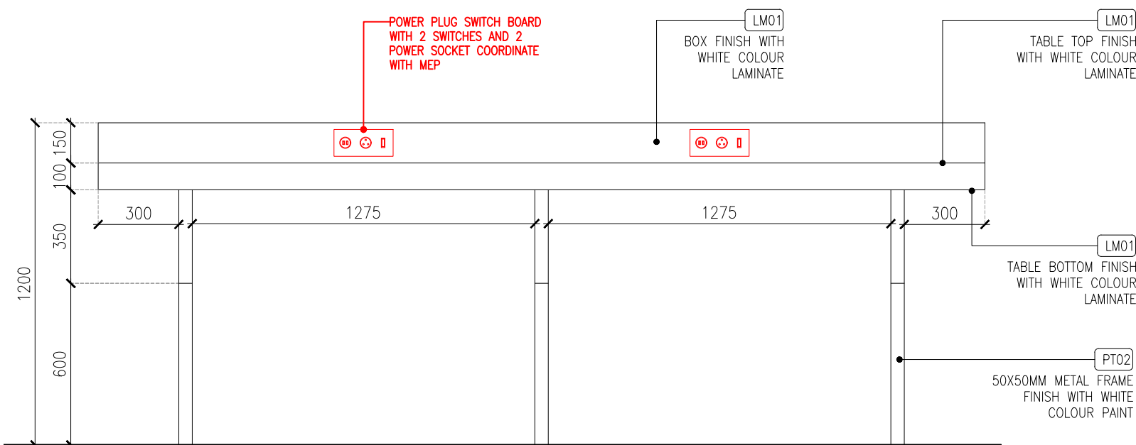
ELEVATION-01 (SCALE-1:20)
