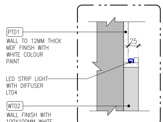
DETAIL-A (SCALE 1:10)
