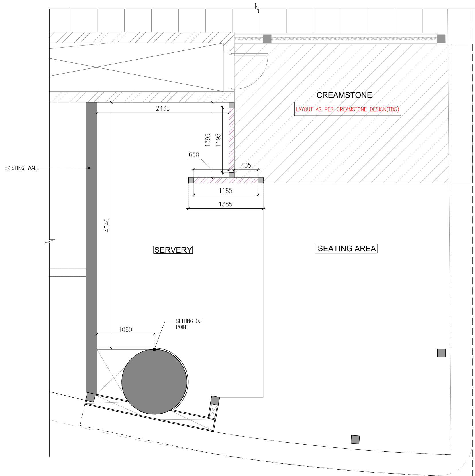
01 WALL DETAIL LAYOUT 02GA-102 1:40
