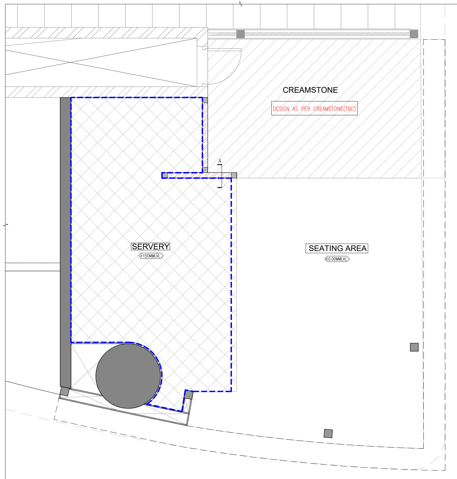
01 WATER PROOFING LAYOUT 02GA-107 1:40
