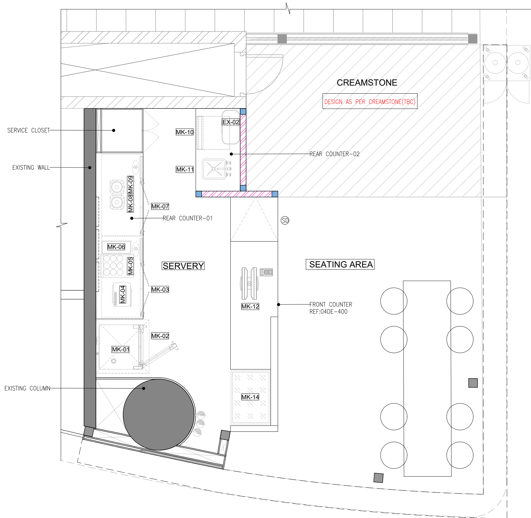
01 EQUIPMENT LAYOUT 02GA-101 1:40
