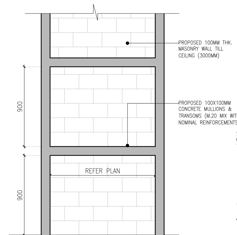
TYPICAL STRUCTURAL ELEVATION (WALL CONSTRUCTION) SCALE 1:25
