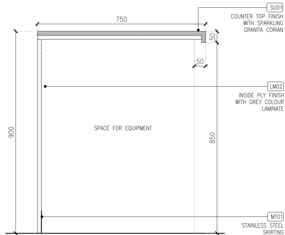
SECTION-01 (SCALE 1:10)
