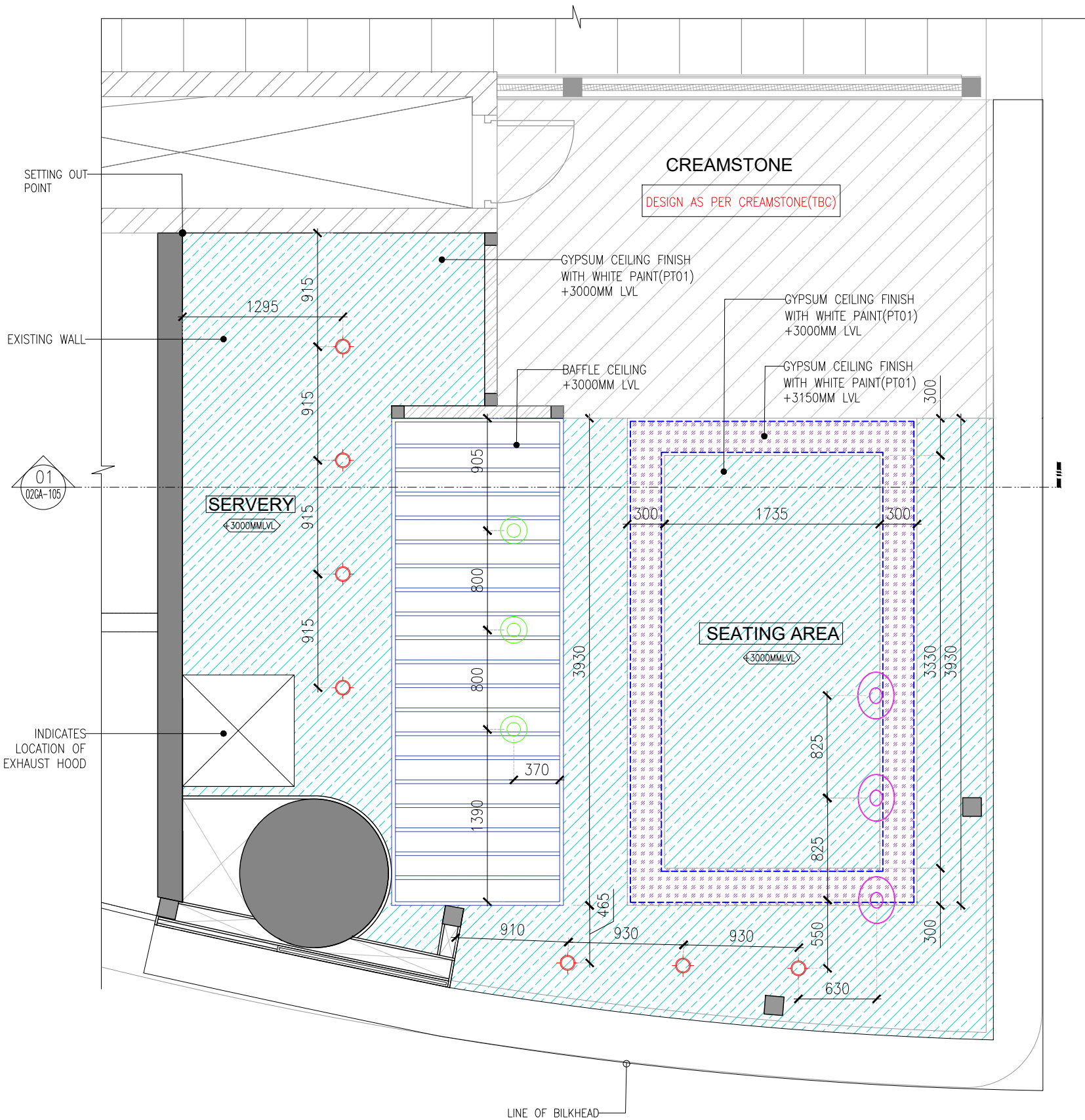
01 RCP + LIGHTING LAYOUT :PART-A 02GA-104/ 1:40
