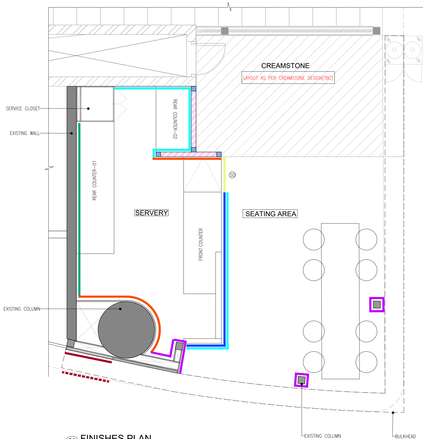
01 FINISHES PLAN 02GA-108 1:40
