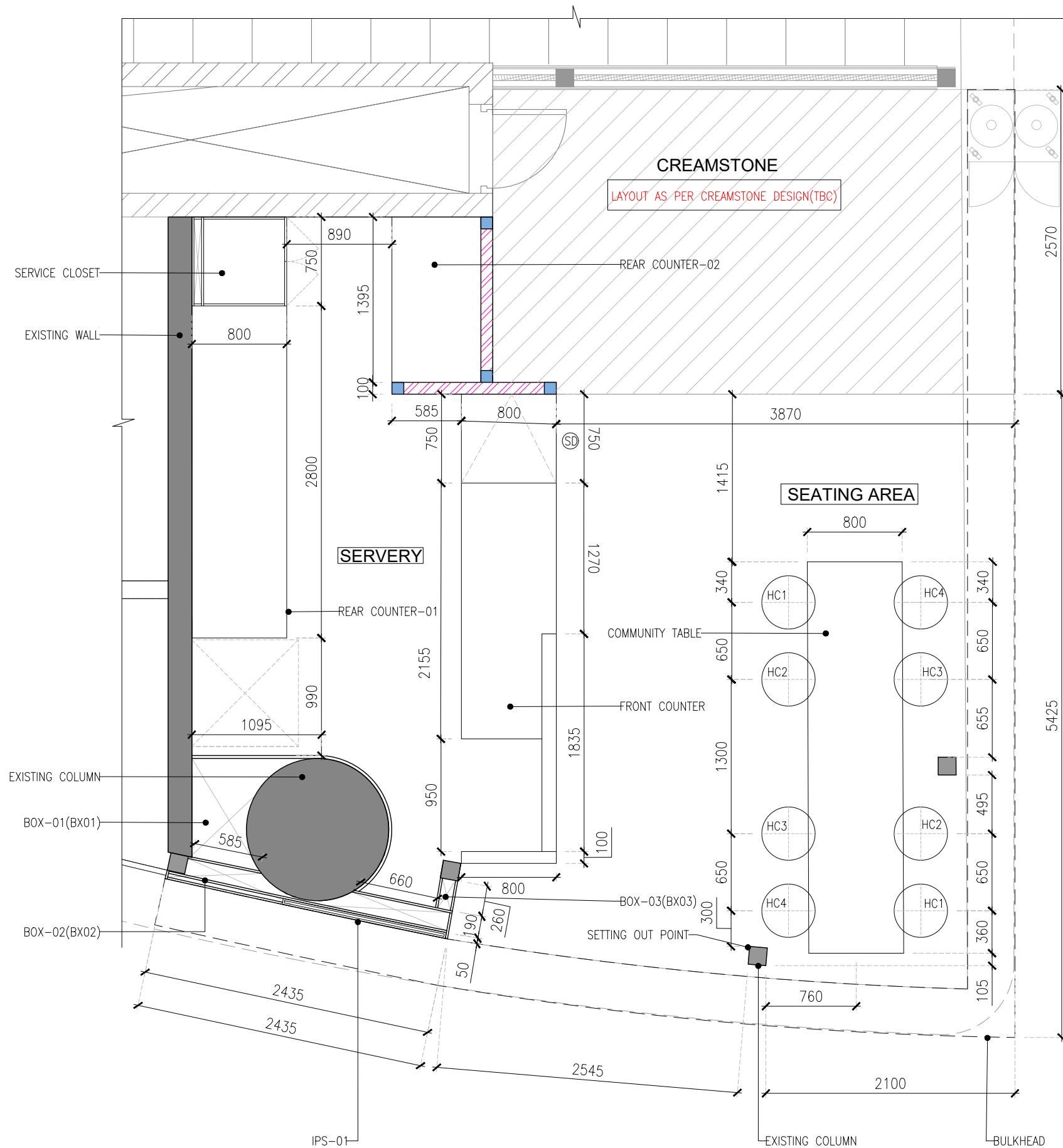
01 SETTING OUT PLAN 02GA-103 1:40
