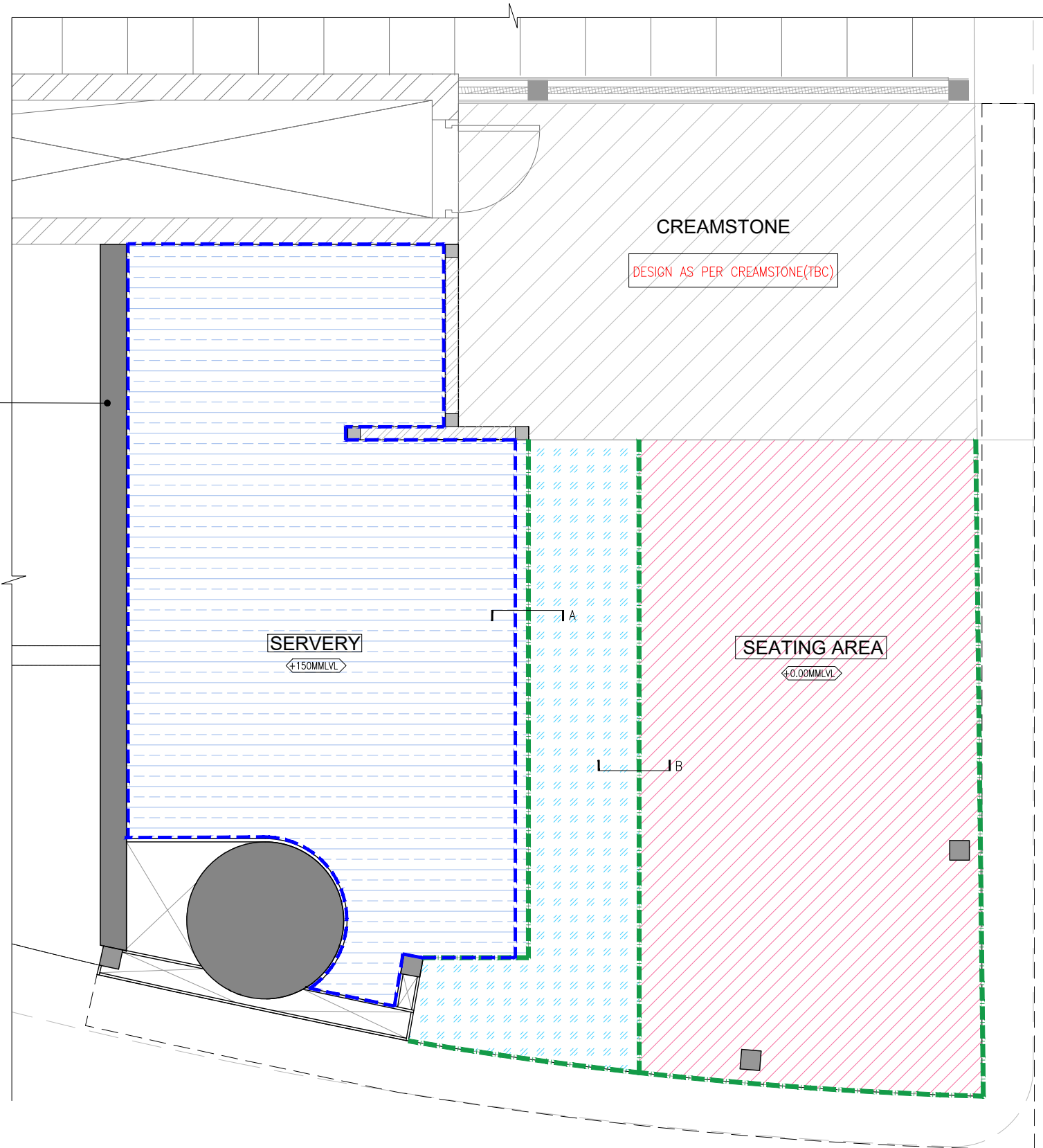
01 FLOORING LAYOUT 02GA-106 1:40
