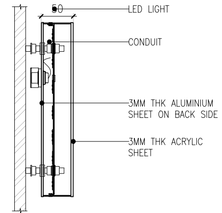
TYPICAL SECTION OF FRONT LIT SIGNAGE
