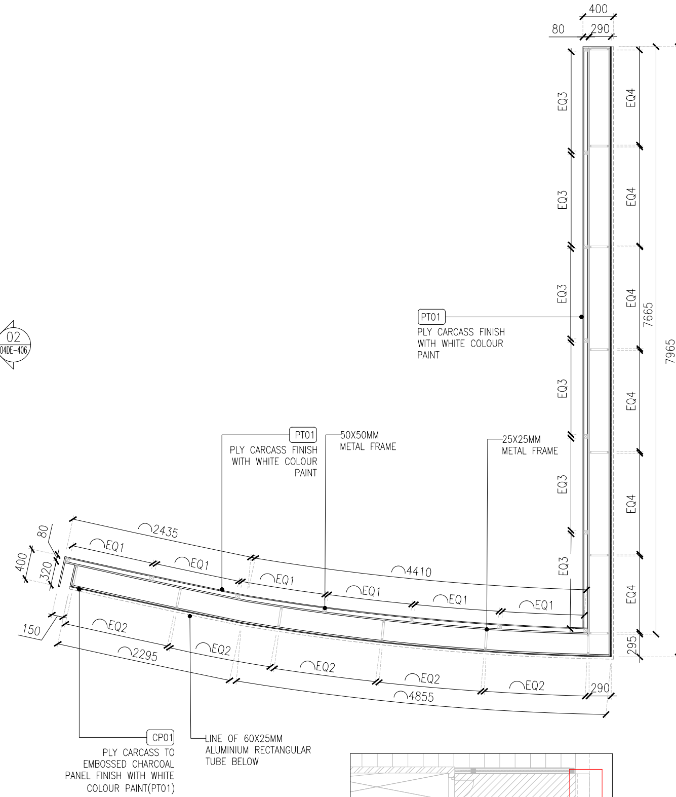
FRAMING PLAN @ 500MM LVL
