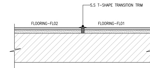
TYPICAL FLOOR TRANSITION DETAIL SECTION-B
