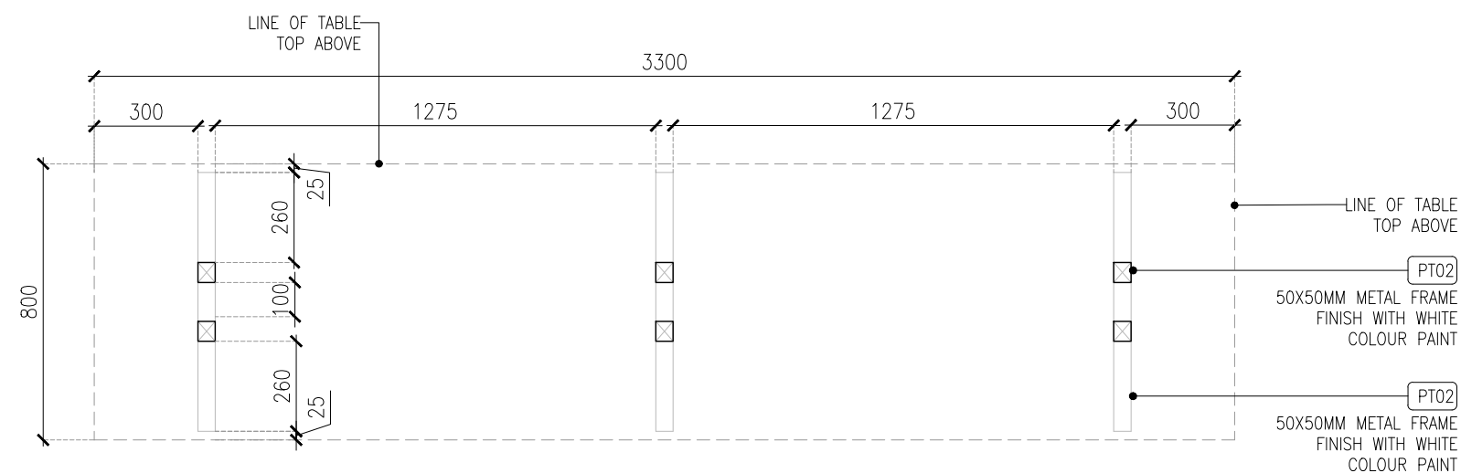
FRAMING PLAN @750MM LVL (SCALE-1:20)
