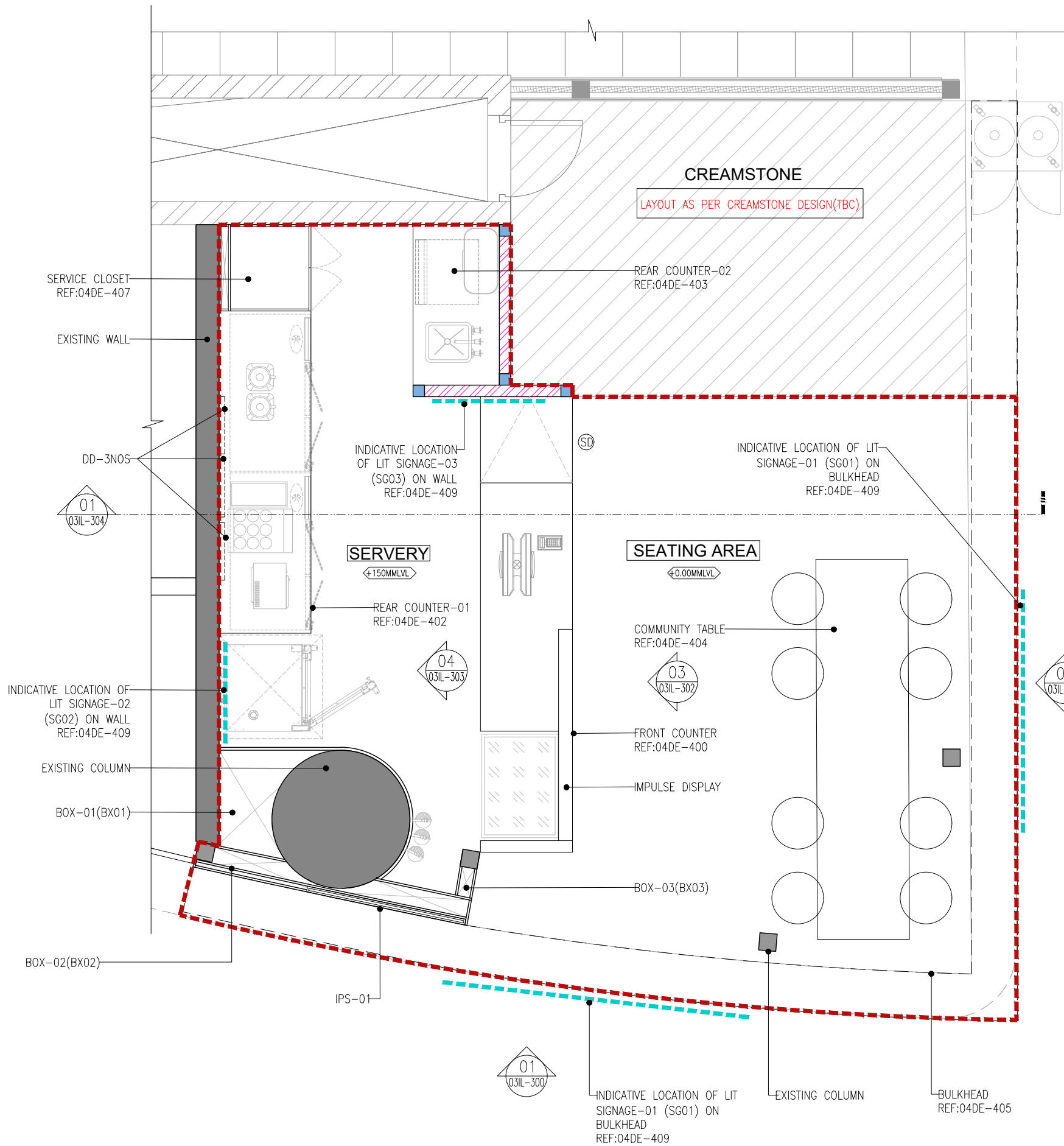
01 GENERAL ARRANGEMENT PLAN 02GA-100 1:40
