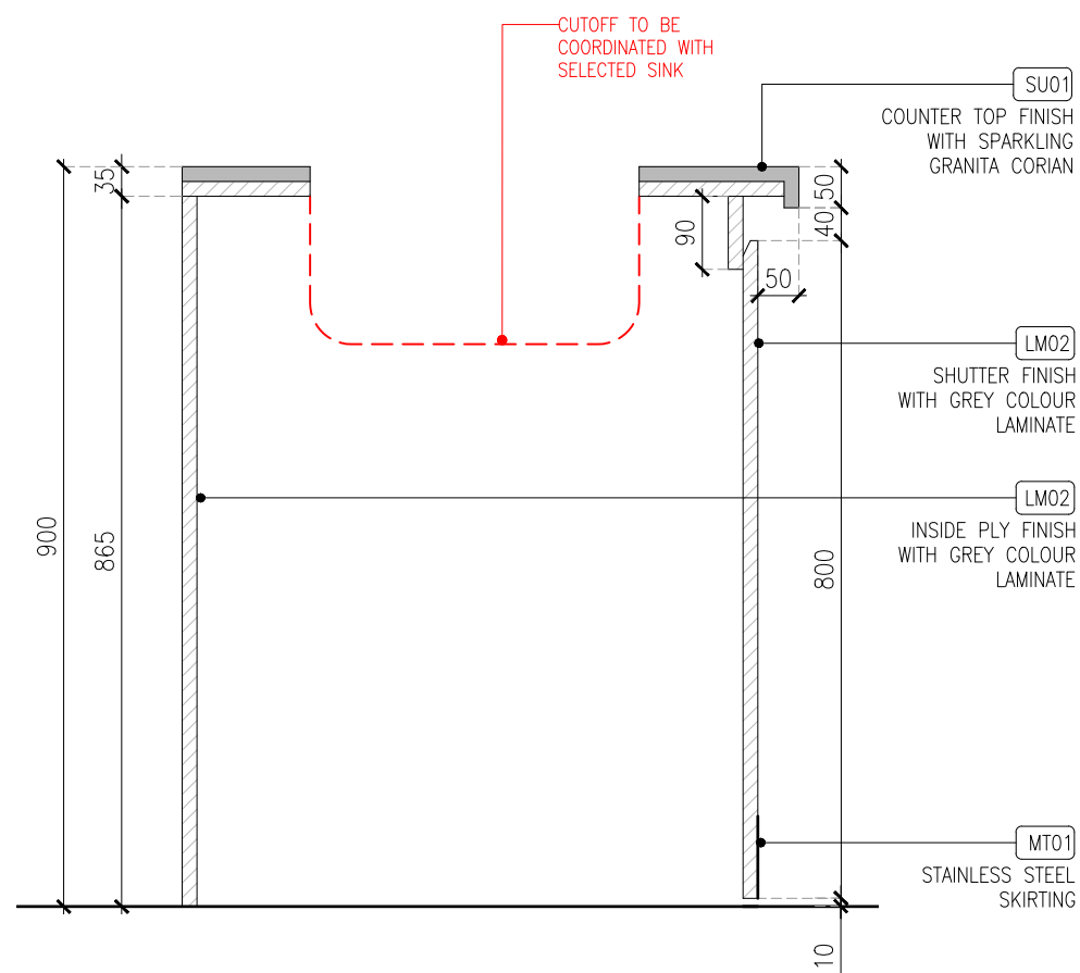
SECTION-01 (SCALE 1:10)
