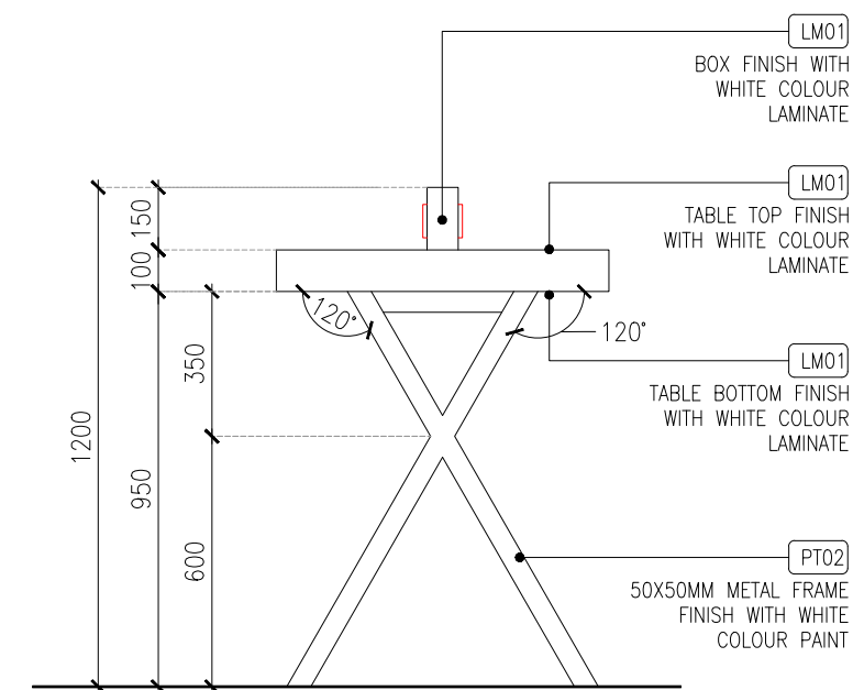
ELEVATION-02 (SCALE-1:20)
