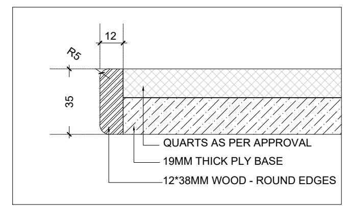
FURNITURE CORNER DETAIL
