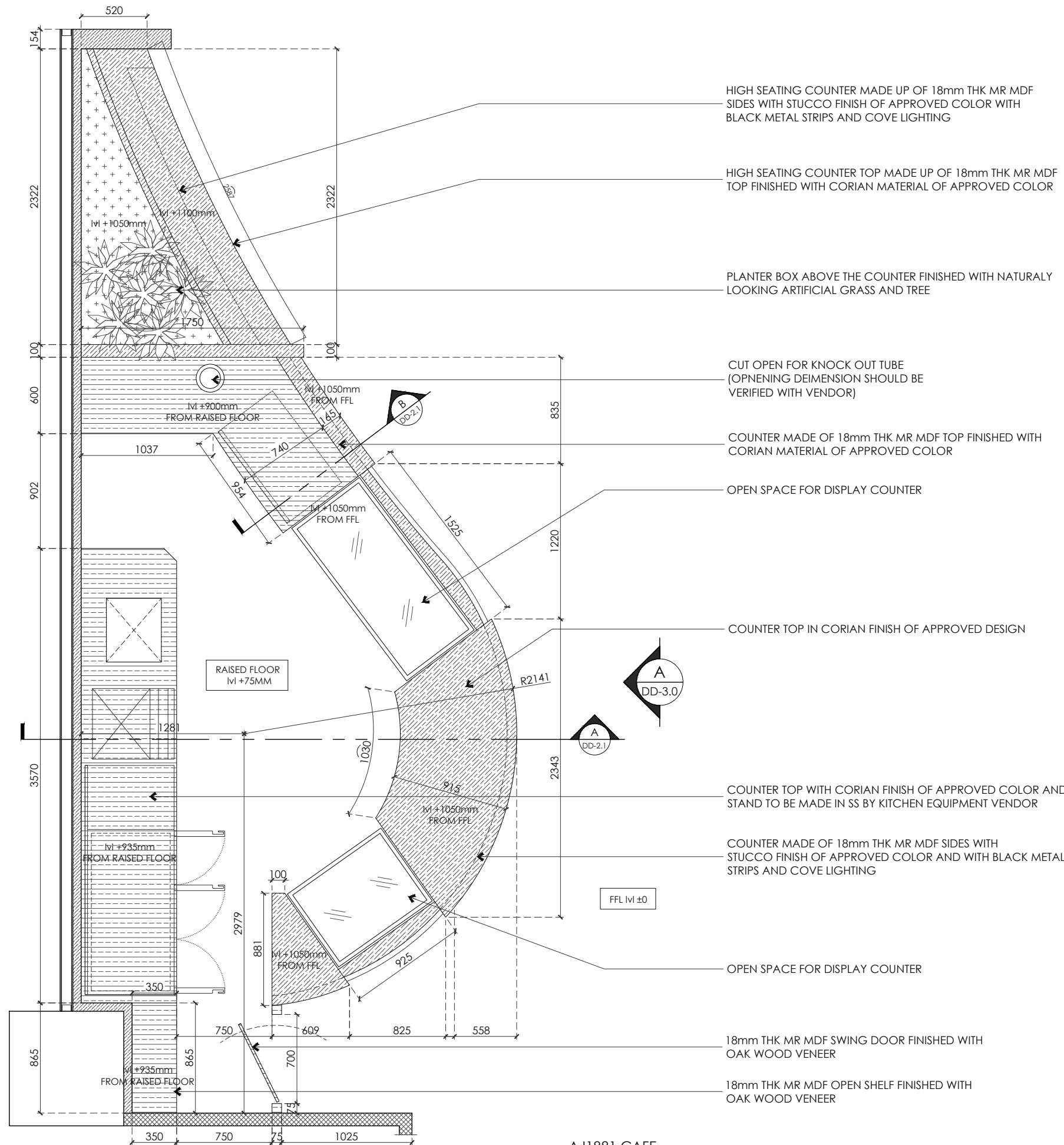
AJ1881 CAFE 1 TOP VIEW DD-1.0 SCALE 1:35 @ A3
