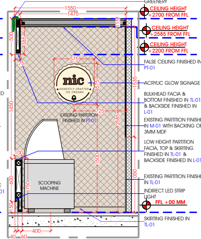
SECTIONAL ELEVATION BB'
