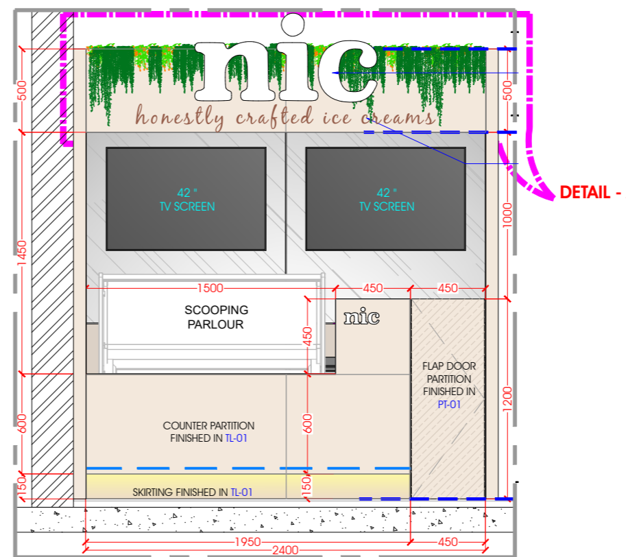
SECTIONAL ELEVATION EE'
