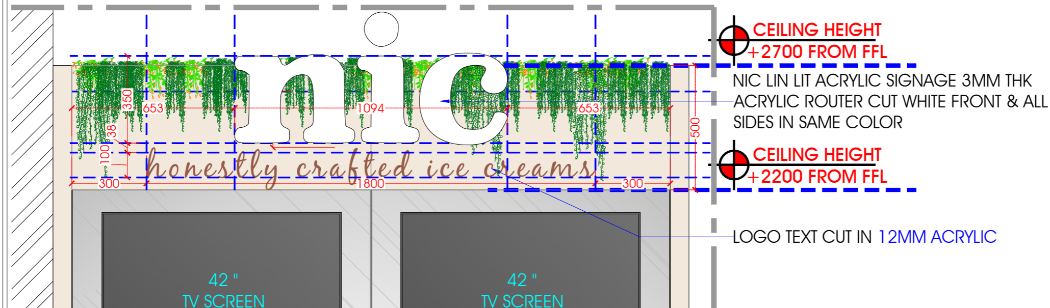
SIGNAGE DETAIL - A (GL-01 & AL-01)
