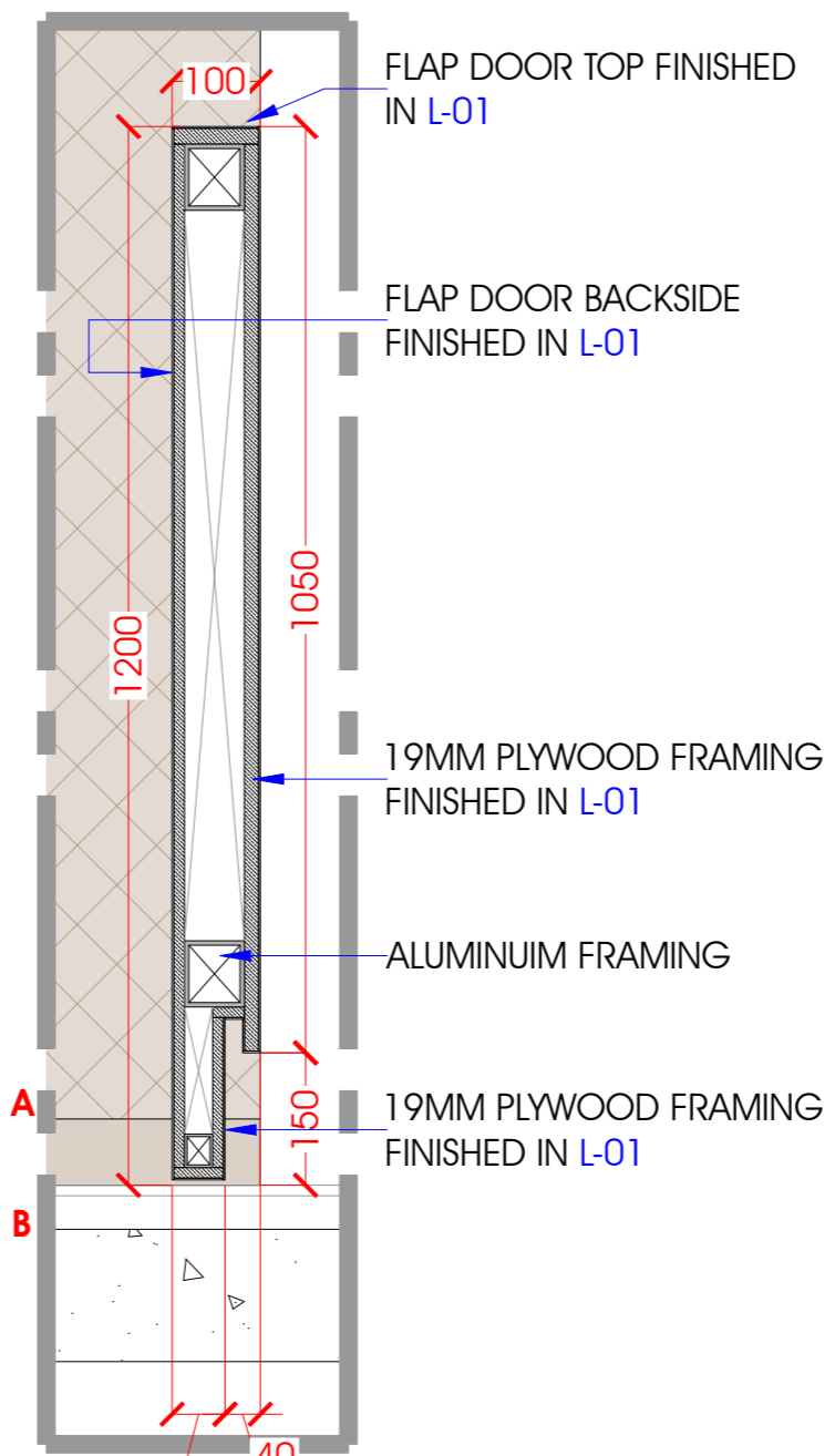
DETAIL - C (FLAP DOOR)
