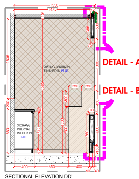
SECTIONAL ELEVATION DD'
