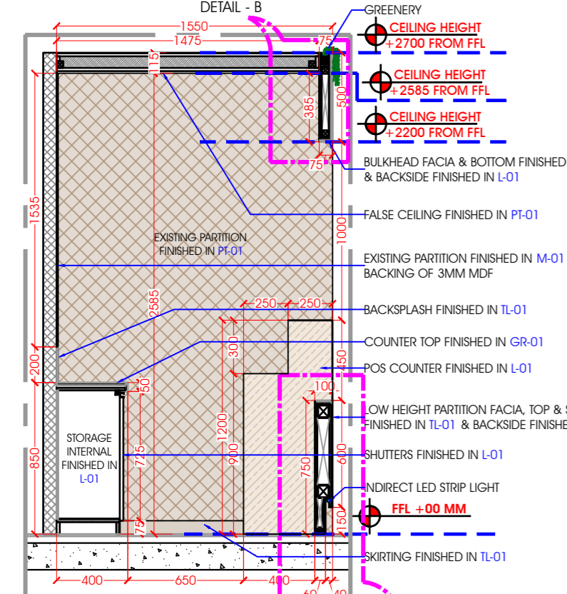
SECTIONAL ELEVATION DD'
