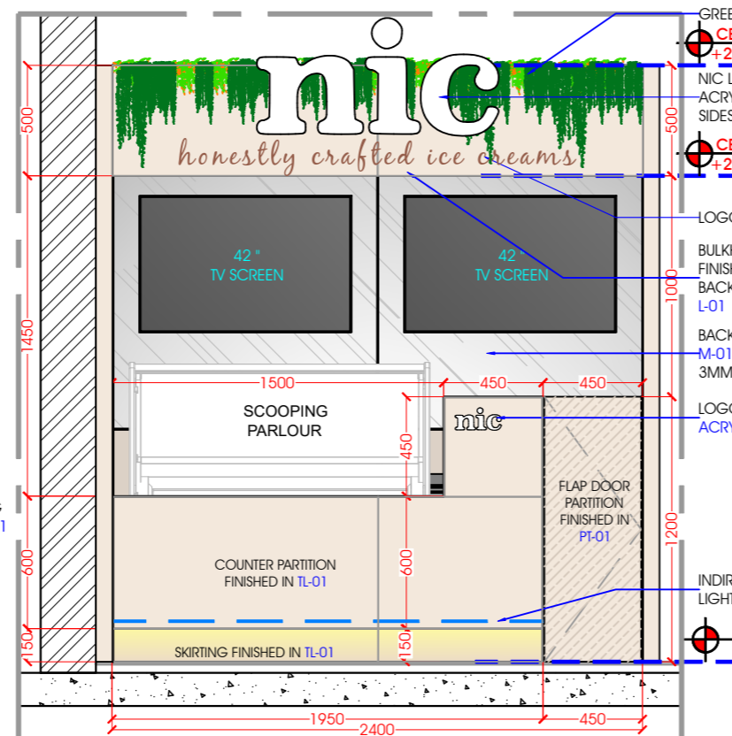
SECTIONAL ELEVATION EE'
