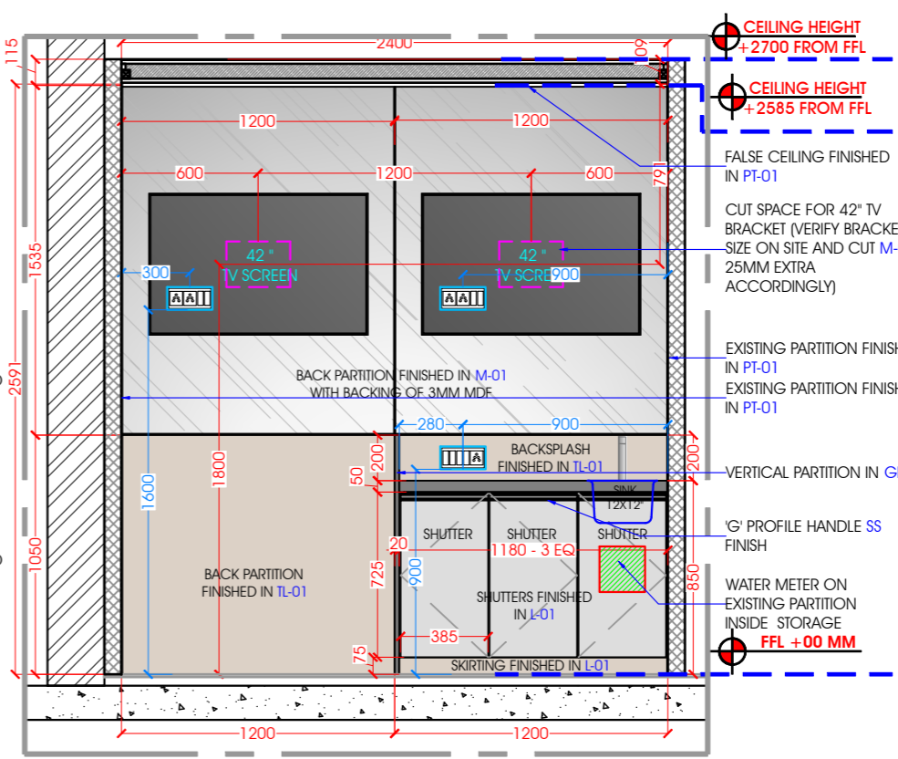
SECTIONAL ELEVATION CC'
