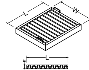
TYPICAL DETAIL FOR BAFFLE TYPE GREASE FILTER
