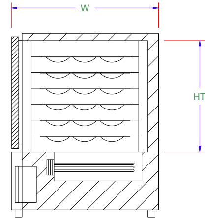
RHS SECTION
