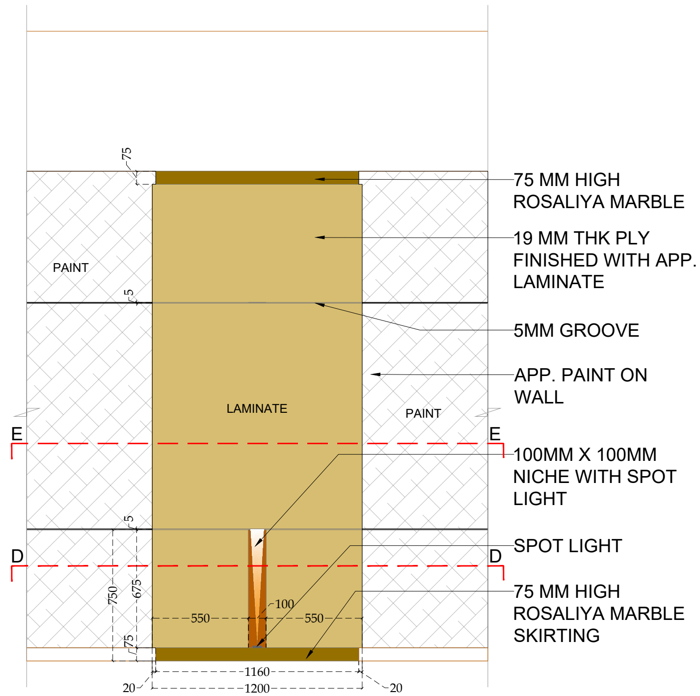
ELEVATION C
