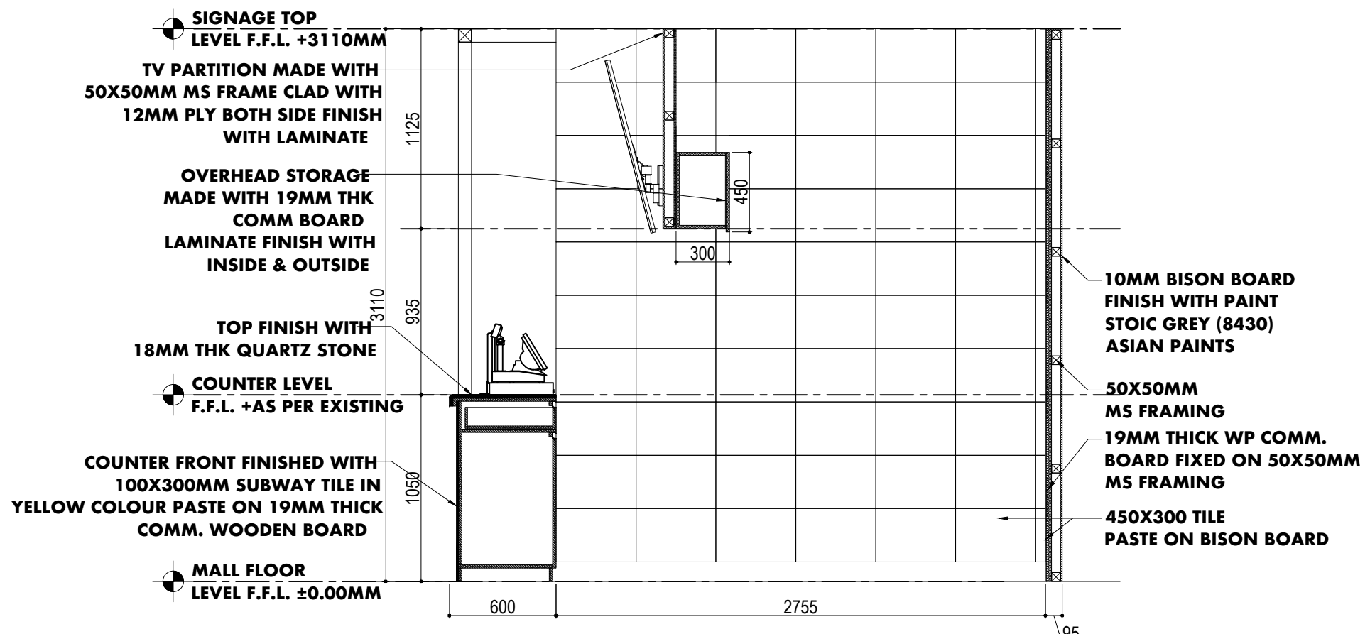
SECTION AA' 07
