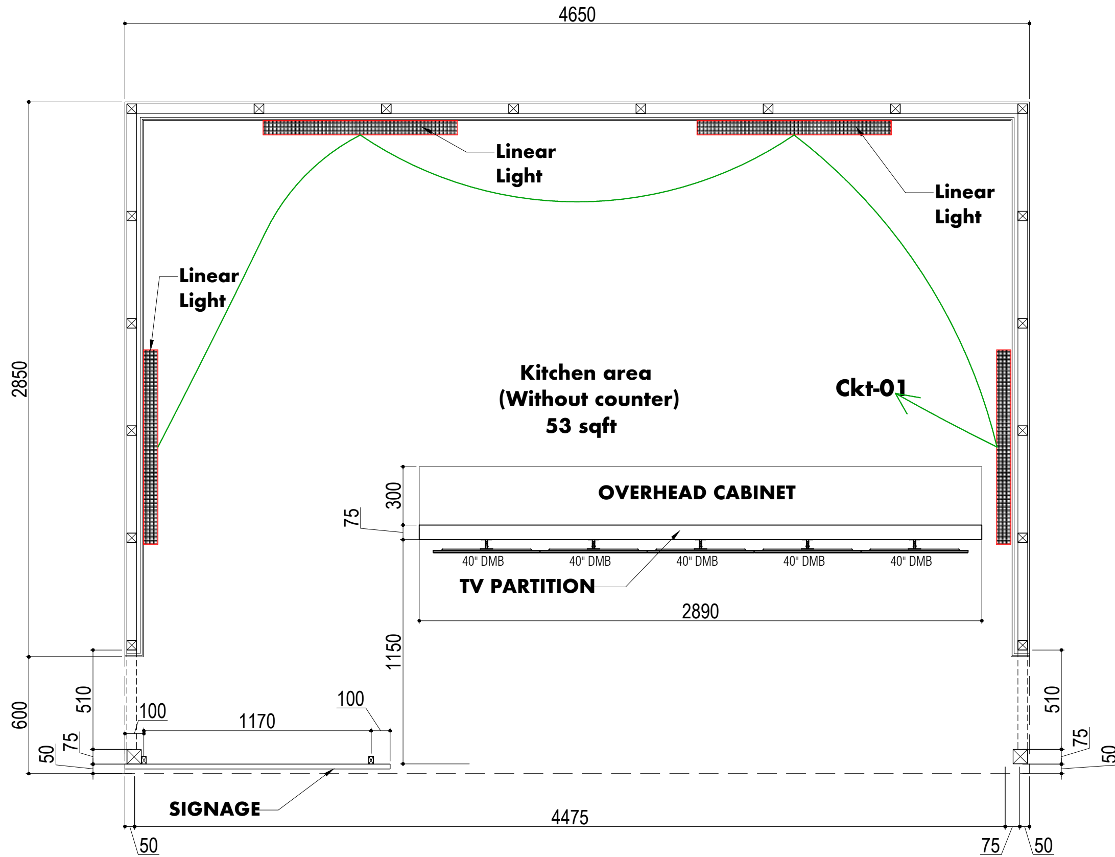
PLAN @Ceiling LEVEL 03
