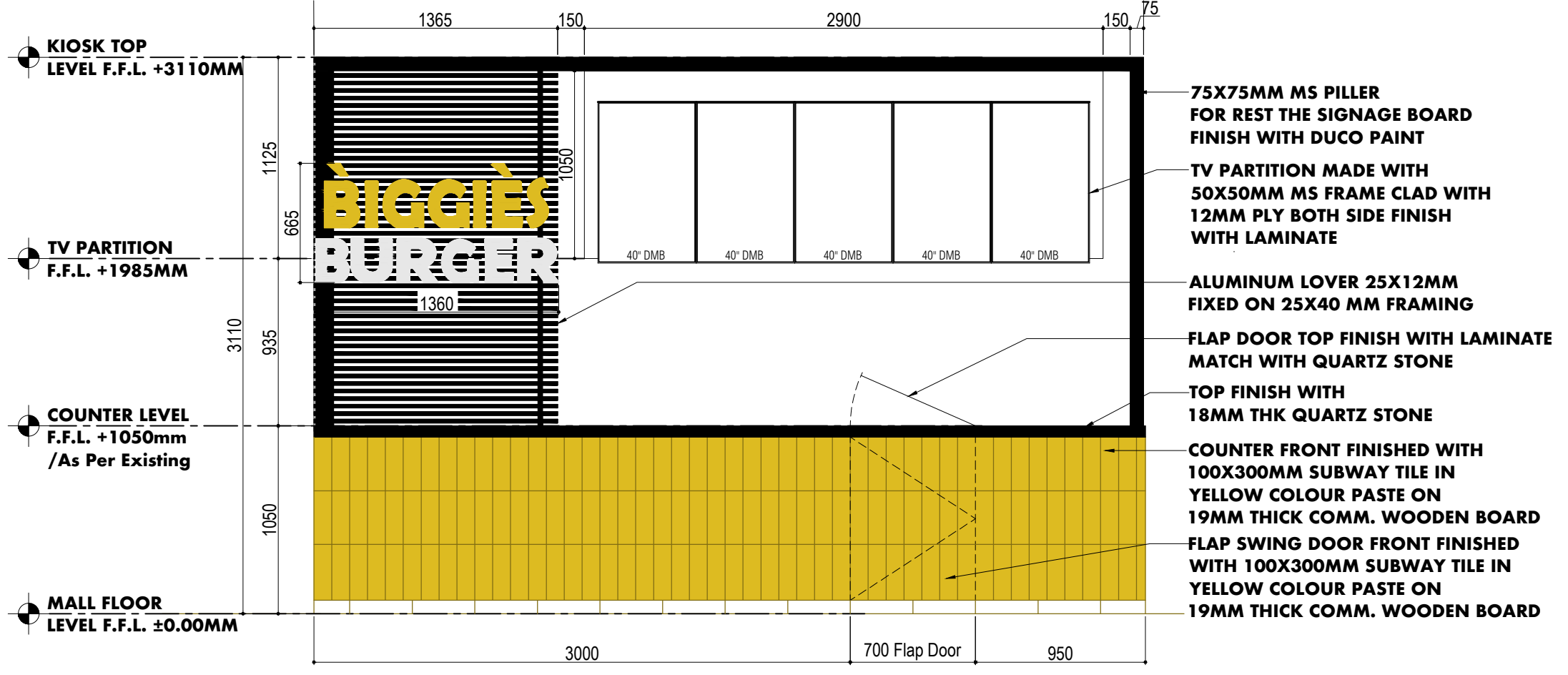
FRONT ELEVATION 08
