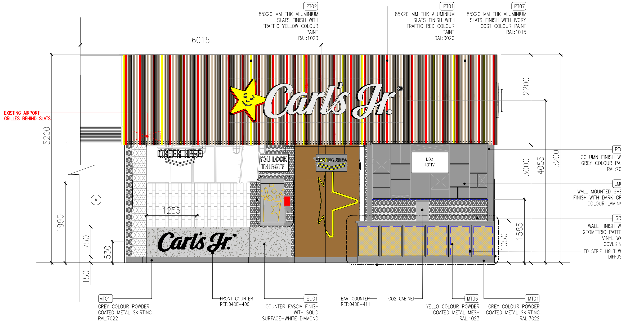
01 ELEVATION-01 OSL-300 1:50
