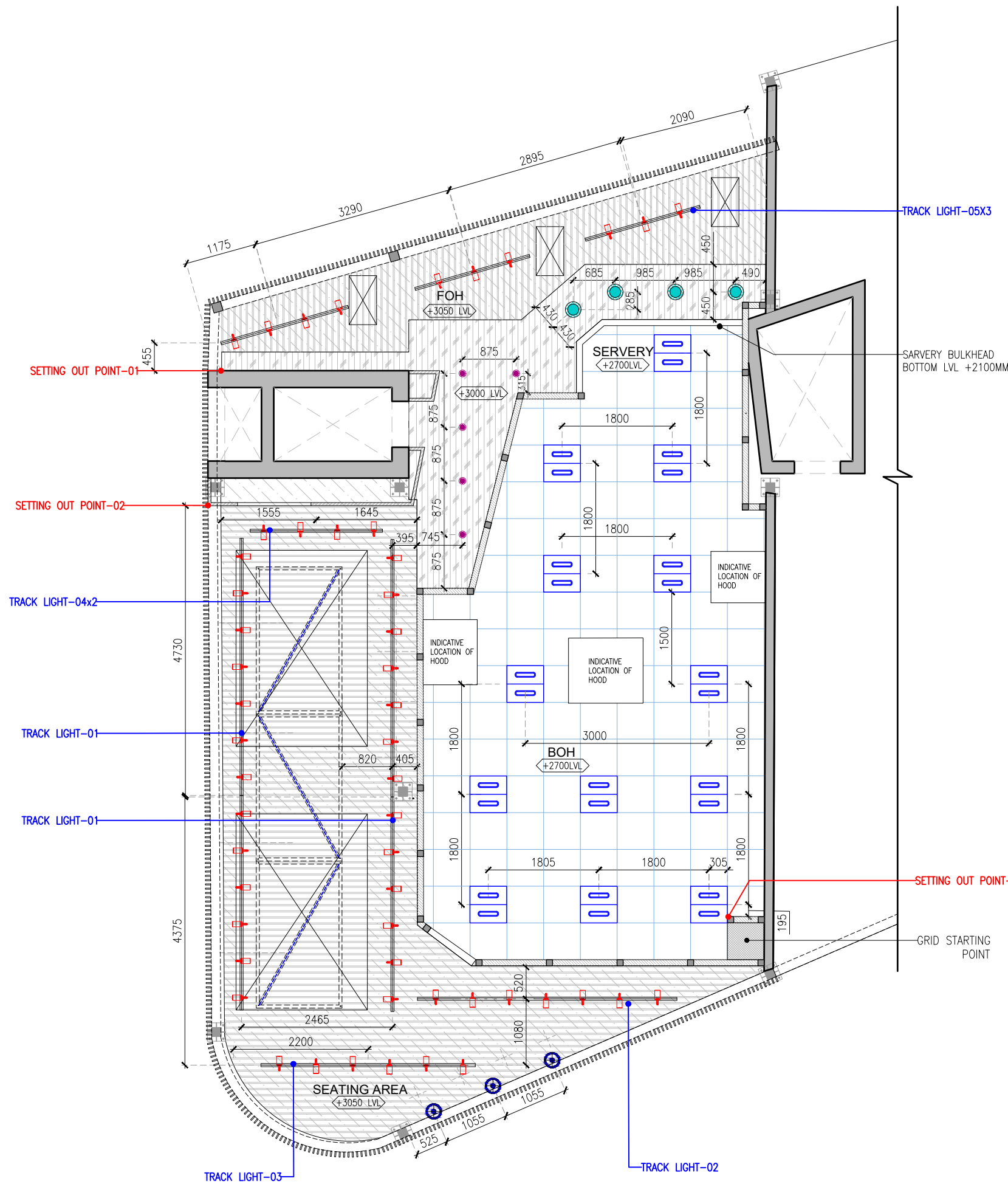
01 LIGHTING LAYOUT & SCHEDULE 02GA-104B 1:75
