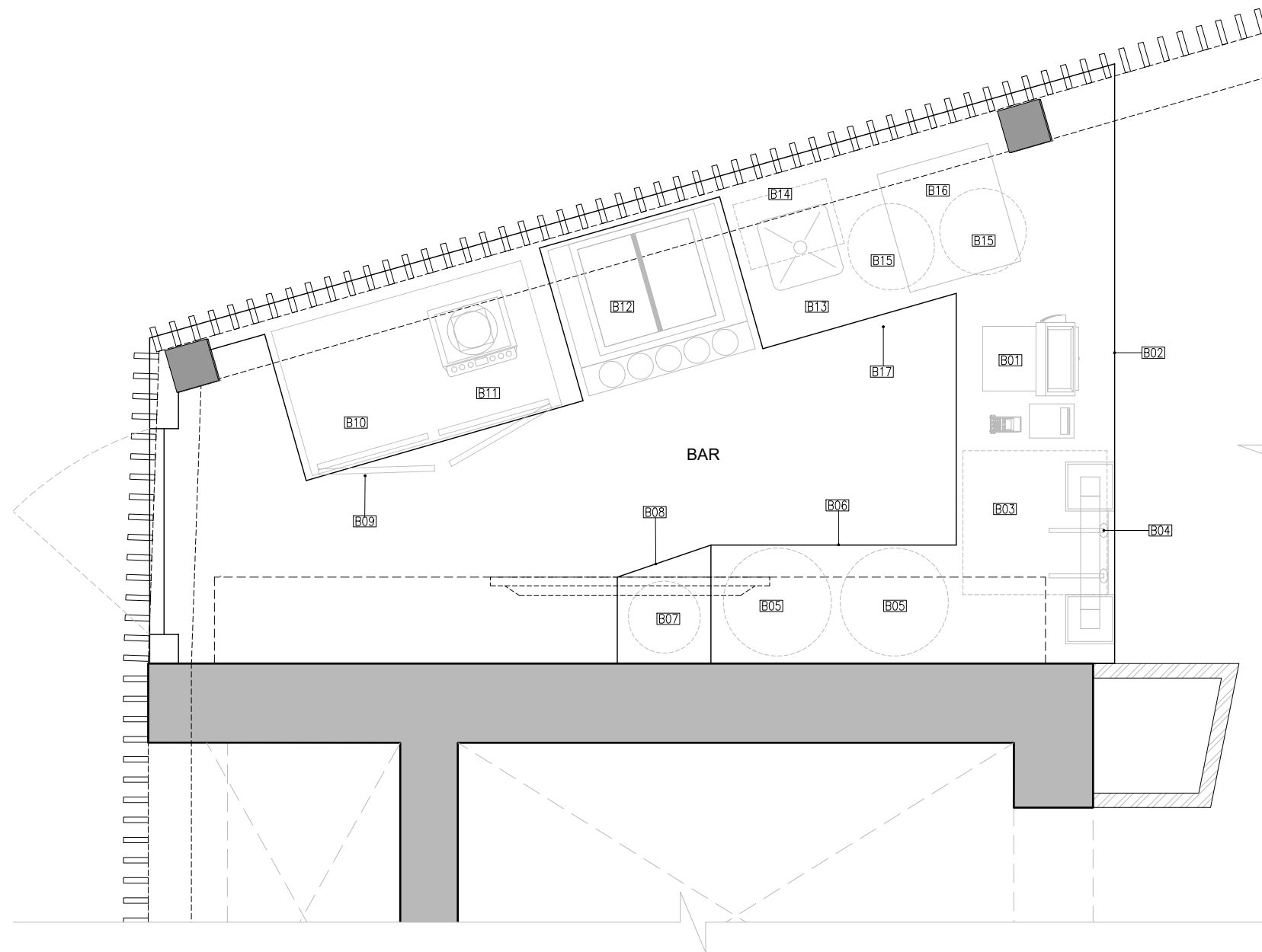
01 EQUIPMENT LAYOUT 02GA-106 1:75
