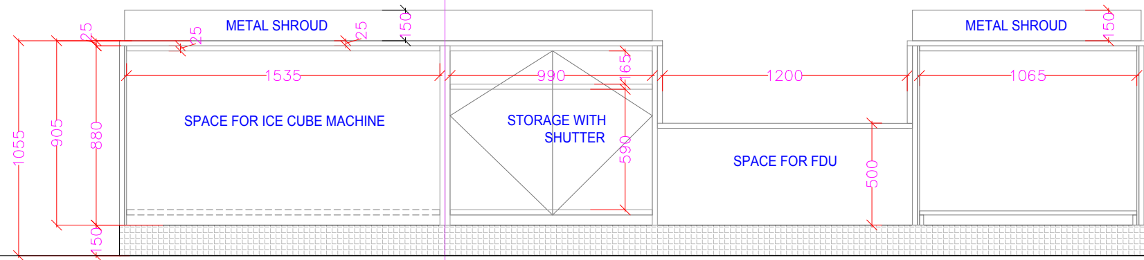
SECTION E
