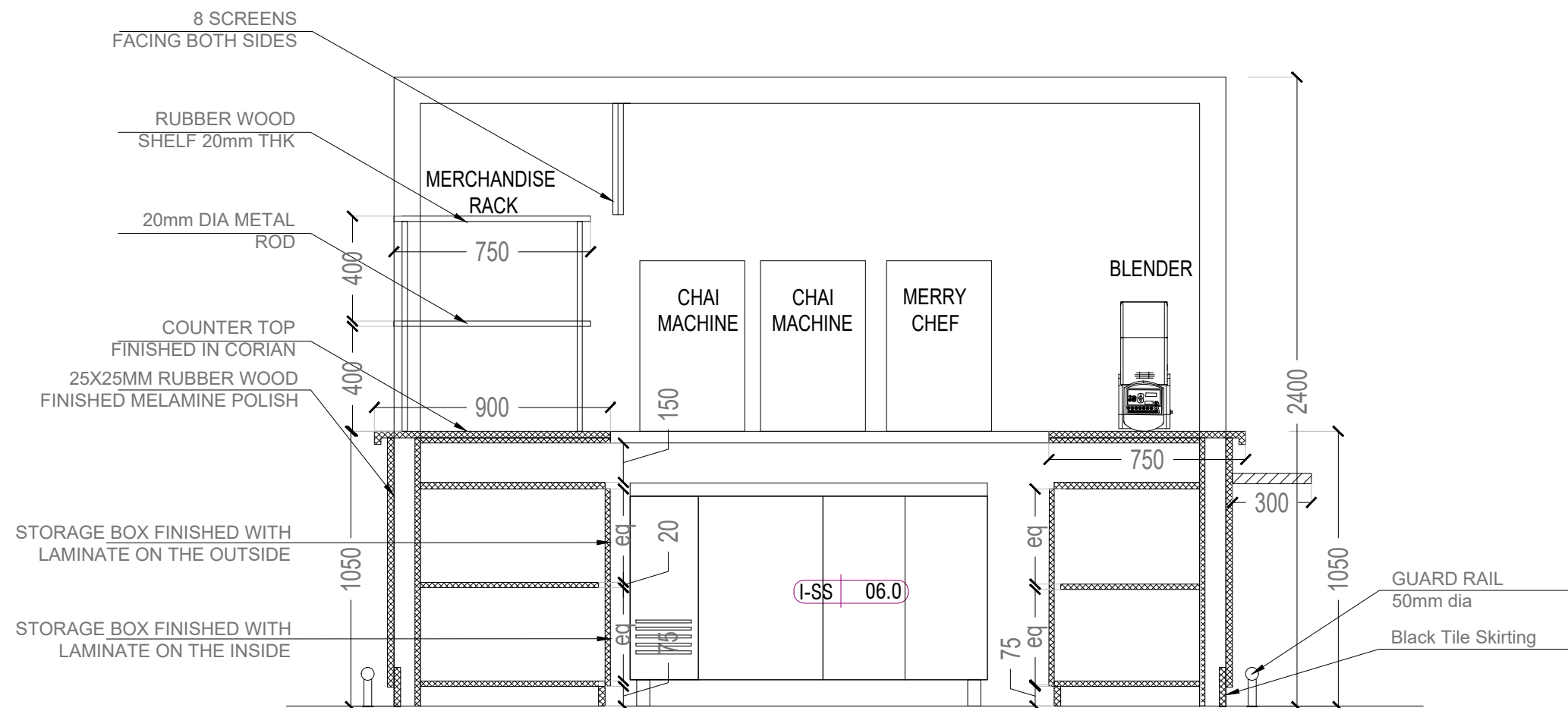
SECTION A
