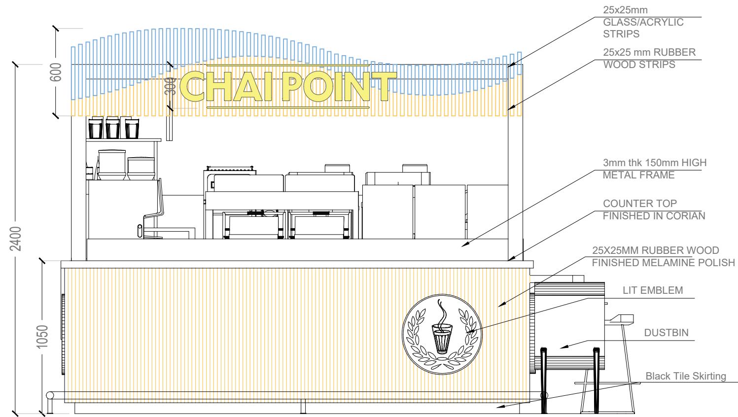
SIDE ELEVATION
