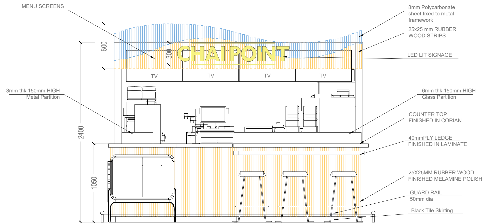
REAR ELEVATION
