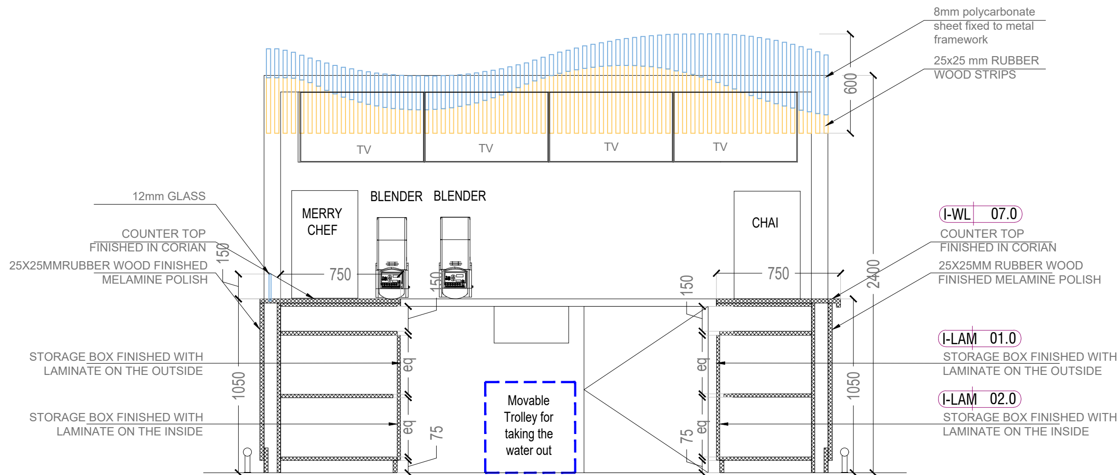
SECTION C
