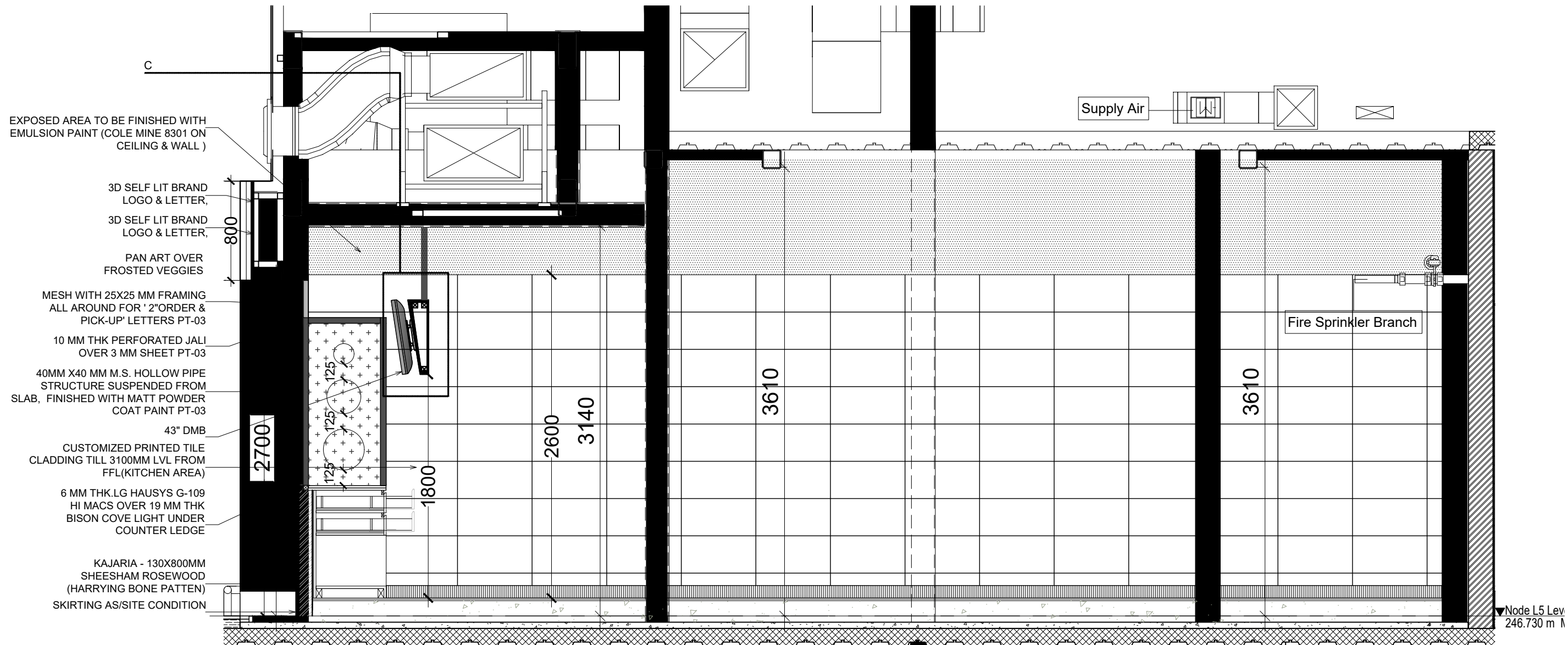
SECTION 'A' SCALE: NTS
