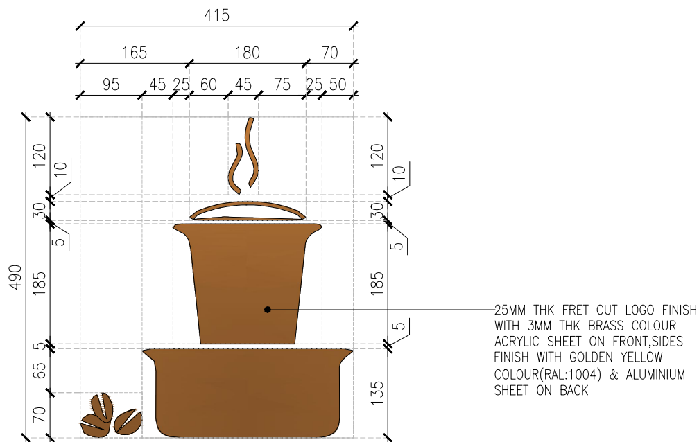
03 LOGO SIGNAGE-01 (LG01)(2NOS) 04DE-413 1:10
