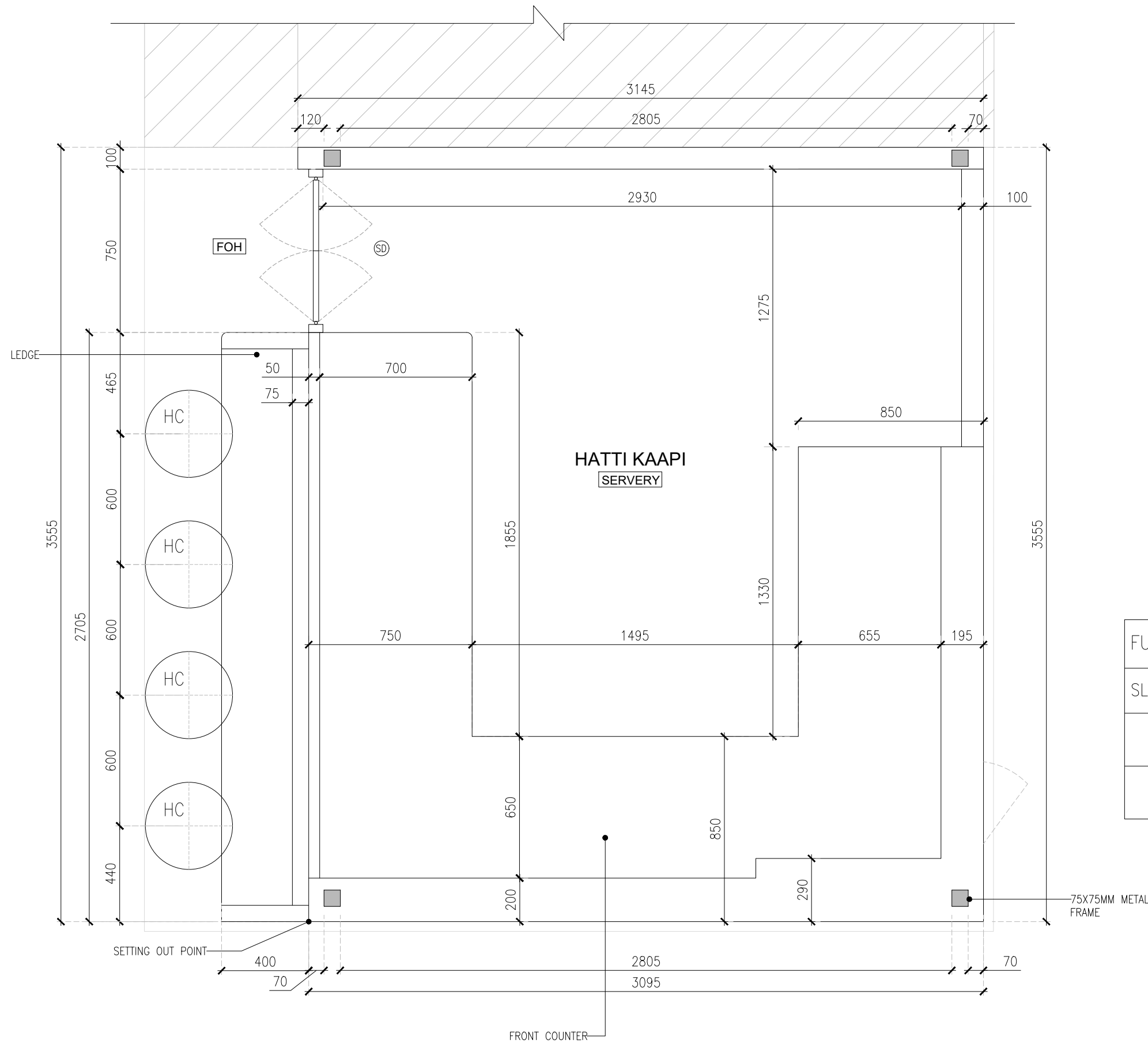
01 SETTING OUT PLAN 02GA-102 1:20
