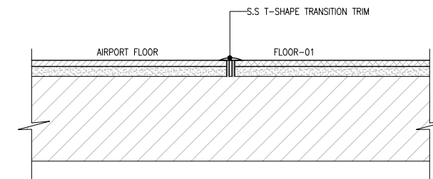
TYPICAL FLOOR TRANSITION DETAIL SECTION-A(SCALE 1:10)
