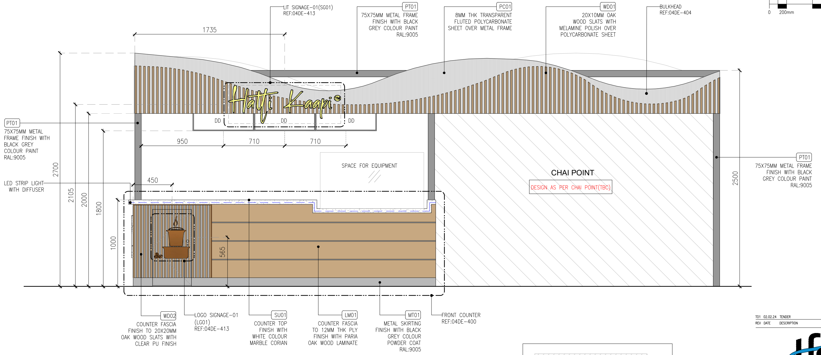
01 ELEVATION-01 03IL-300 1:25
