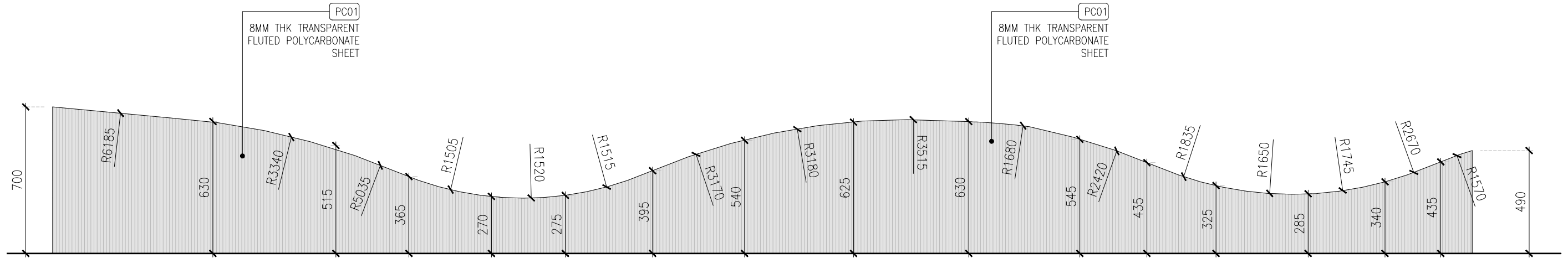
DETAIL-B(POLYCARBONATE SHEET)
