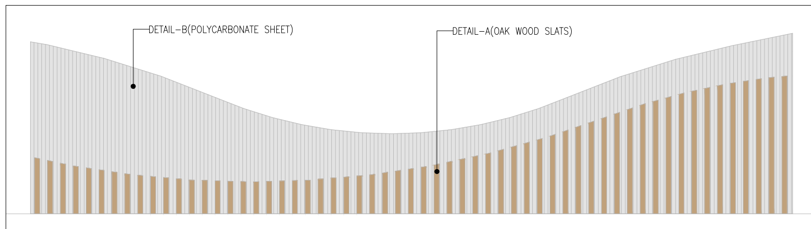
KEY PLAN(ELEVATION-02)
