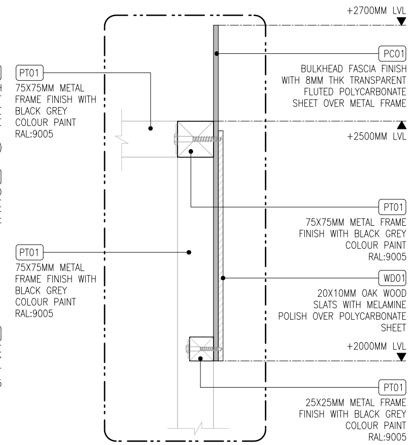
DETAIL-A (SCALE 1:10)
