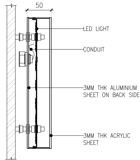
TYPICAL SECTION OF FRONT LIT SIGNAGE
