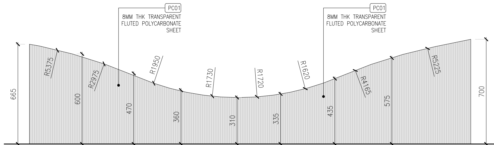
DETAIL-B(POLYCARBONATE SHEET)
