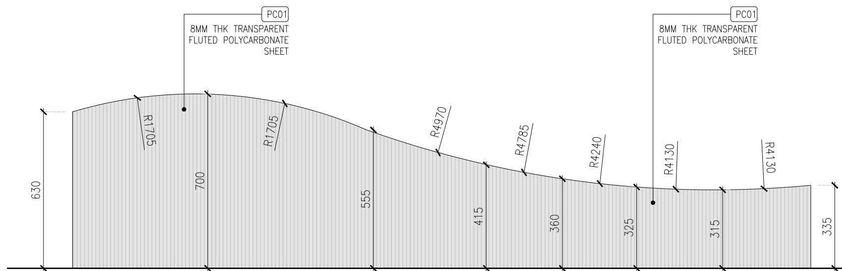
DETAIL-B(POLYCARBONATE SHEET)
