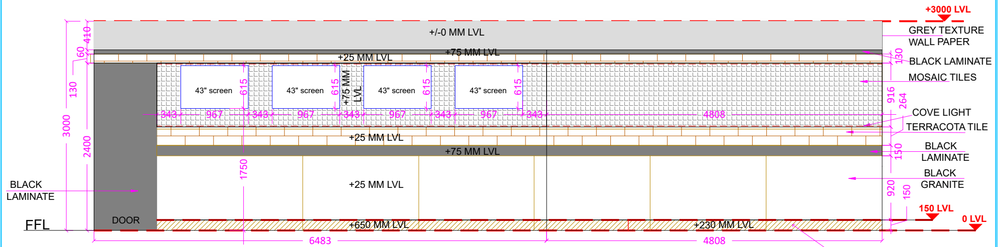
INTERIOR WALL ELEVATION
