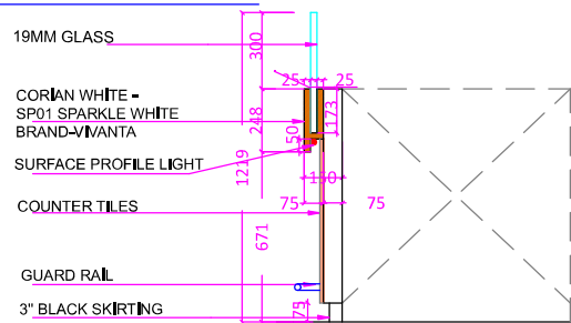
COUNTER FRONT ELEVATION
