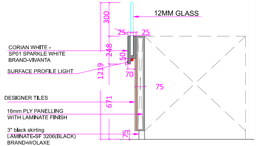
SECTION-XX'
