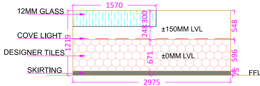
COUNTER FRONT ELEVATION
