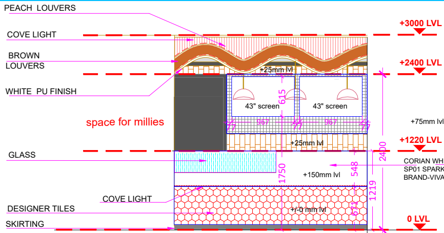
FRONT EXTERIOR ELEVATION
