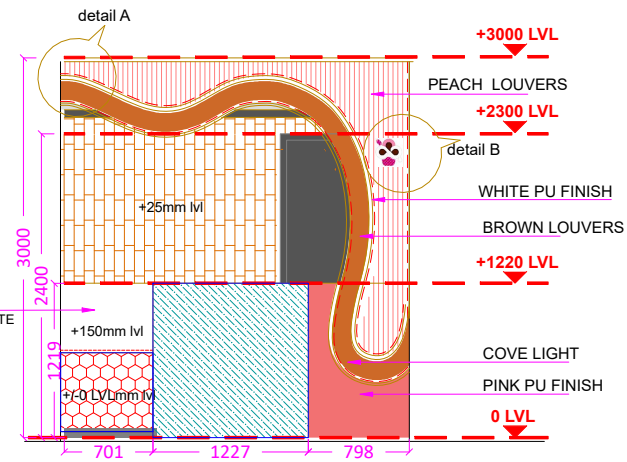
SIDE EXTERIOR ELEVATION
