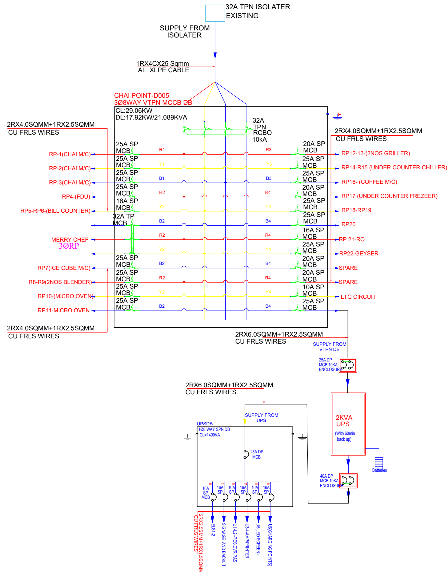
MAIN SINGLE LINE DIAGRAM
