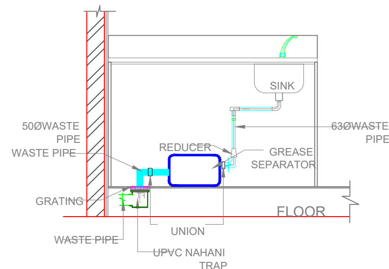
TYPICAL ARRANGEMENT FOR GREASE SEPARATOR
