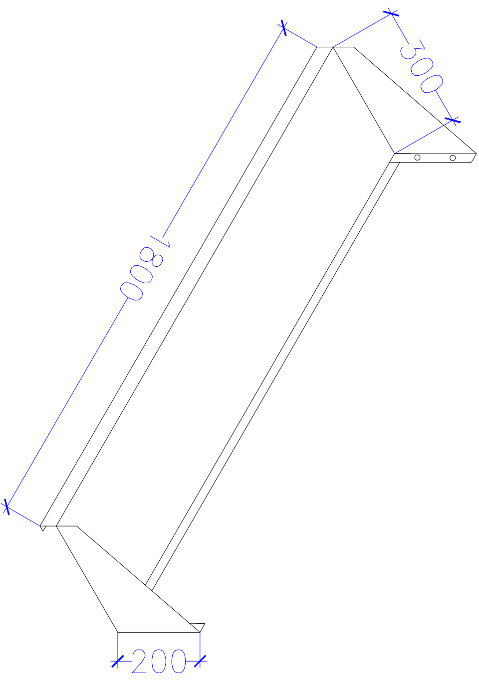
OVERHEAD SHELF (1800MMX300MM)
