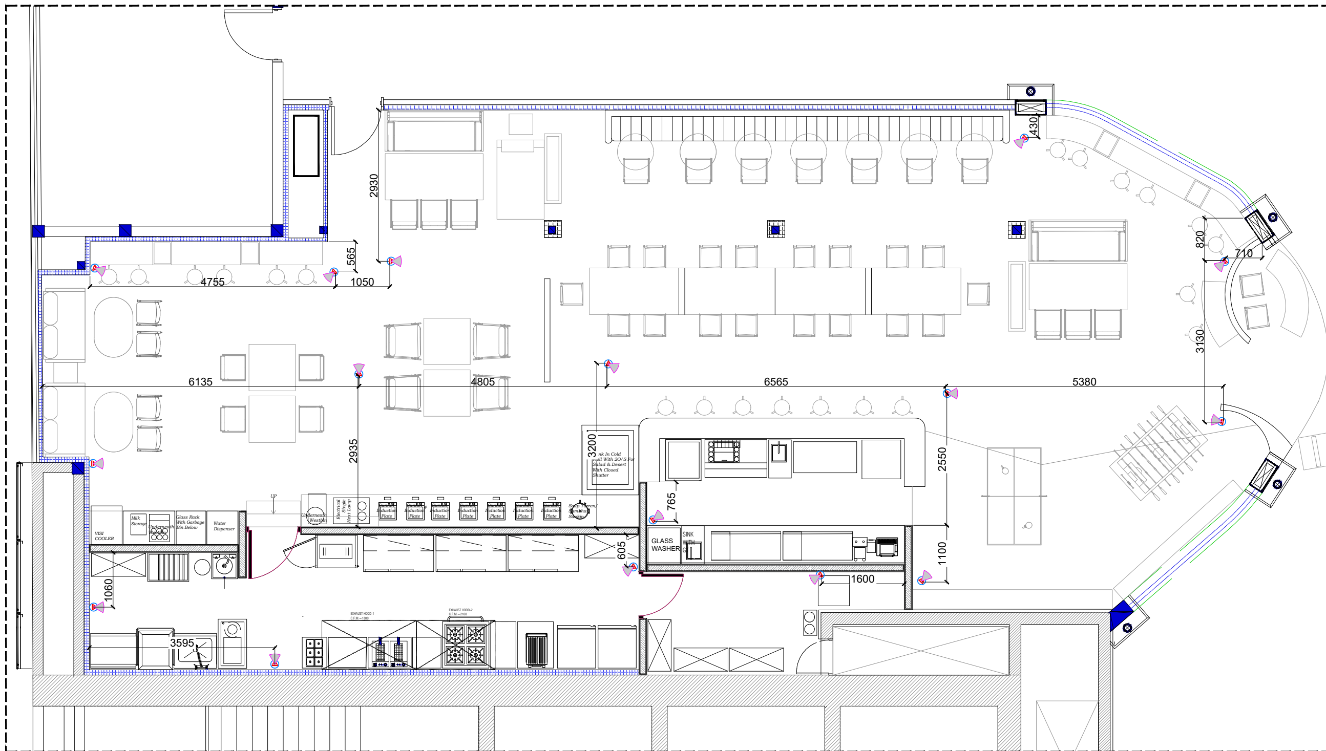
1 CCTV LAYOUT & WORKING Scale:-1:75
