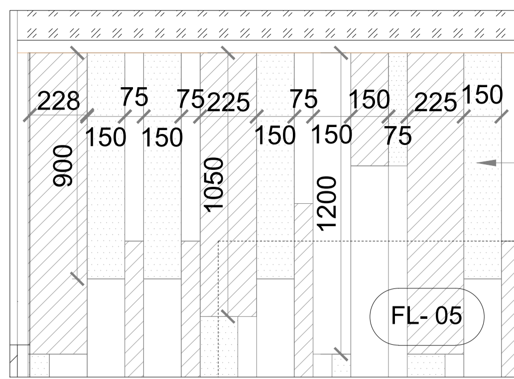
FLOORING PATTERN PLAN ( DETAIL -1) SCALE:1:15
