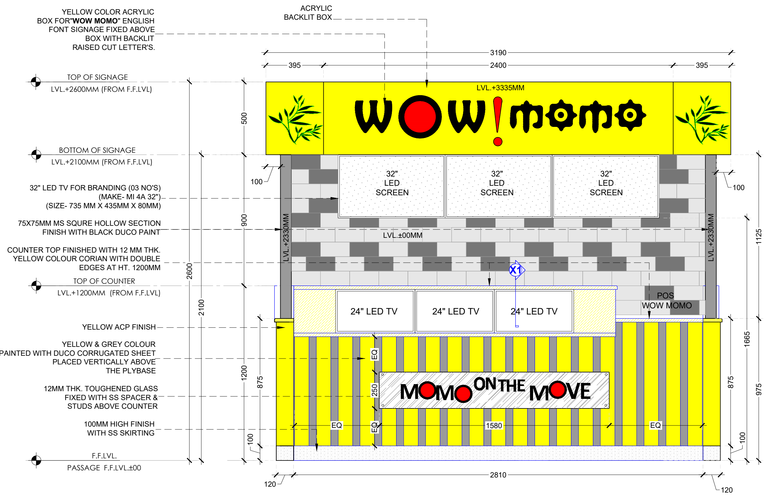
FRONT ELEVATION
