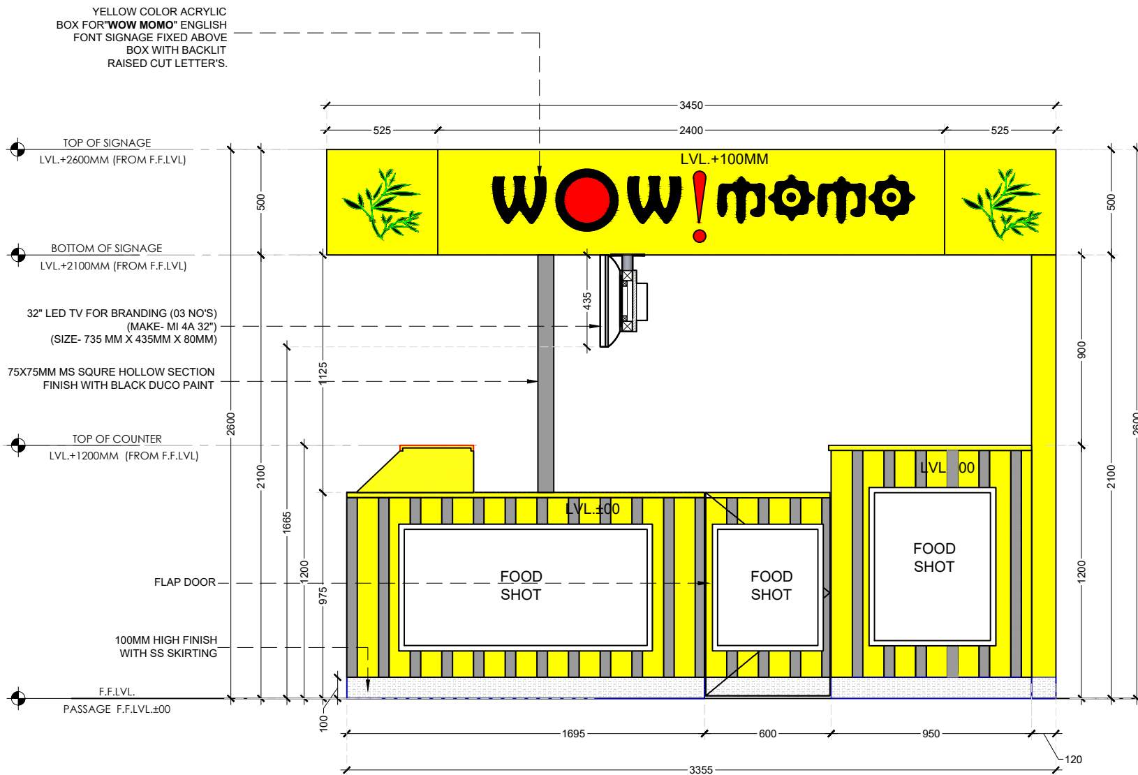
SECTIONAL ELEVATION BB
