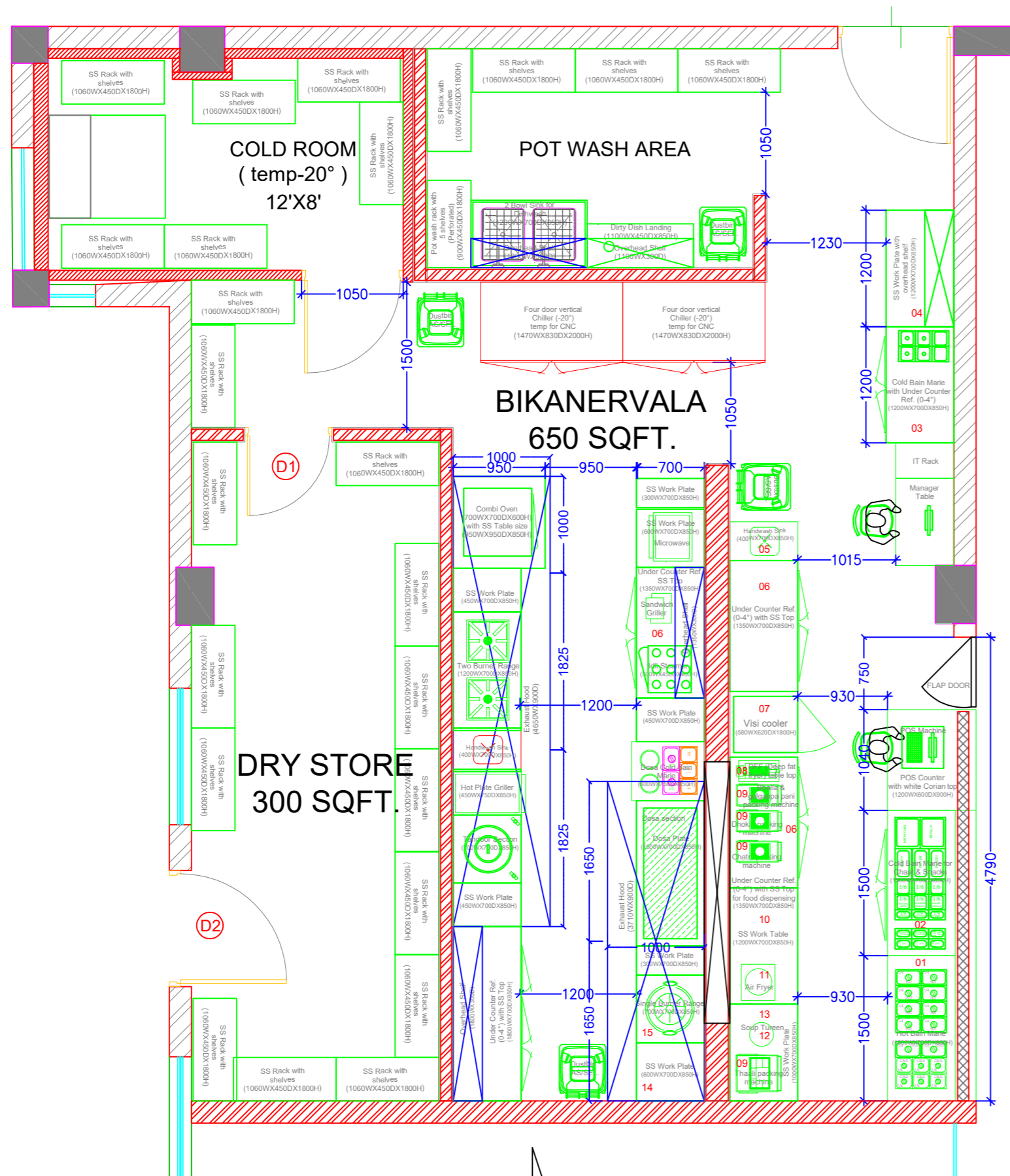
BIKANERVALA EQUIPMENT LAYOUT
