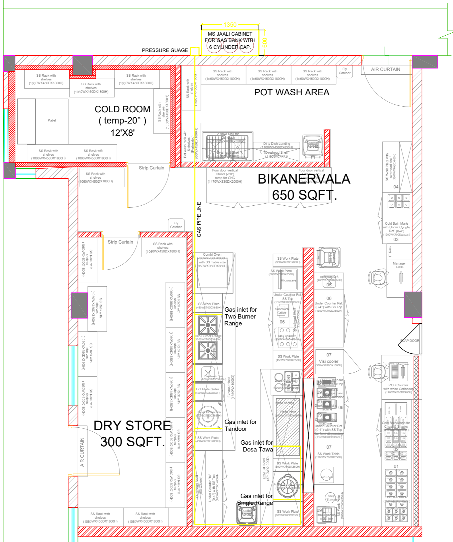
Bikanervala Gas Bank Layout
