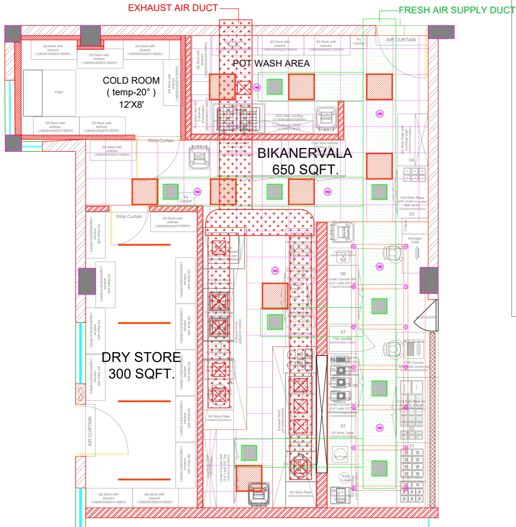
Bikanervala Coordinated RCP Layout
