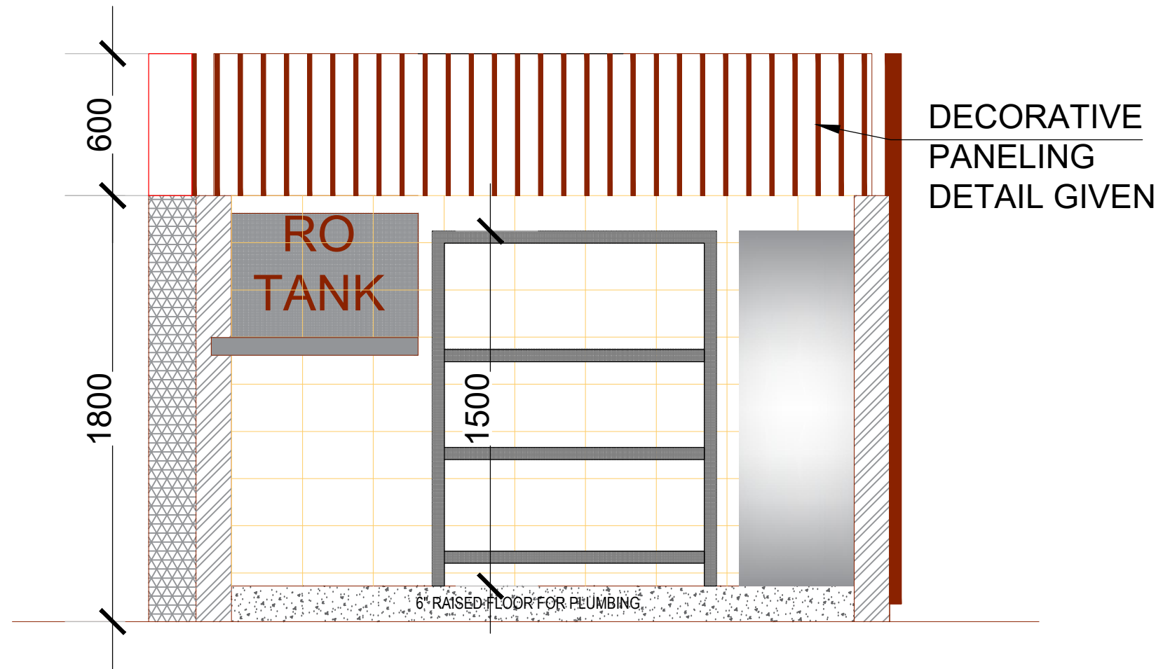
ELEVATION E-E
