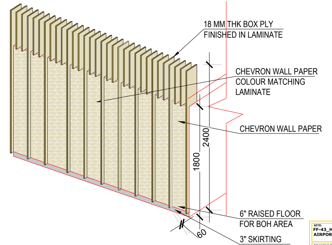
ISOMETRIC VIEW
