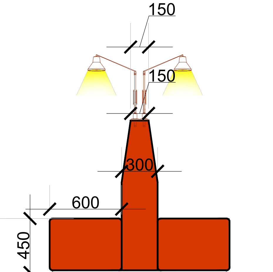
SIDE ELEVATION
