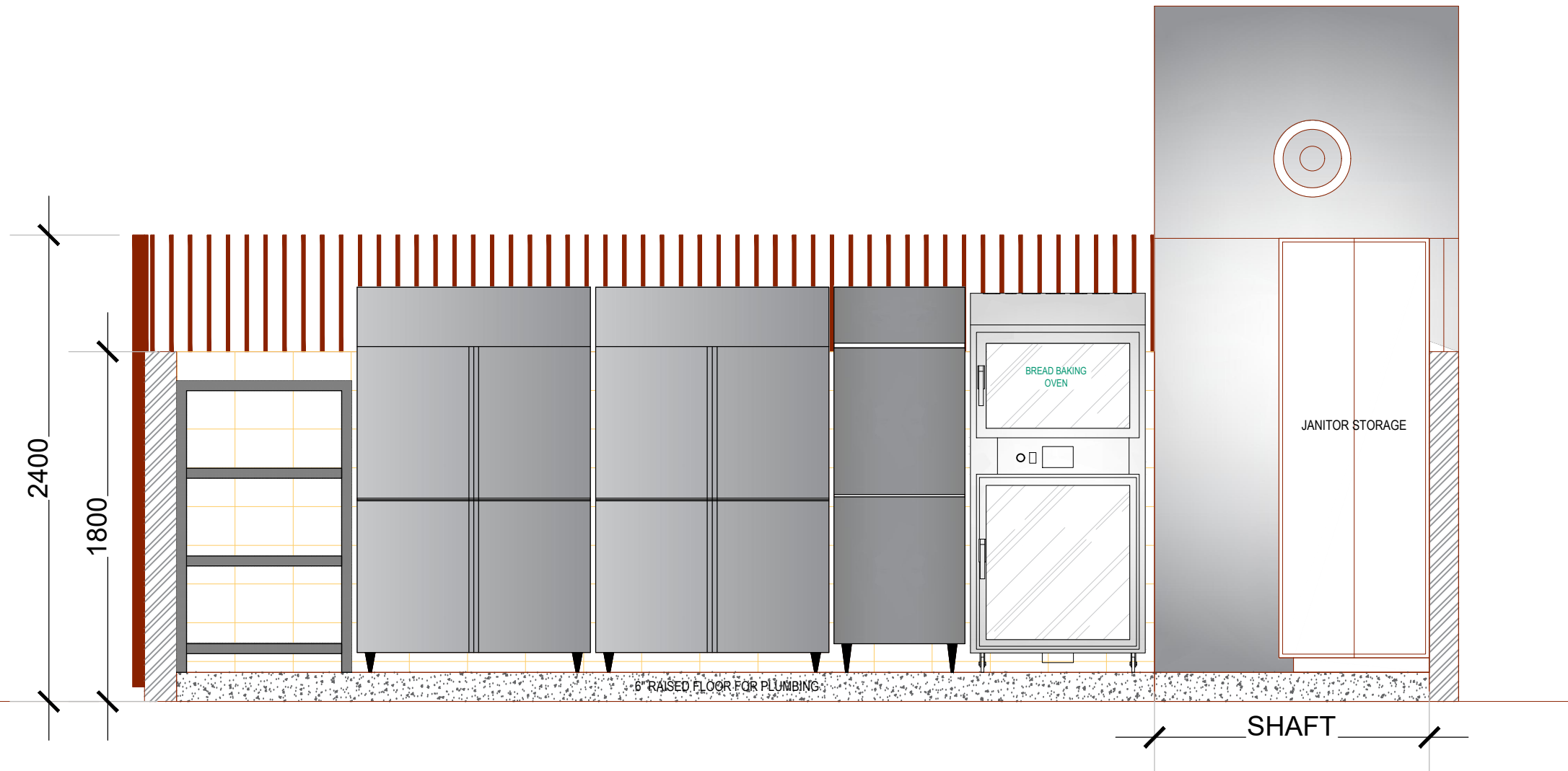
ELEVATION F-F
