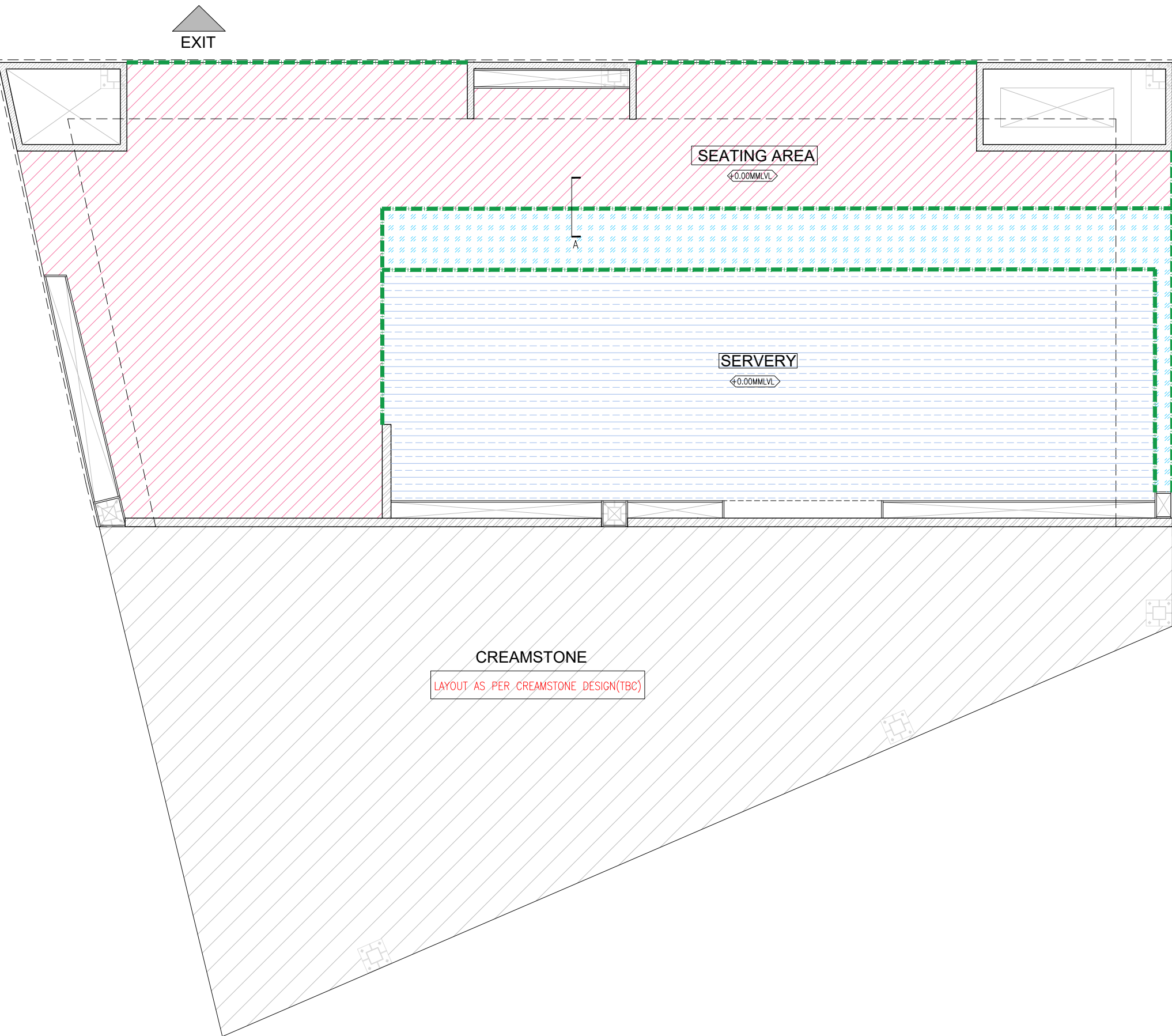
01 FLOORING LAYOUT 02GA-105 1:50
