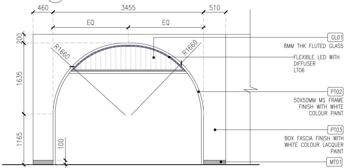
03 FACADE FRAMING (ELEVATION-01) 04DE-414 1:50
