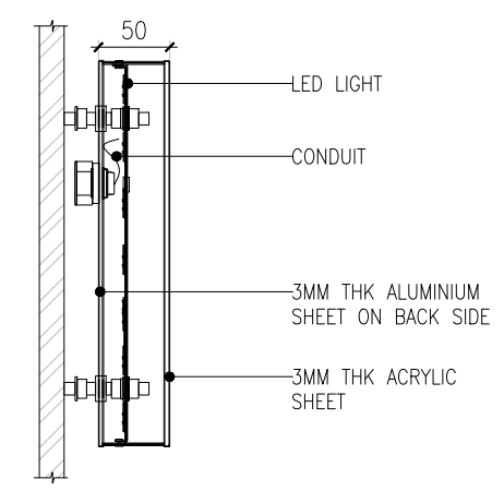
TYPICAL SECTION OF FRONT LIT SIGNAGE
