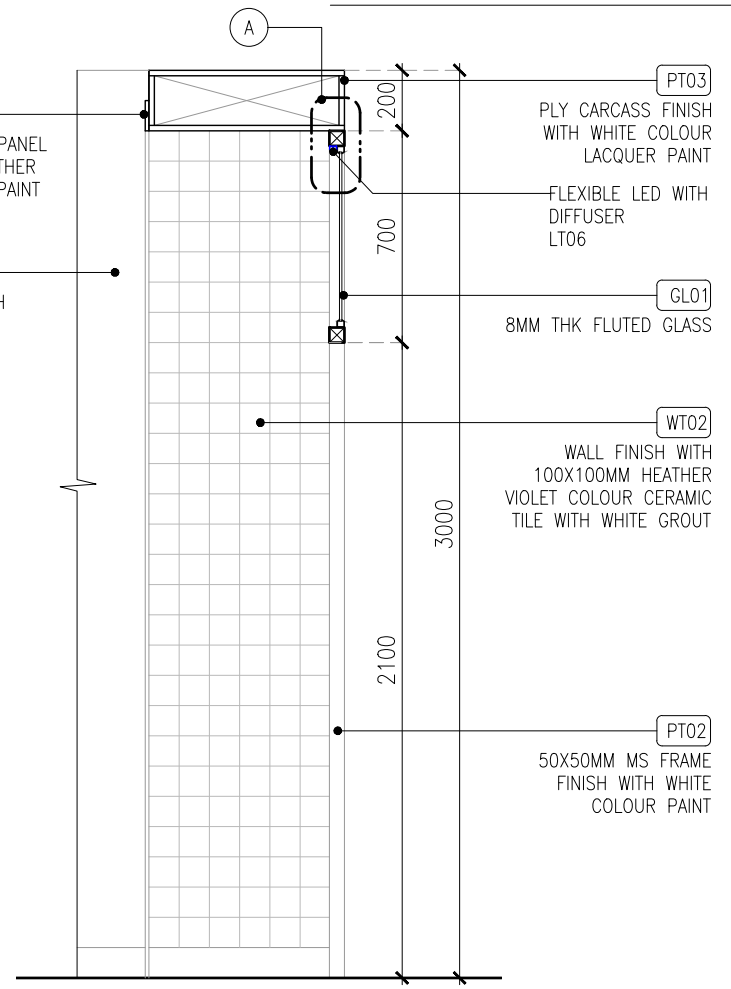
TYPICAL SECTION-A (SCALE 1:25)
