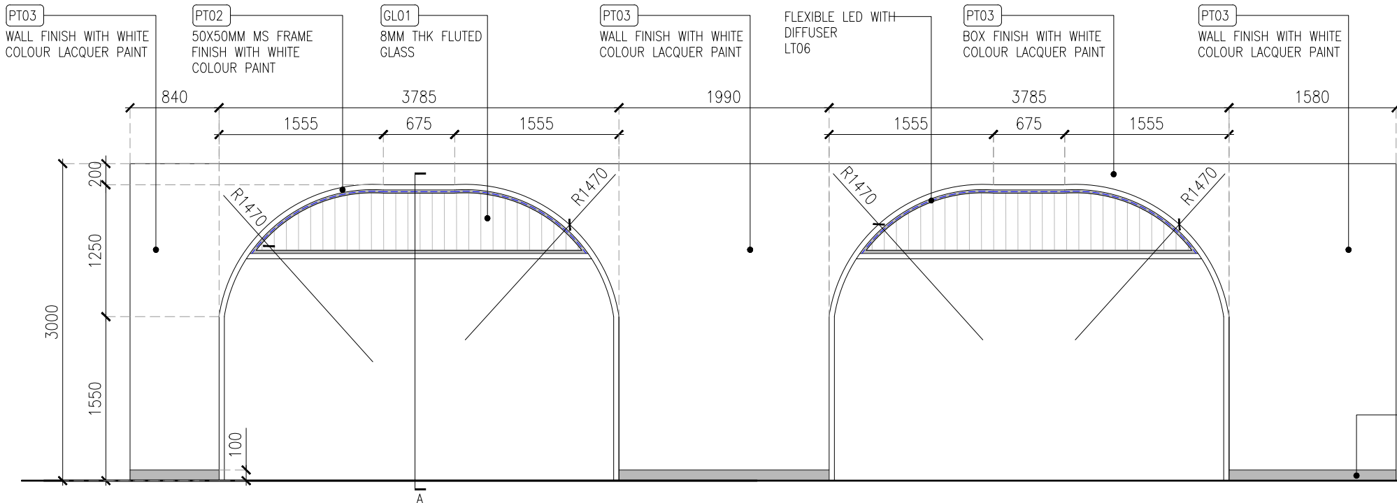
01 FACADE FRAMING (ELEVATION-02) 04DE-414 1:50
