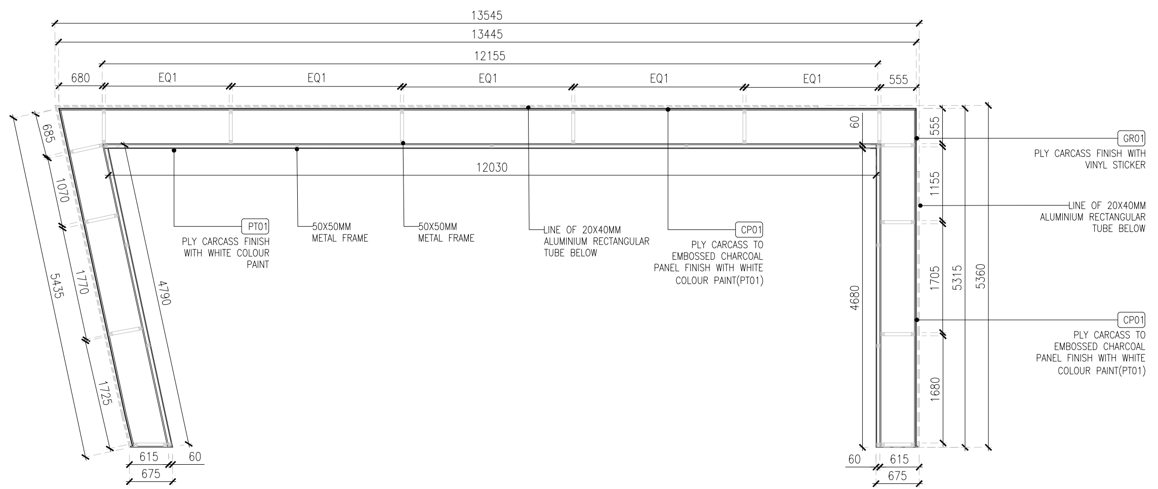
FRAMING PLAN @ 500MM LVL
