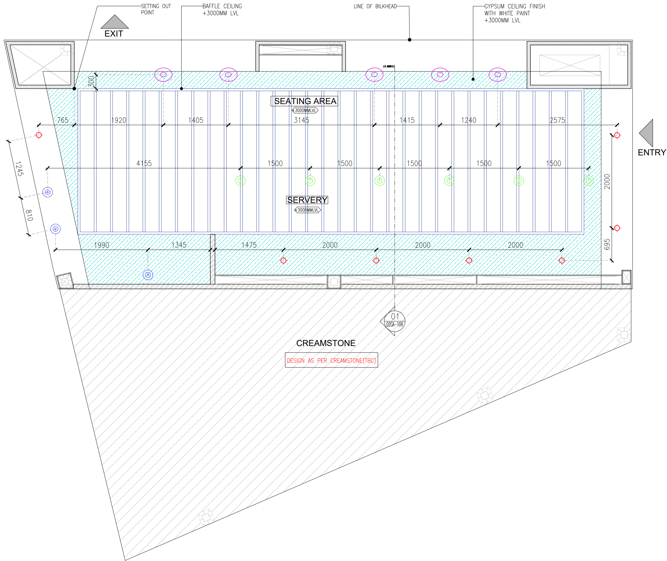
01 RCP + LIGHTING LAYOUT :PART-A 02GA-103 1:50
