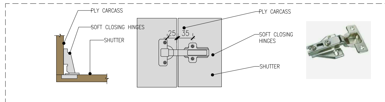
DETAIL A: STAINLESS STEEL HINGE FIXING DETAIL
