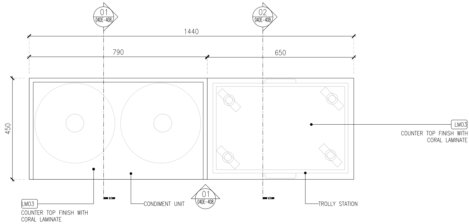
TOP PLAN
