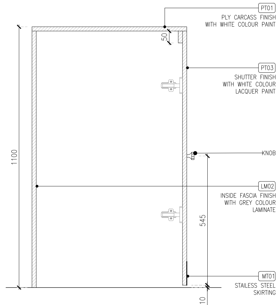
SECTION-A(SCALE 1:10)
