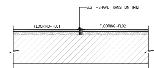
TYPICAL FLOOR TRANSITION DETAIL SECTION-A
