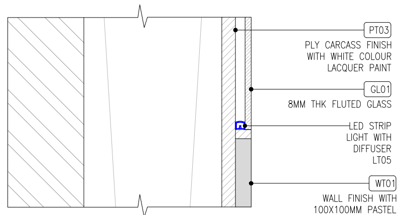
SECTION -A(SCALE 1:5)
