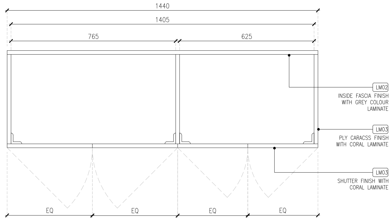
FRAMING PLAN @ 500MM LVL
