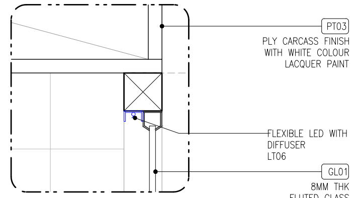
DETAIL-A(SCALE 1:5)
