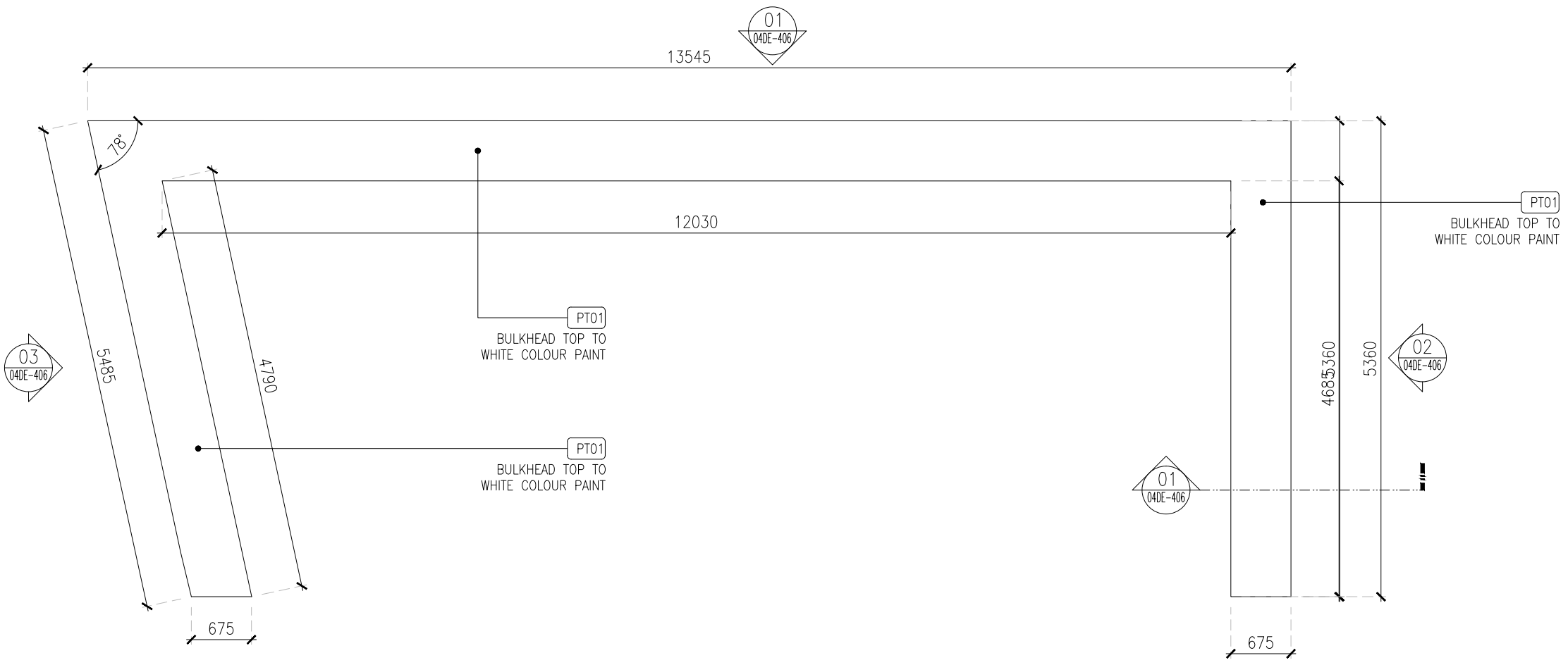
TOP PLAN
