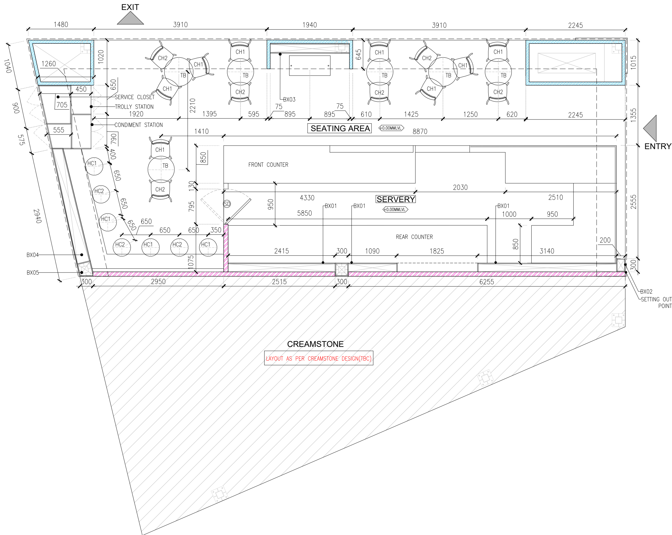
01 SETTING OUT PLAN 02GA-102 1:50
