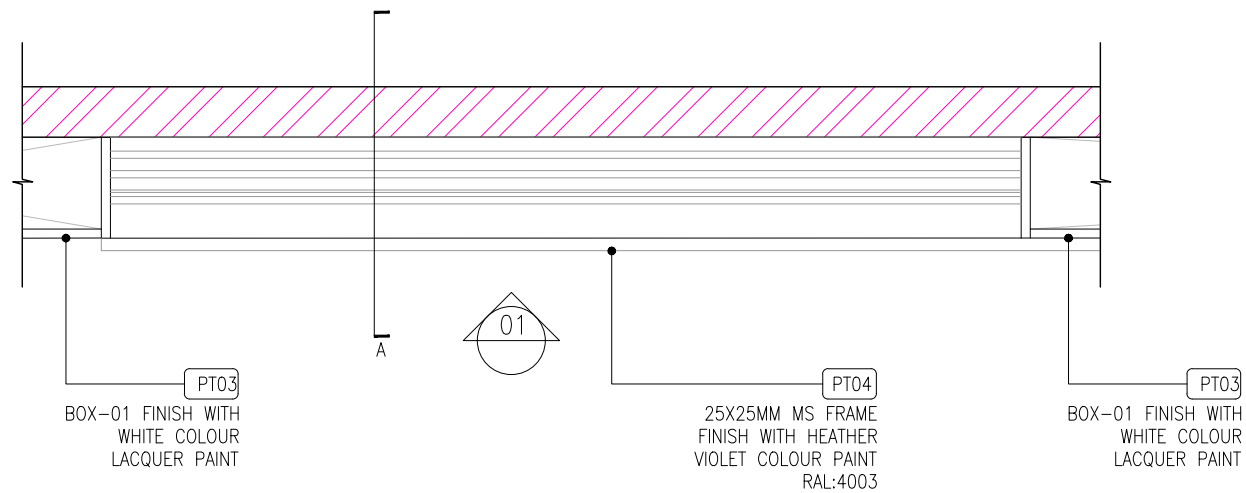
FRAMING PLAN @500MM LVL (SCALE 1:15)
