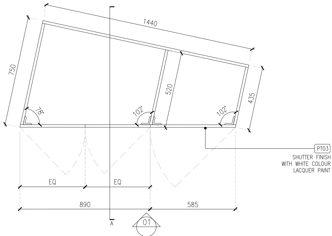
FRAMING PLAN @ 500MM LVL(SCALE 1:15)
