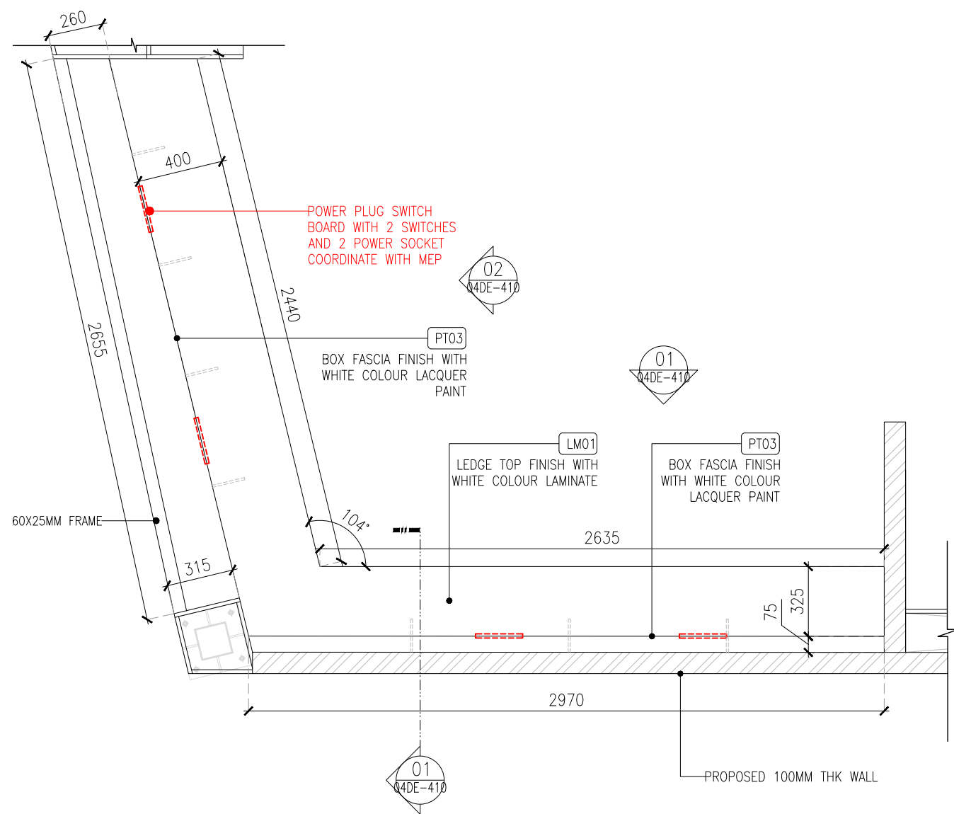
TOP PLAN
