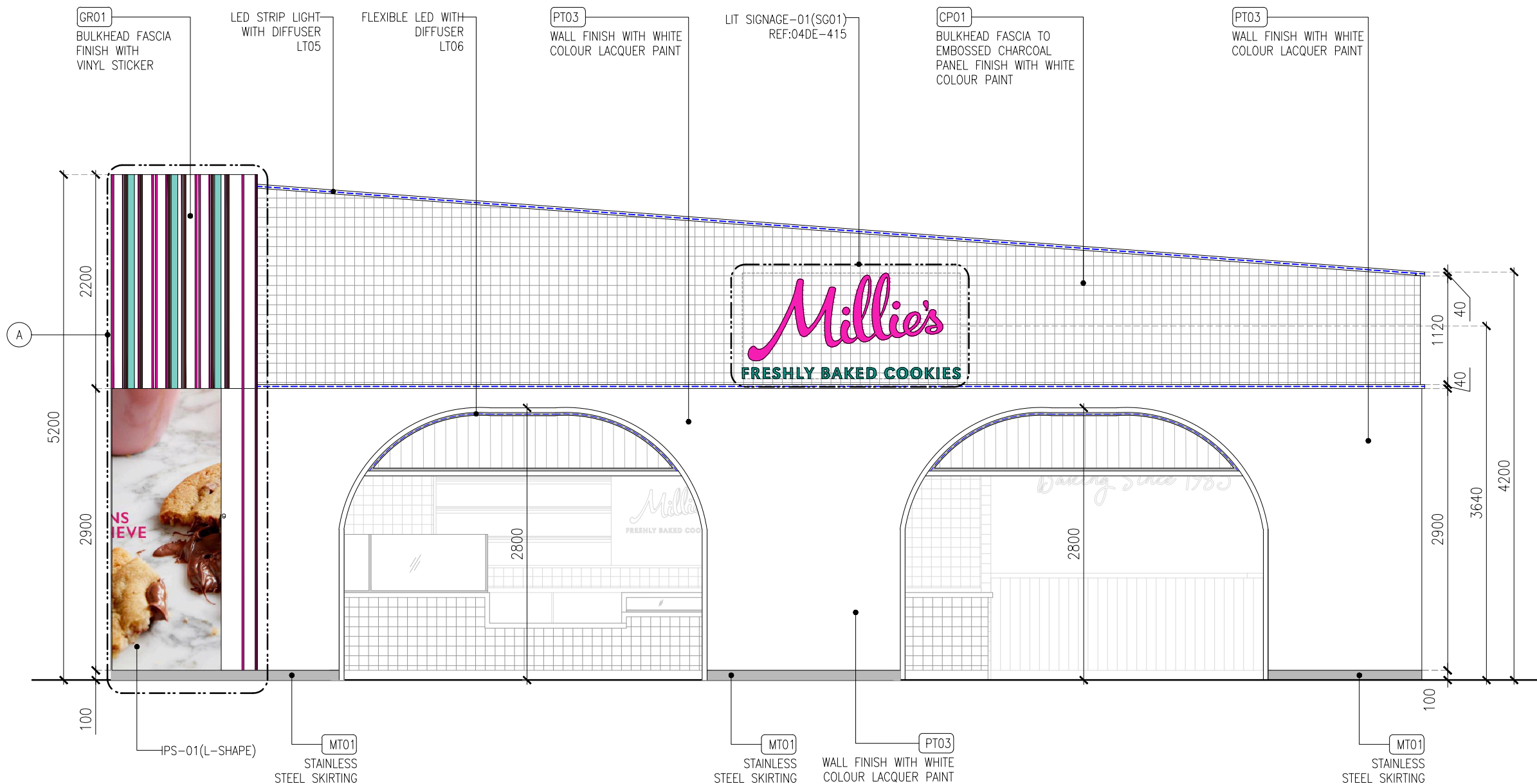
01 ELEVATION-02 03IL-301 1:50
