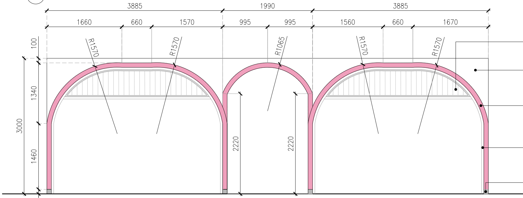
02 FACADE FRAMING (ELEVATION-03) 04DE-414 1:50
