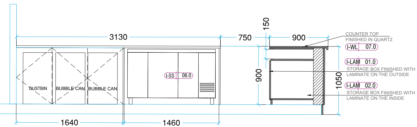
Section B
