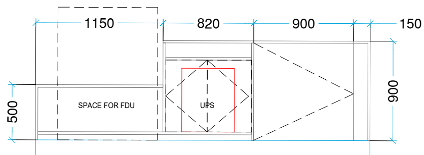
Section C
