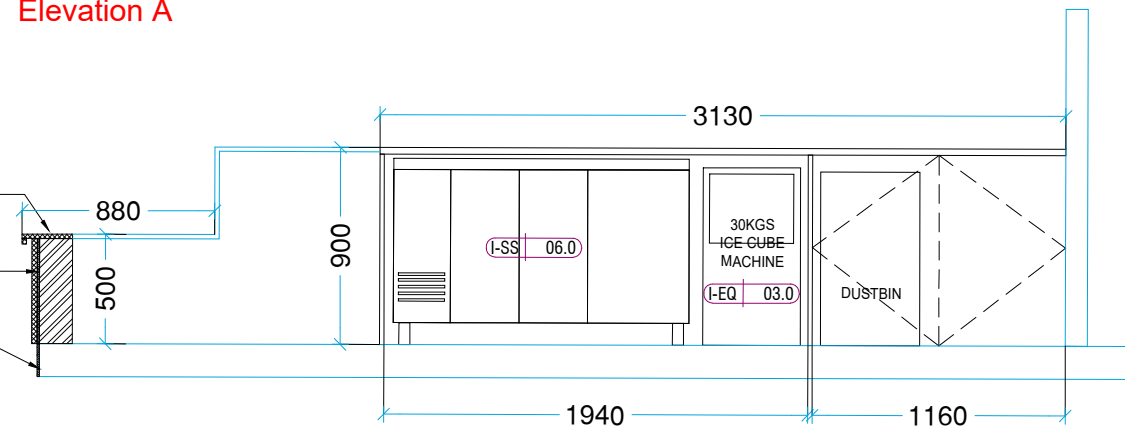
Section A
