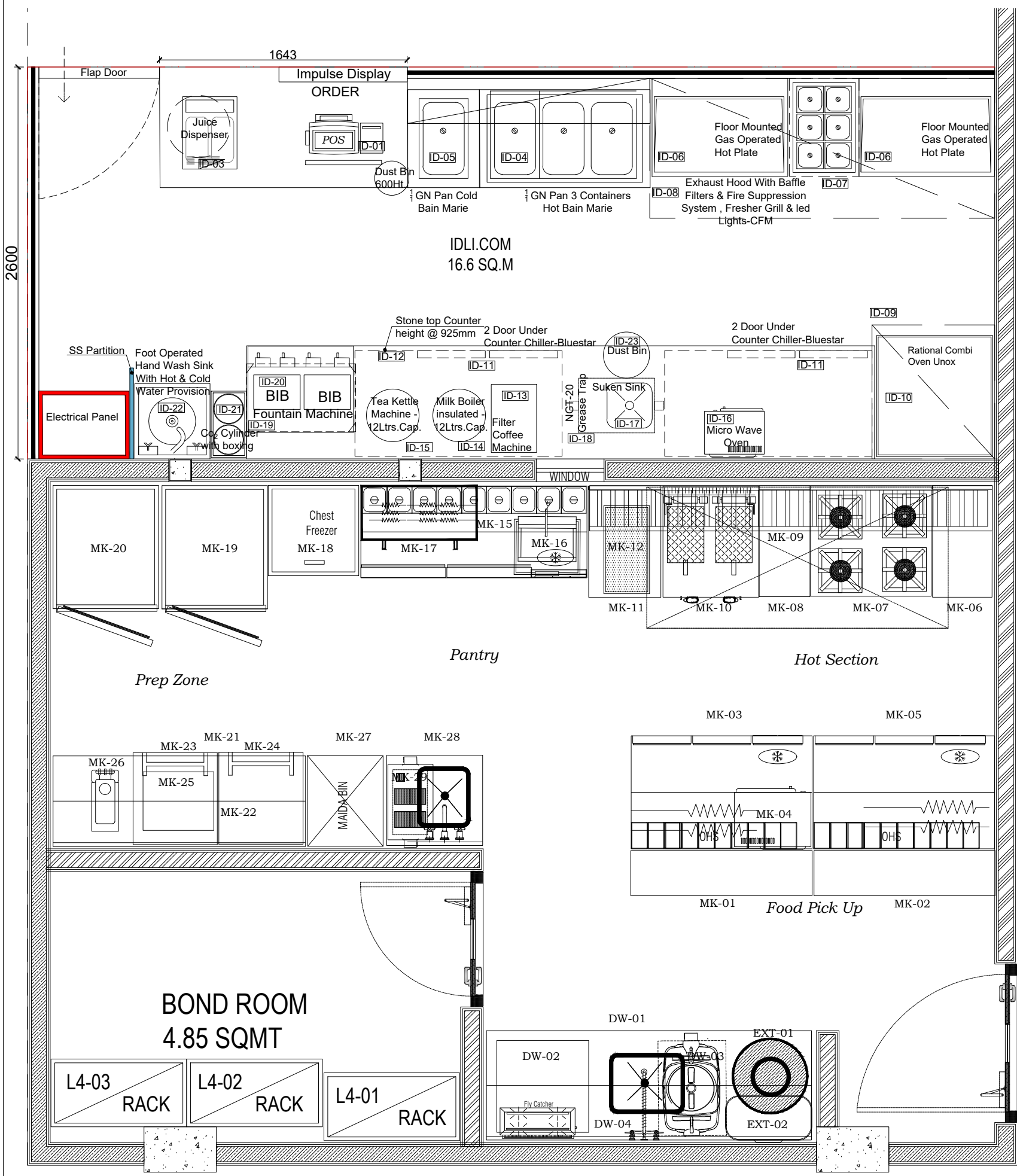
1 GENERAL ARRANGEMENT PLAN Scale:- 1:20
