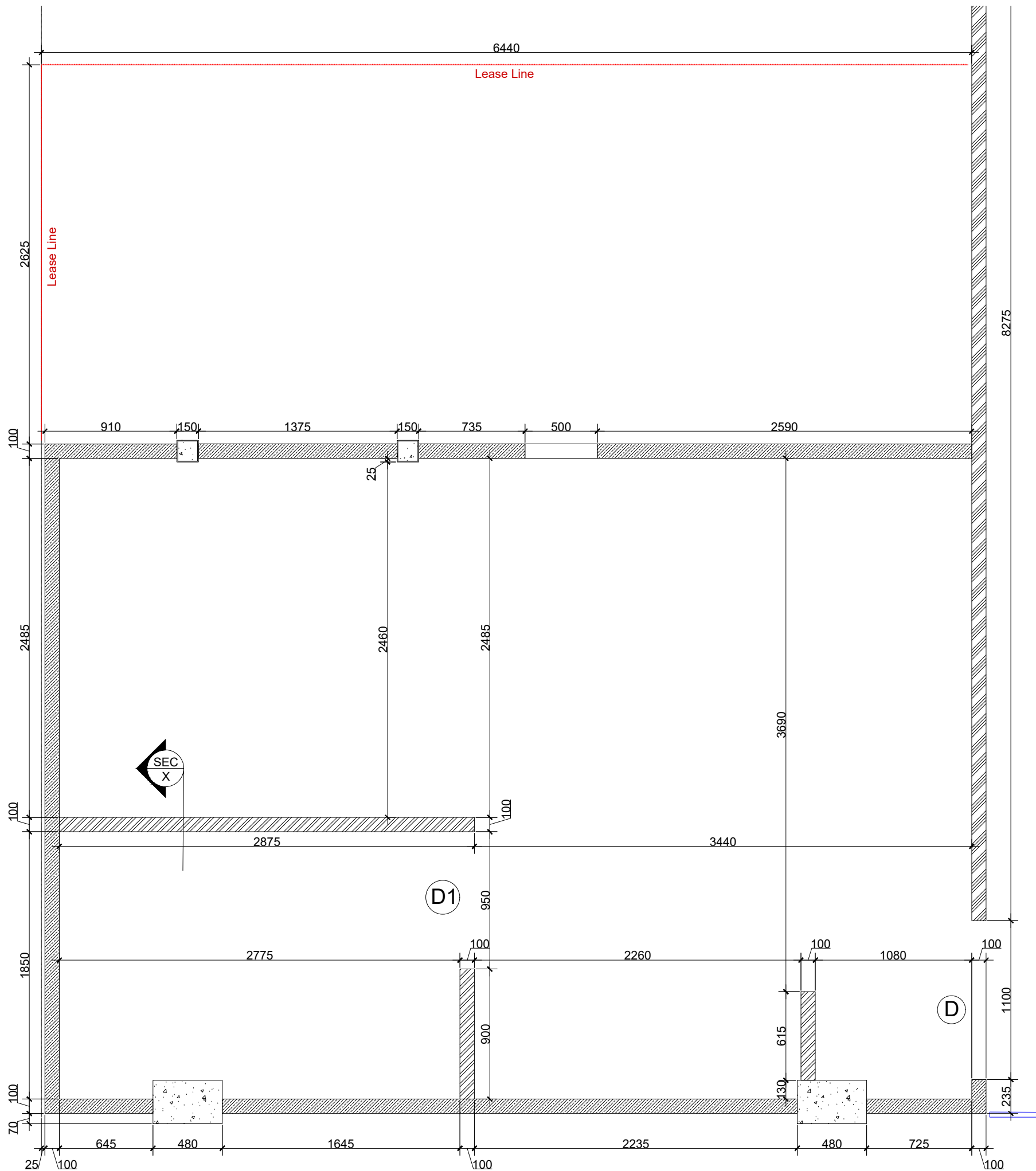
1 CIVIL LAYOUT & WORKING
